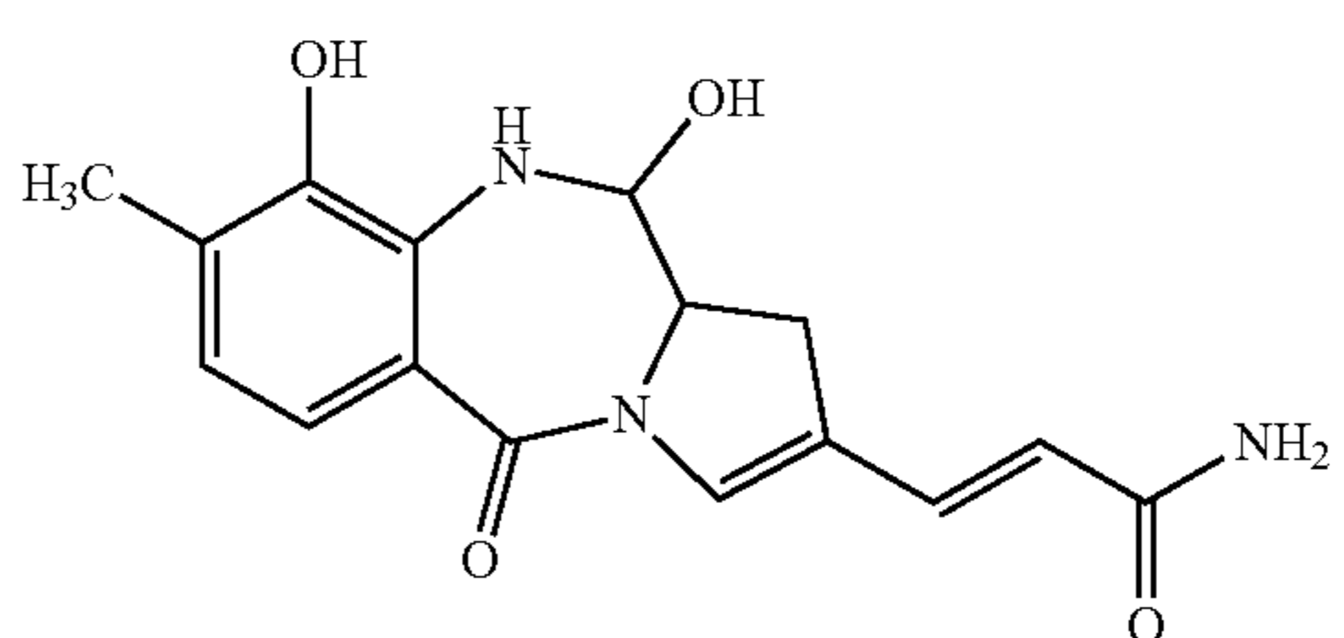
Anthramycin
