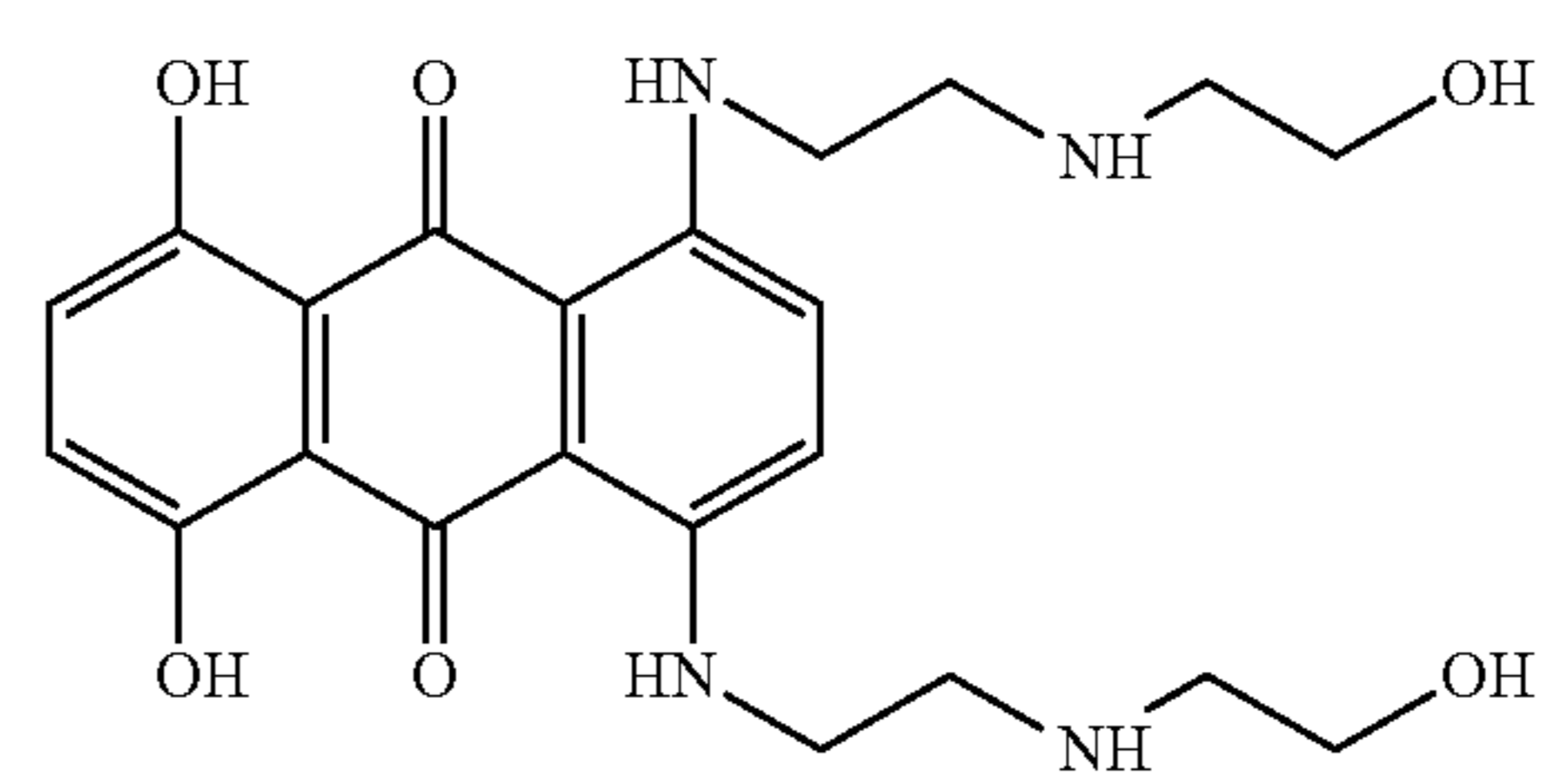
Mitoxantrone
