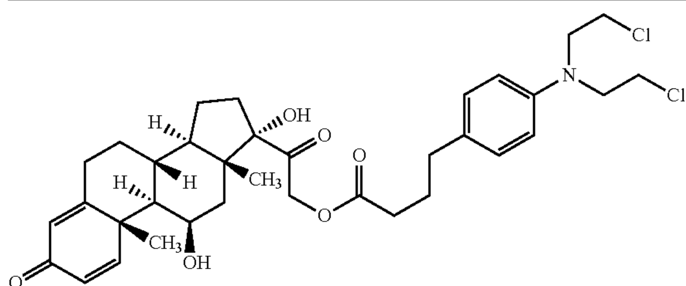
(XXXV) Prednimustine
