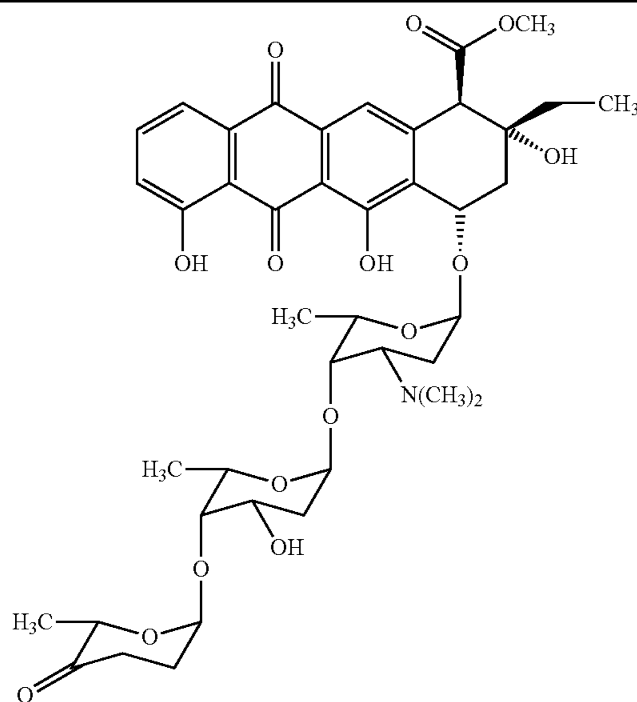
Aclacinomycin A
