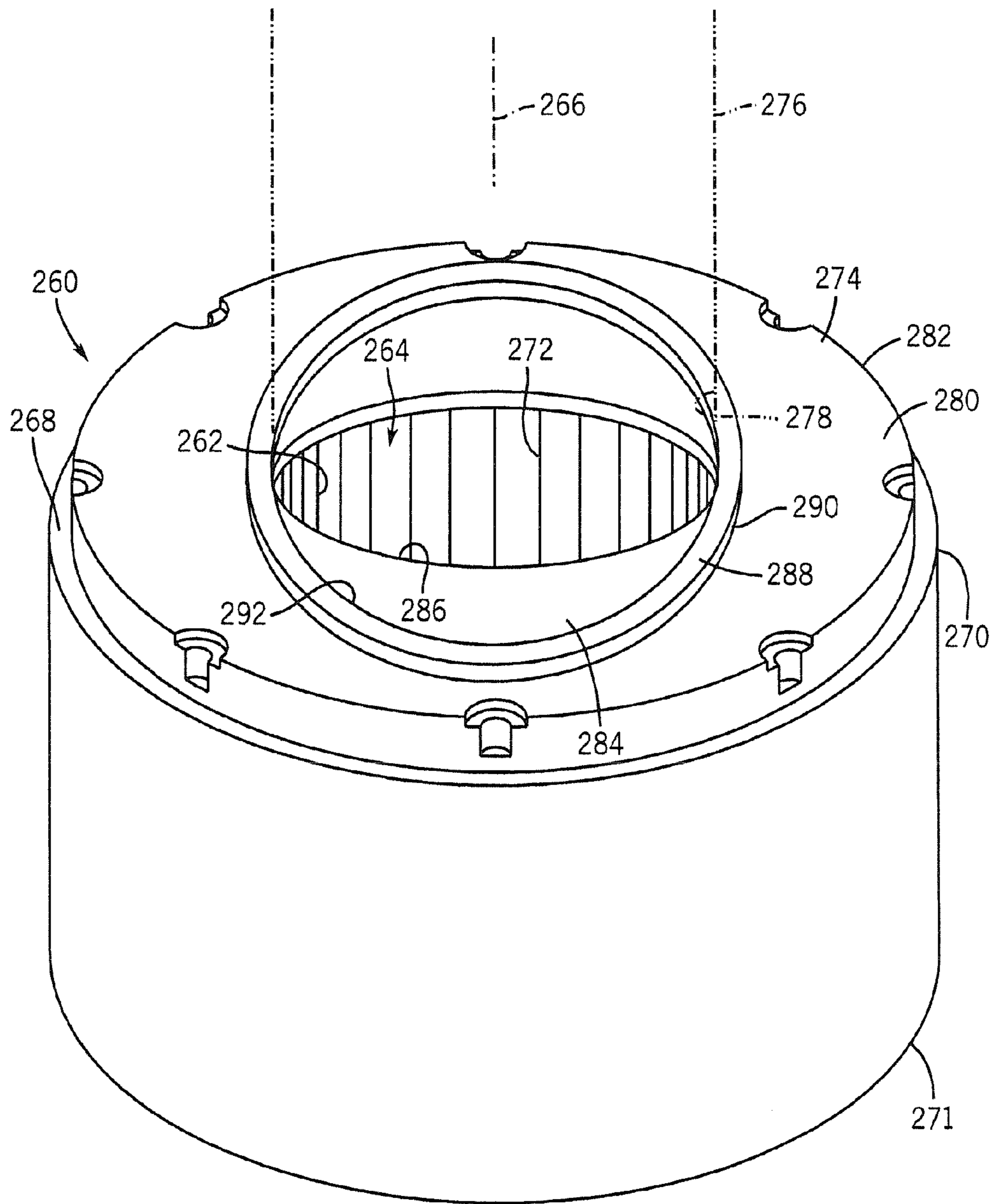
FIG. 14 PRIOR ART
