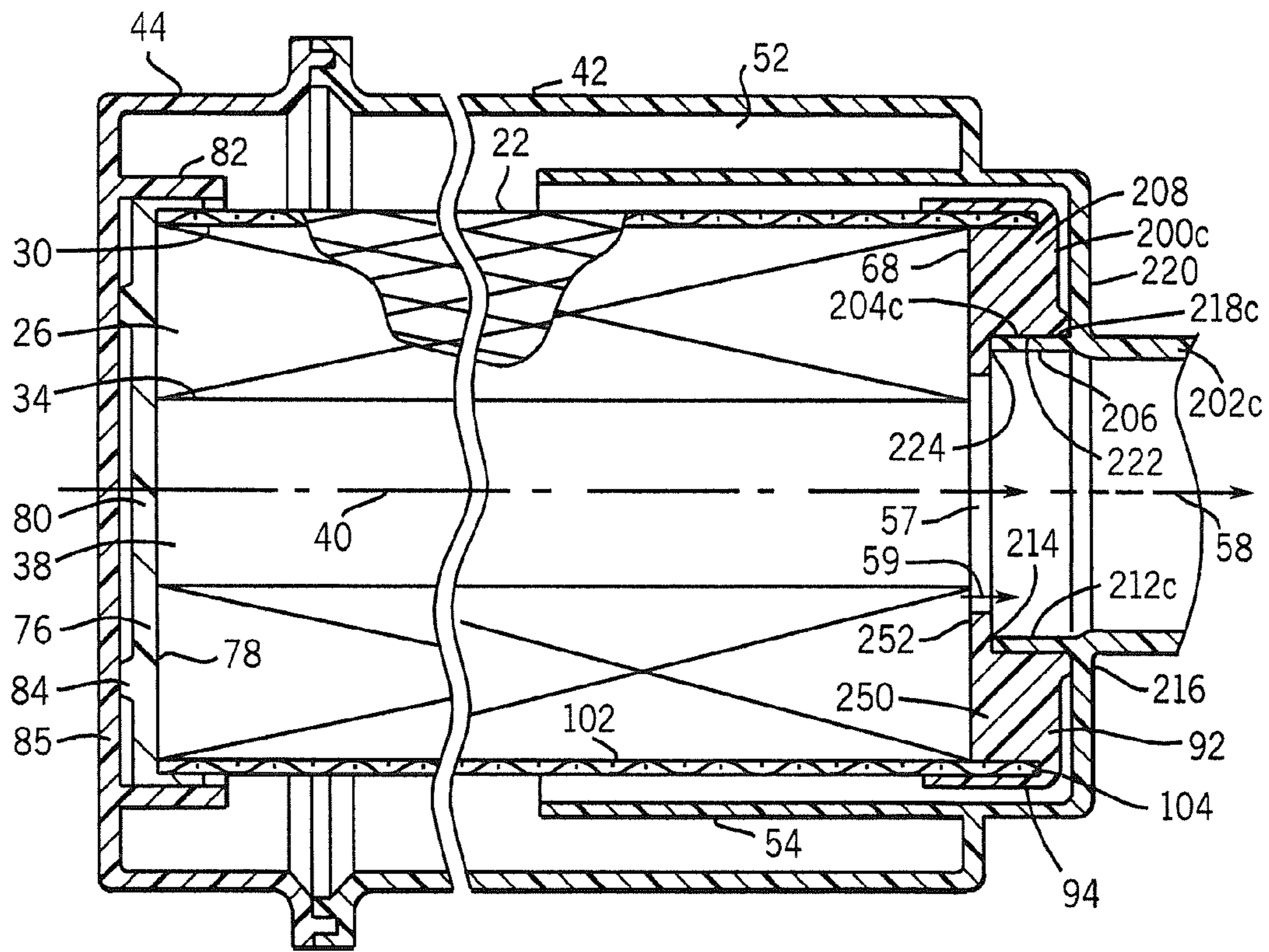
FIG. 13 PRIOR ART
