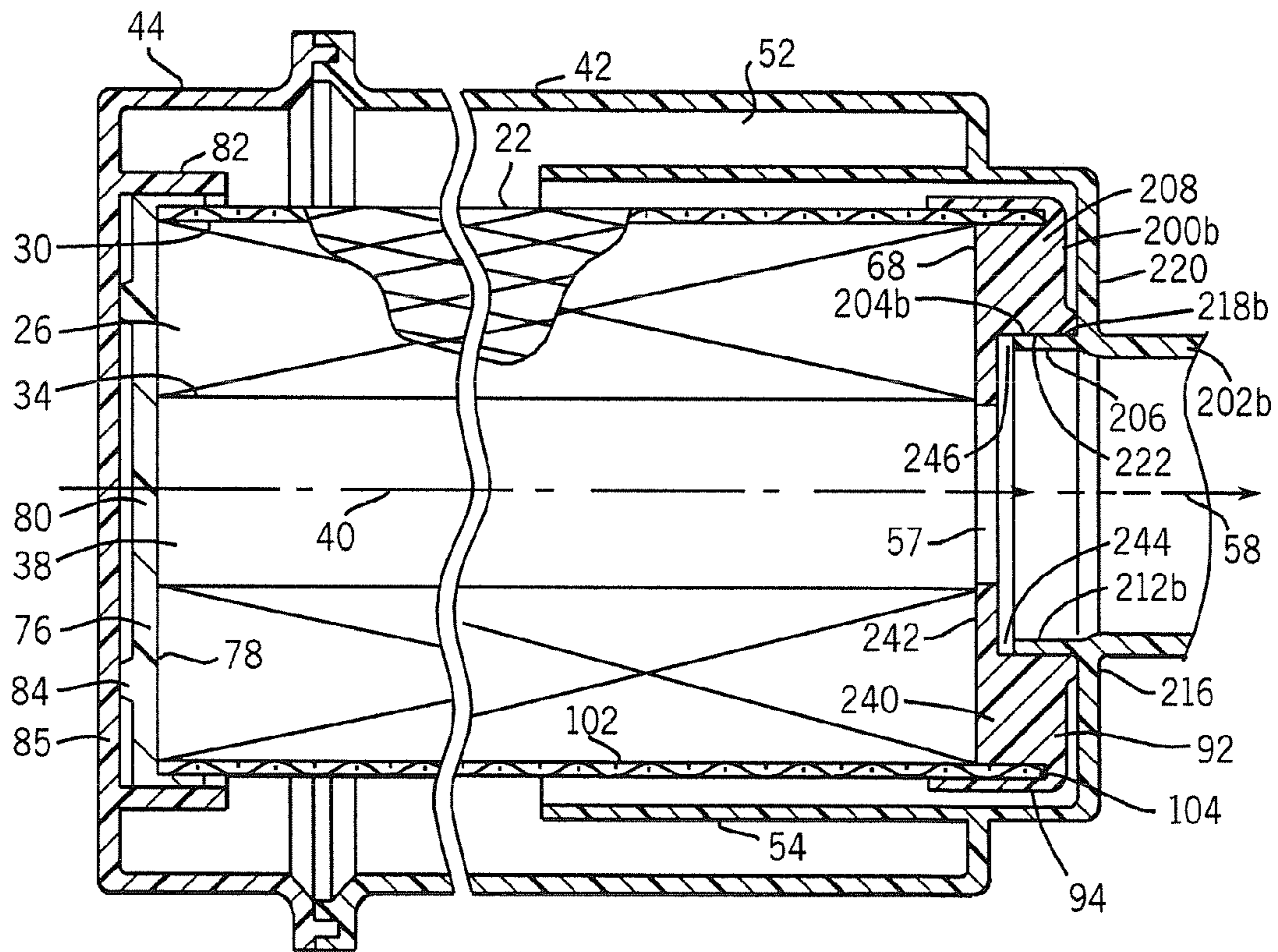
FIG. 12 PRIOR ART
