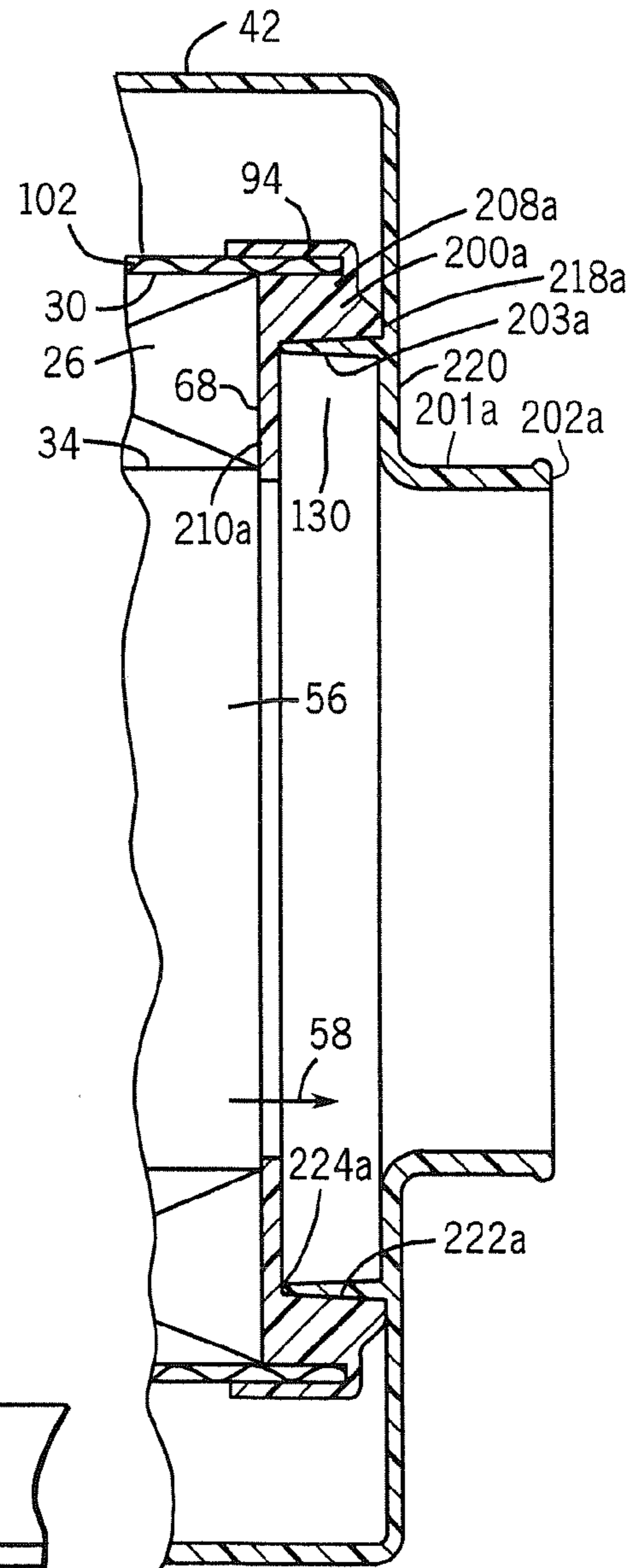
FIG. 11 PRIOR ART
