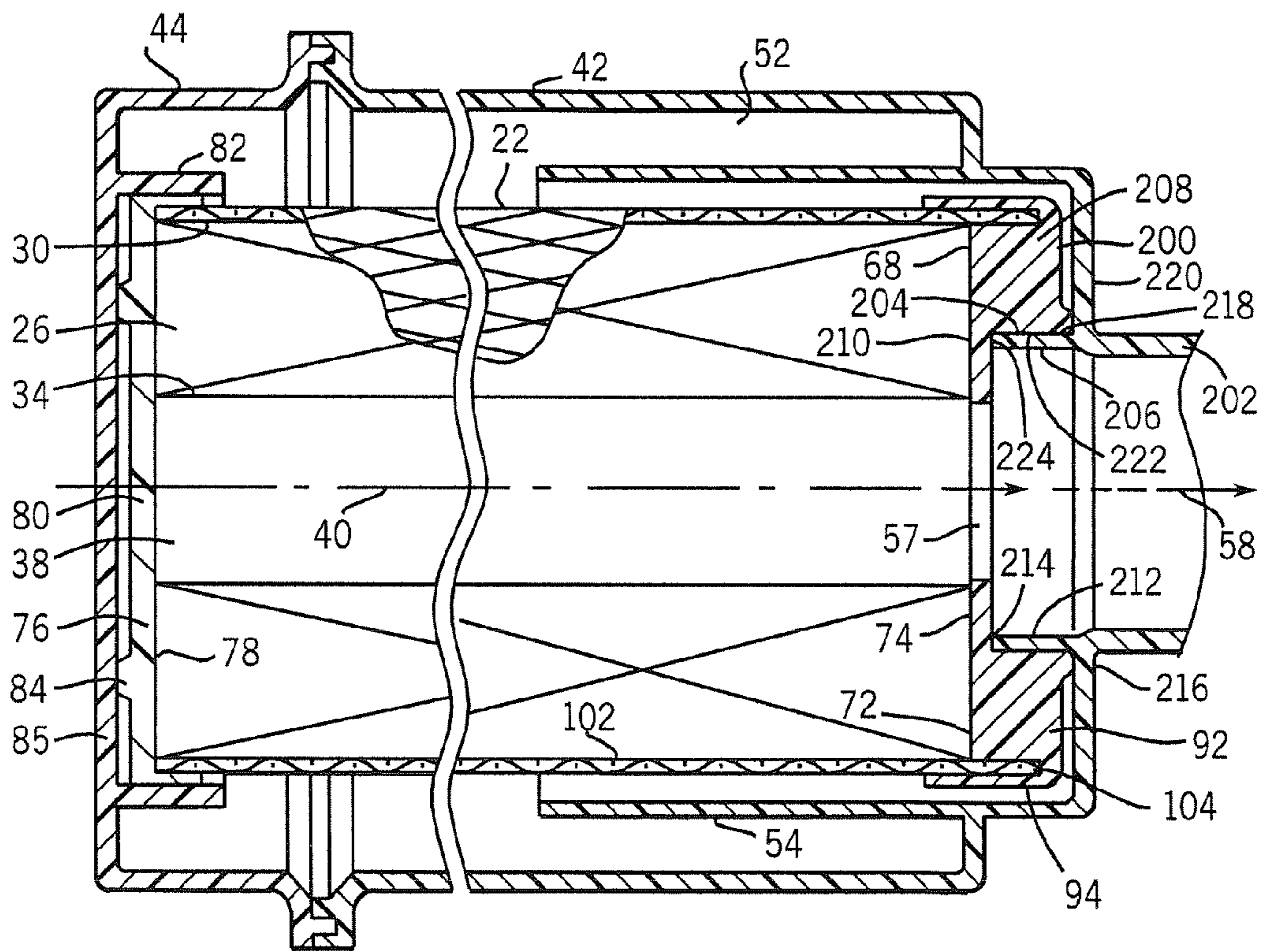
FIG. 7 PRIOR ART
