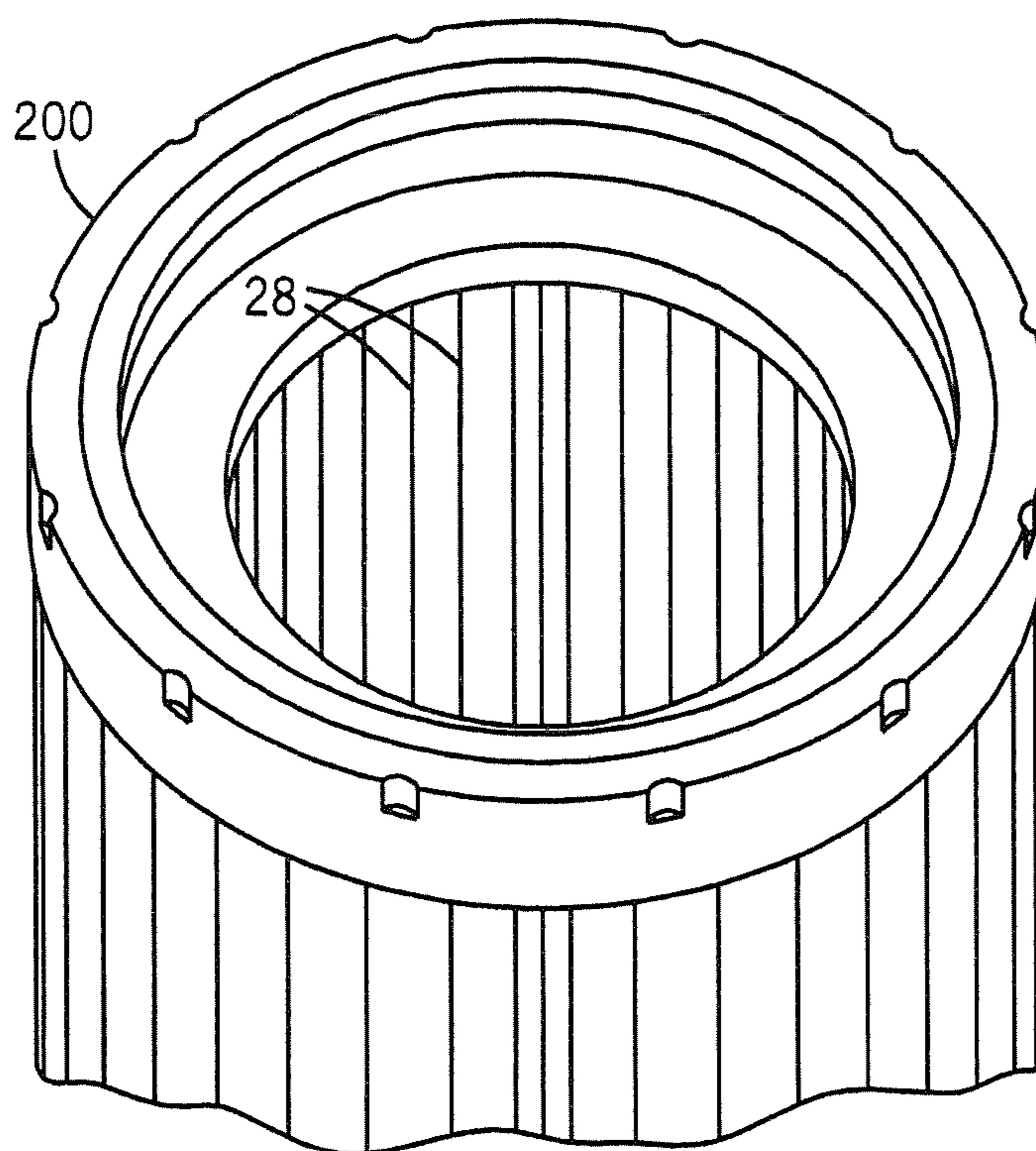
FIG. 9 PRIOR ART
