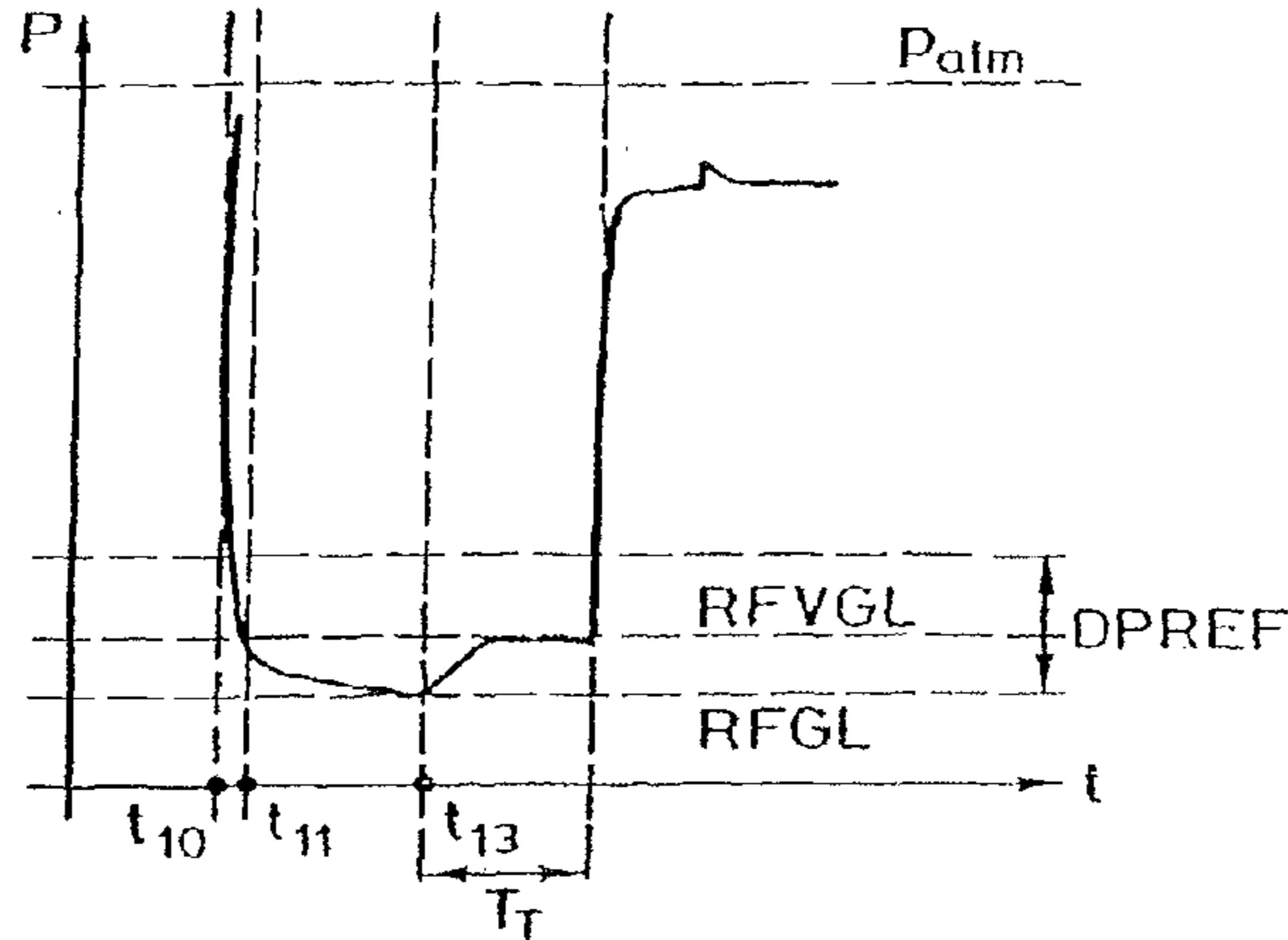
EVAC TEST VENT FIG.11c
