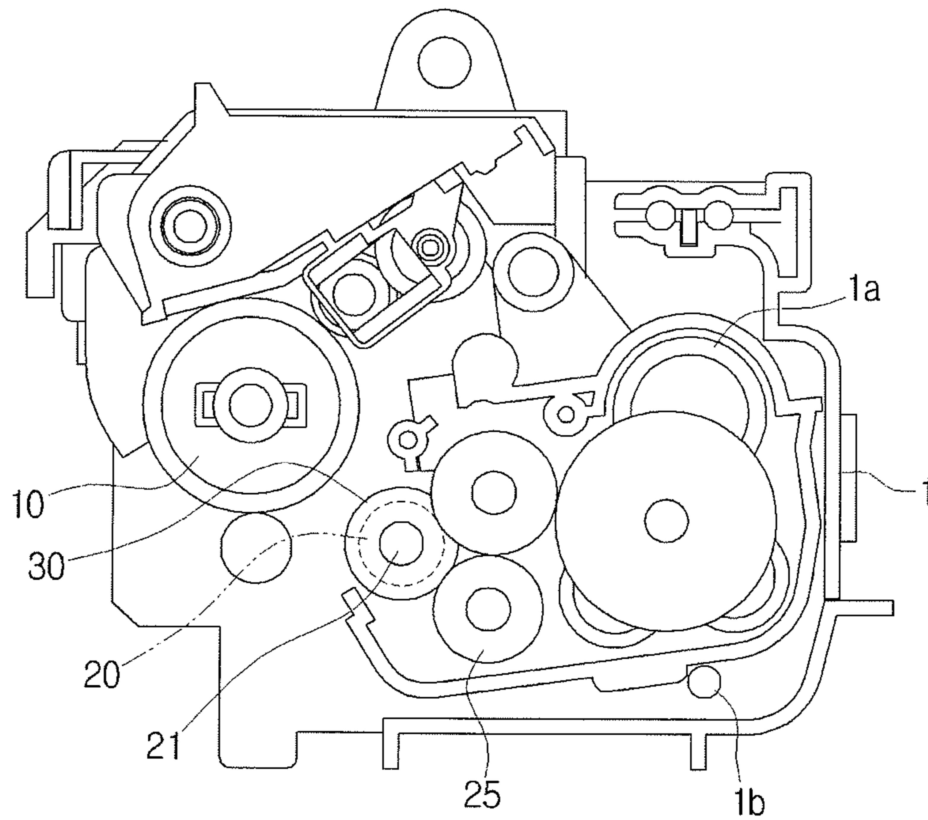
FIG. 2 (PRIOR ART)
