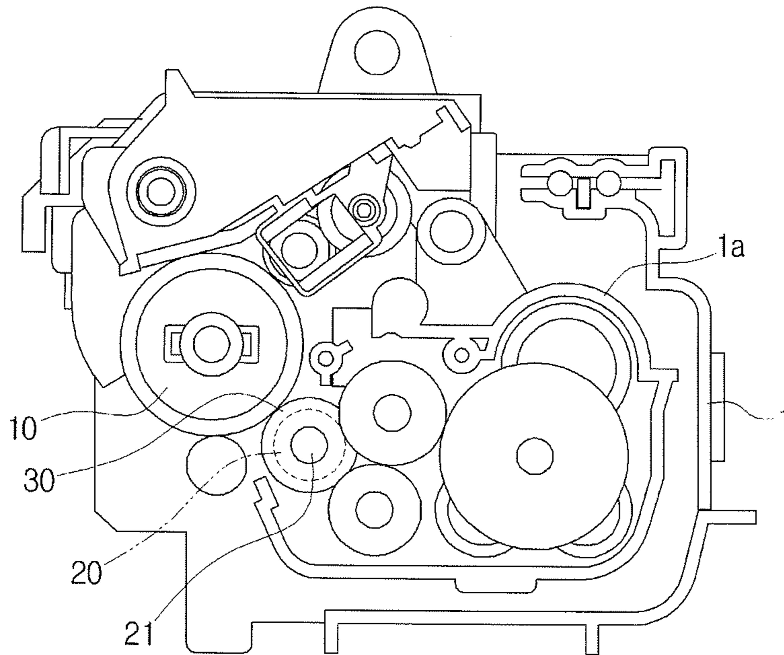
FIG. 1 (PRIOR ART)
