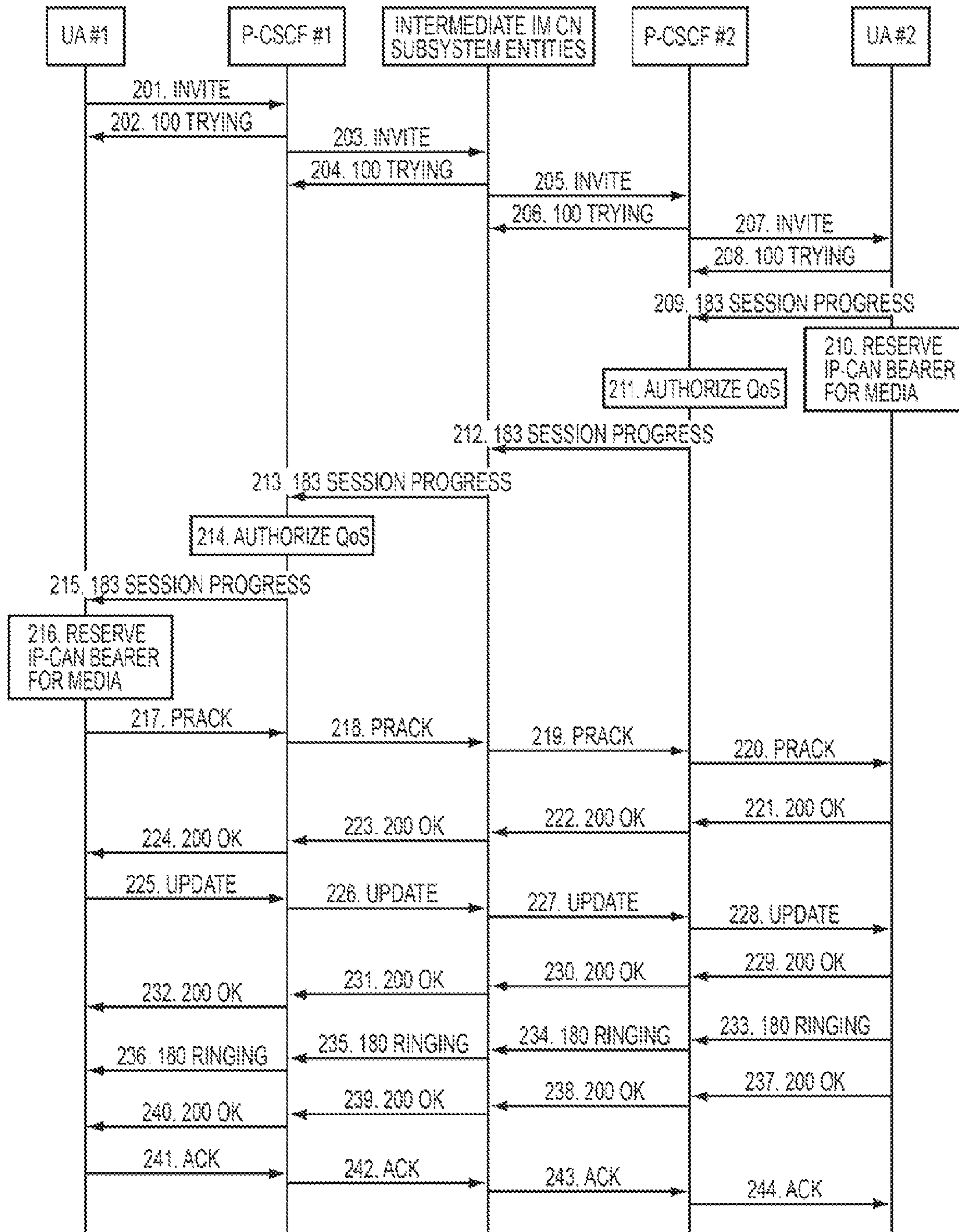
FIG. 2 (PRIOR ART)
