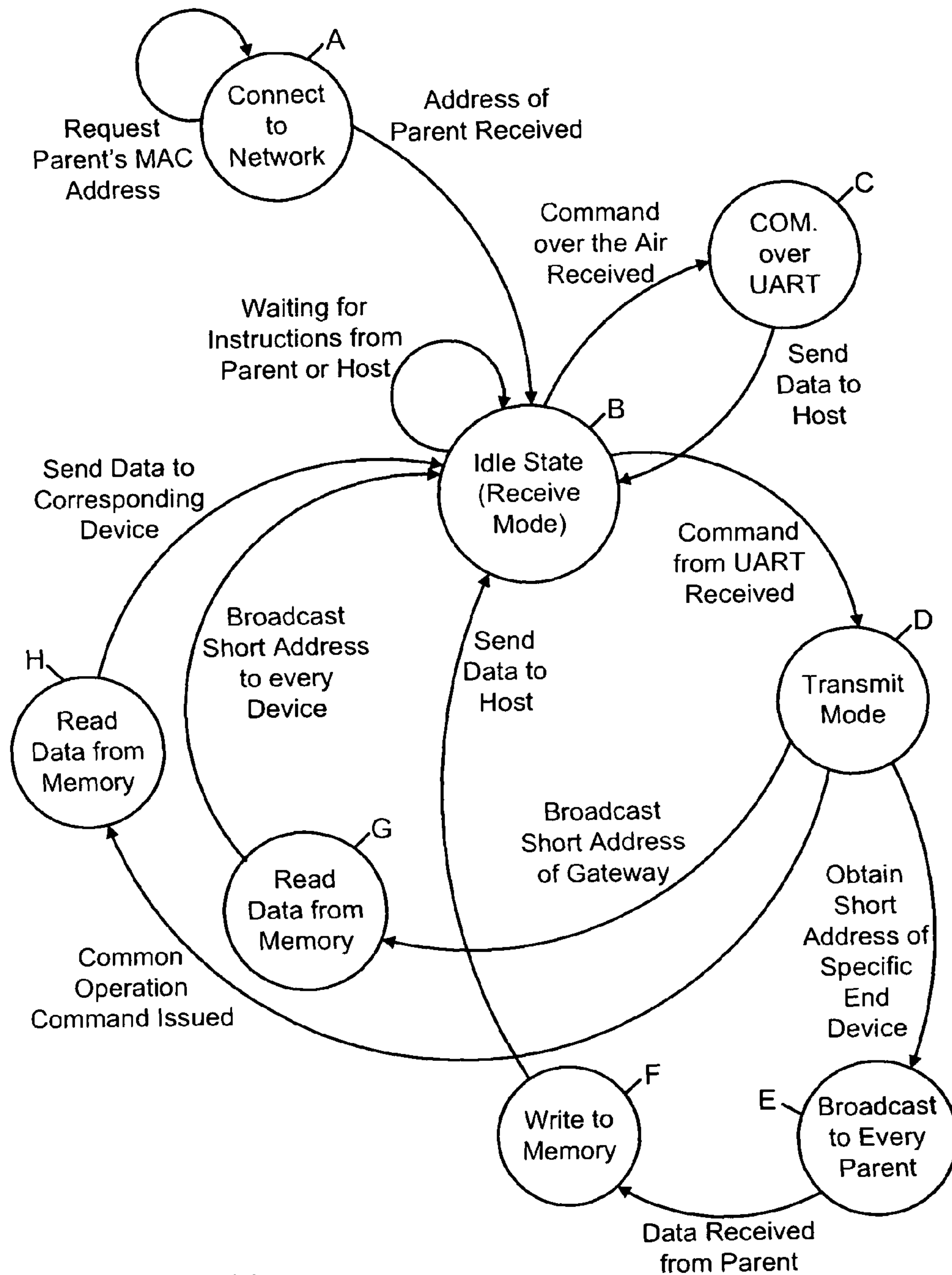
Gateway State Diagram
