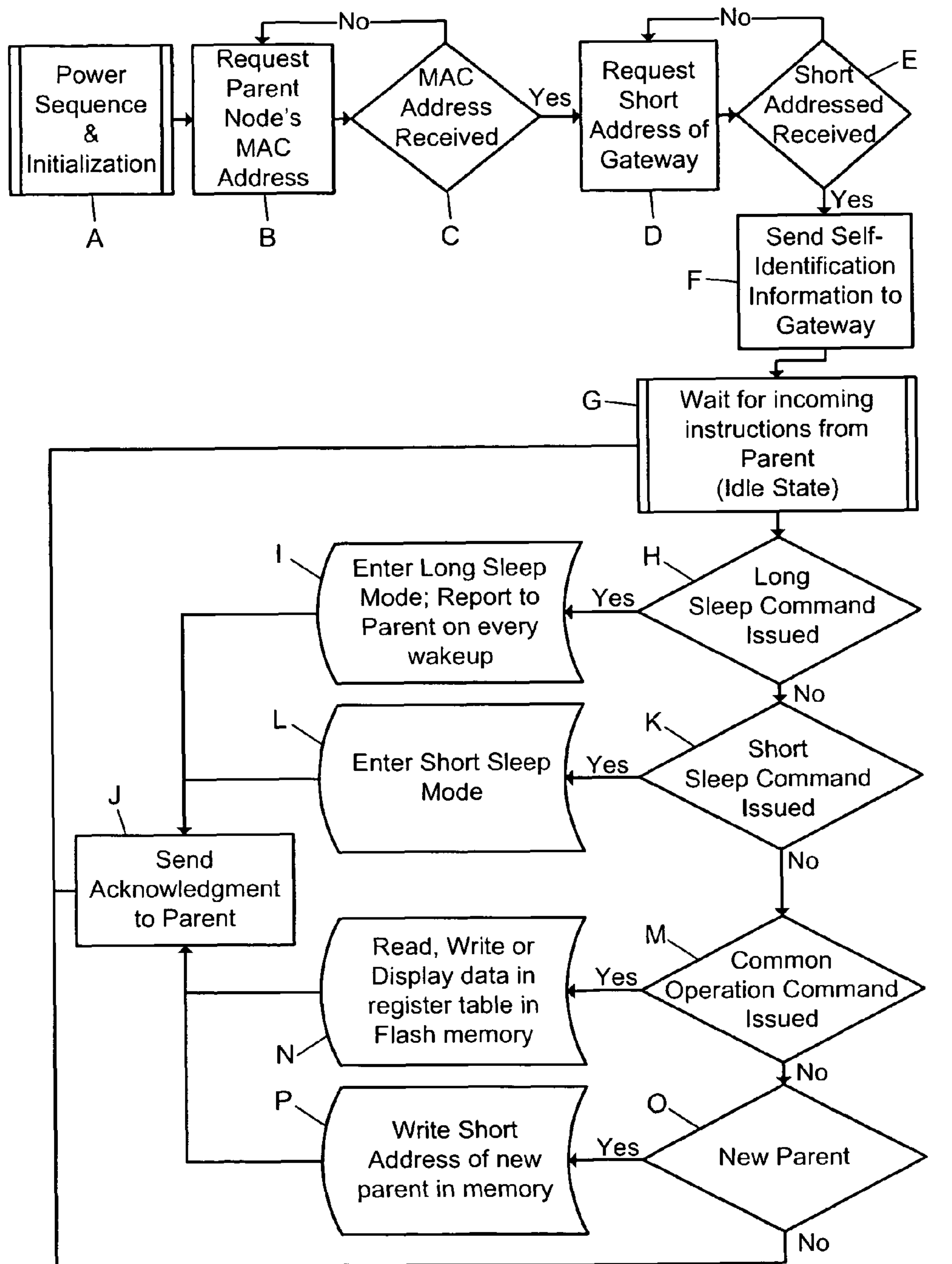
Network End-Device (E-Display) Firmware Flowchart
