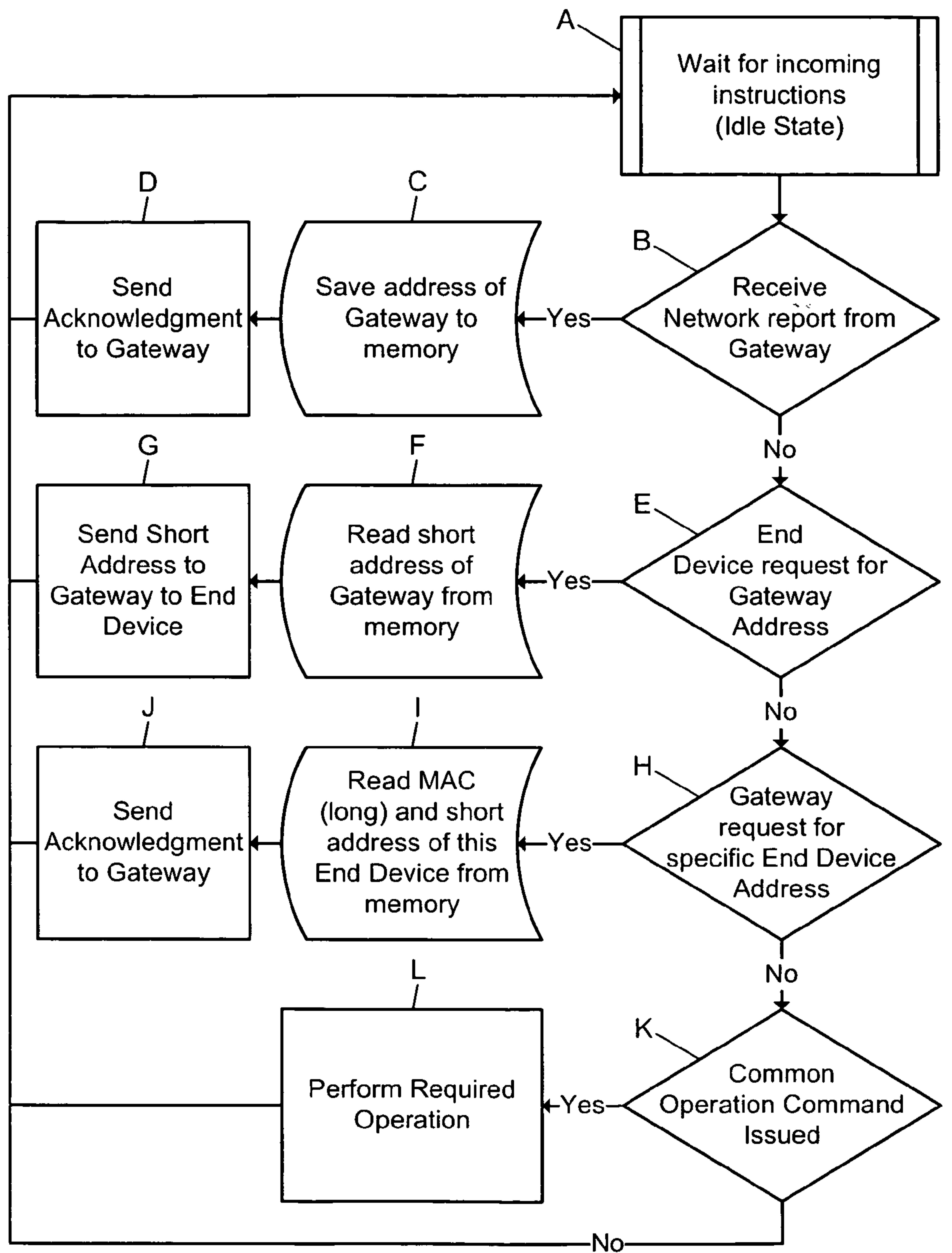
Network Coordinator Firmware Flowchart
