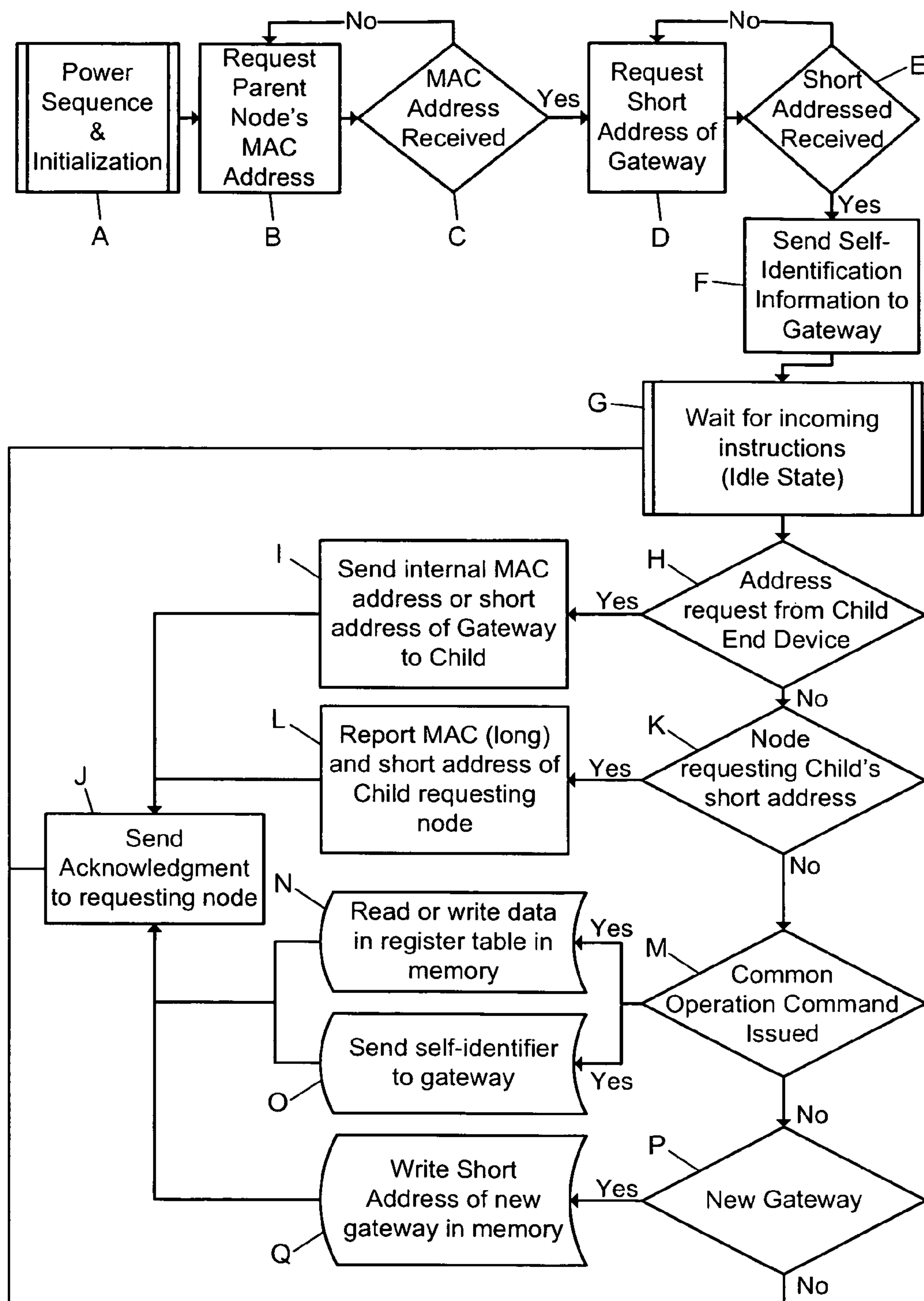
Zigbee Router Firmware Flowchart FIG. 8G
