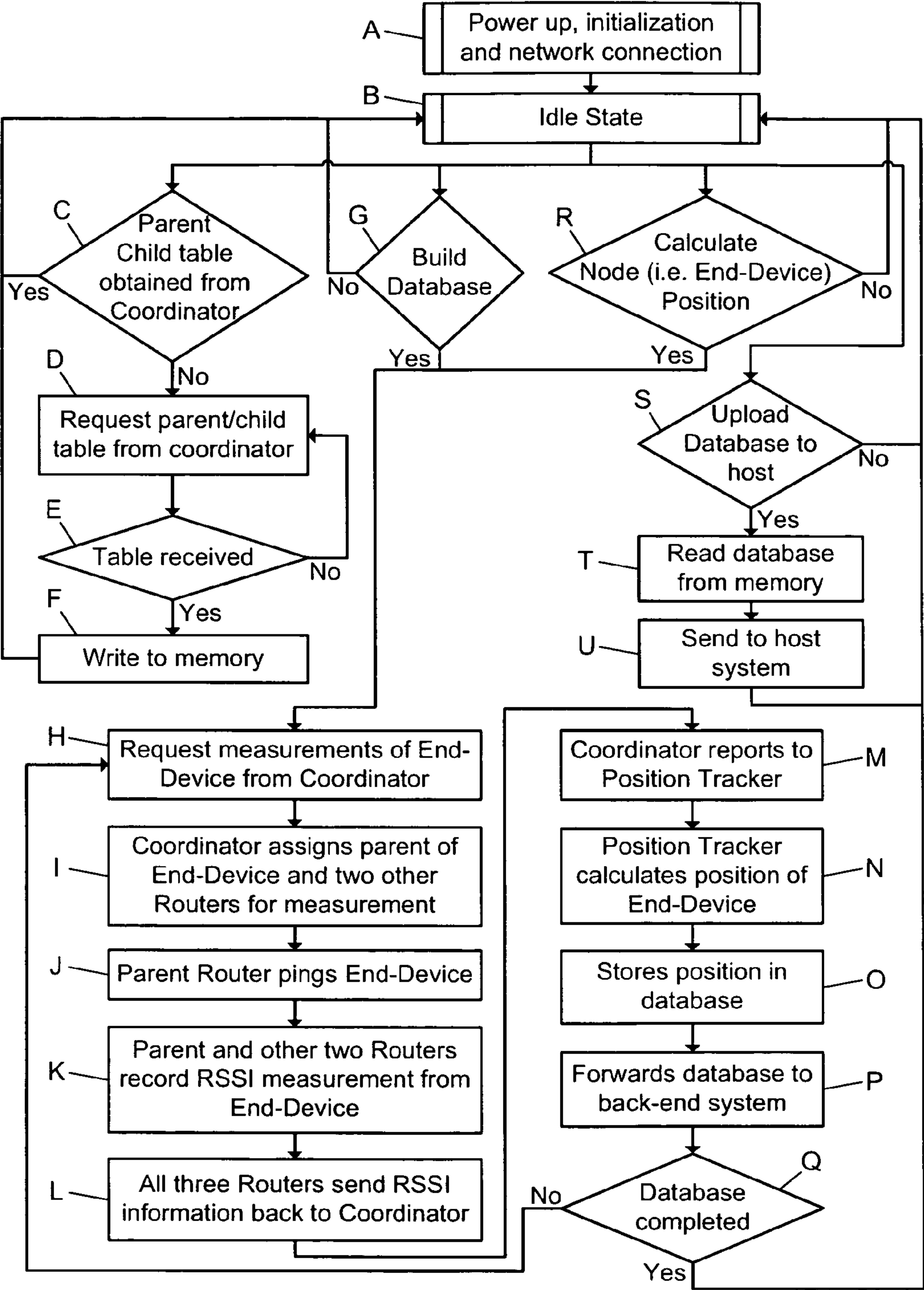
Position Tracking Module Flowchart
