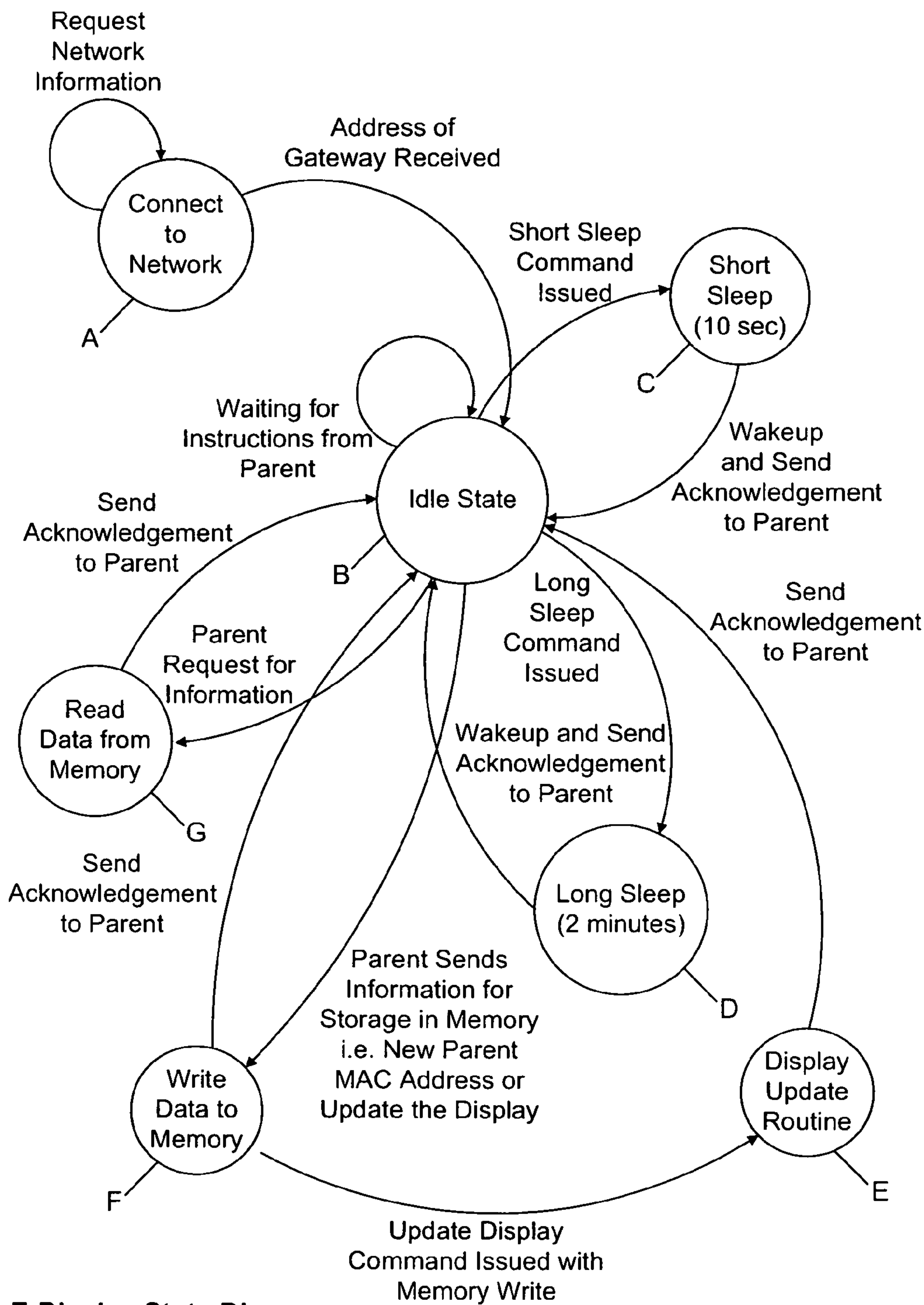
E-Display State Diagram
