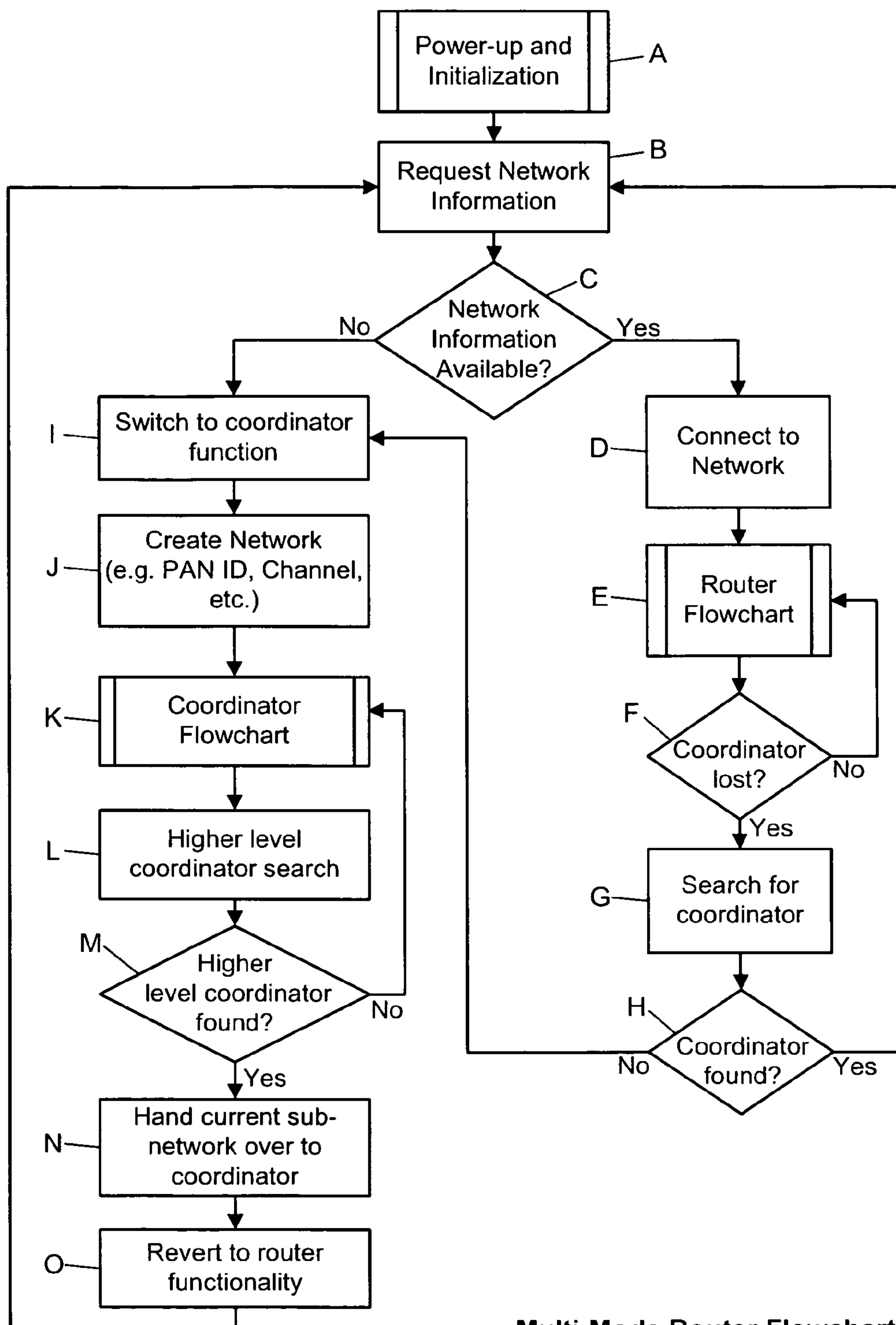
Multi-Mode Router Flowchart
