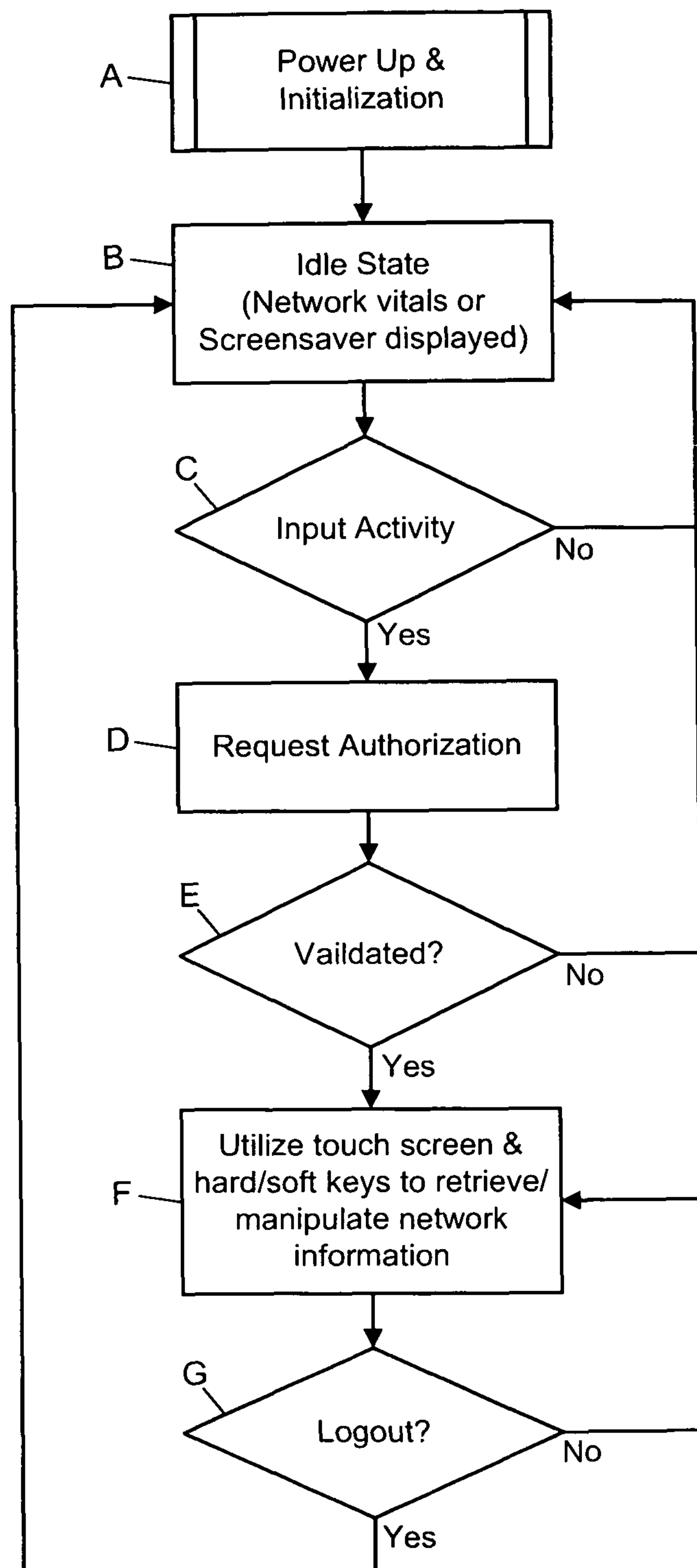
Network Monitoring Device Flowchart
