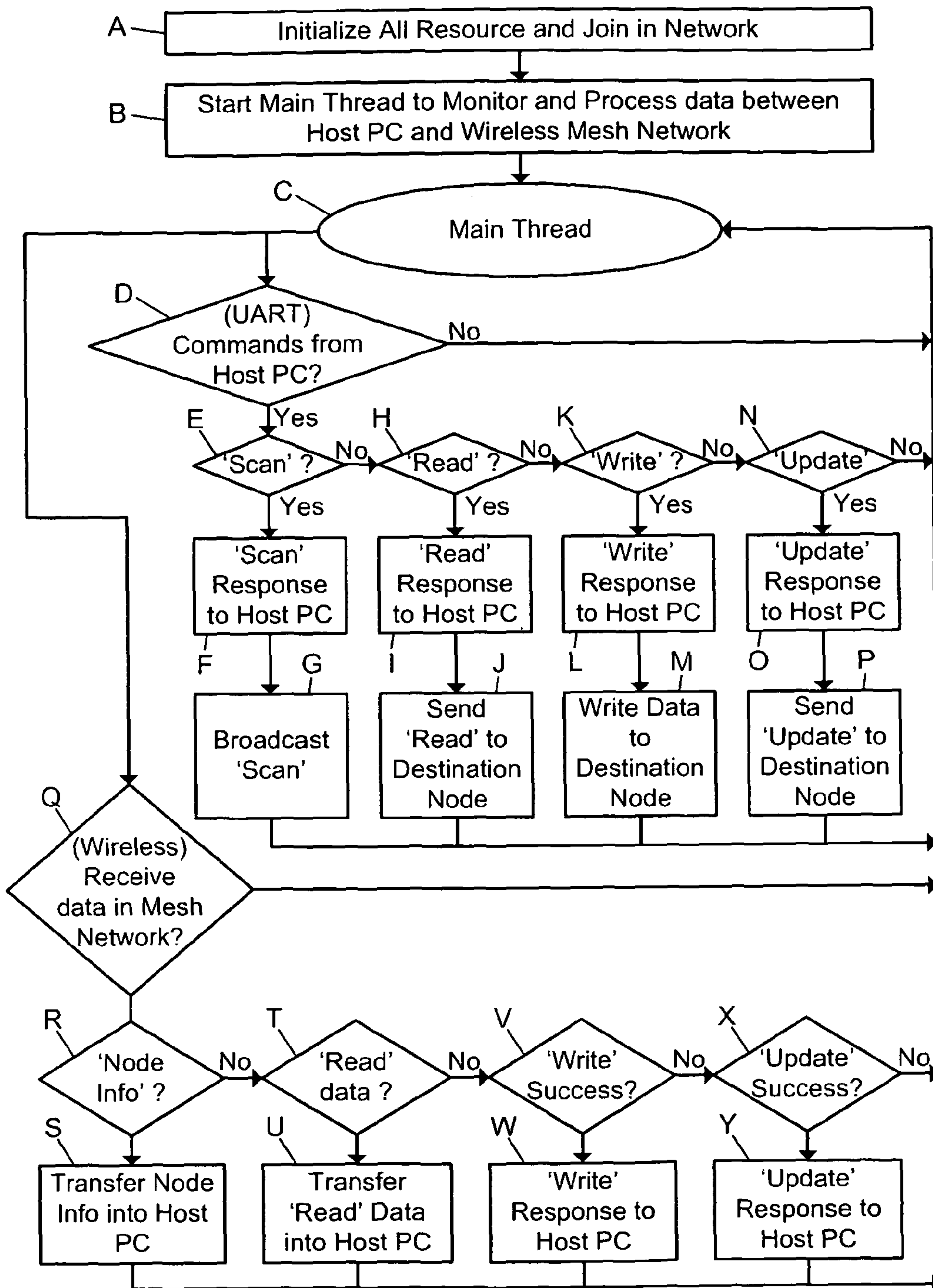
Gateway Firmware Flowchart
