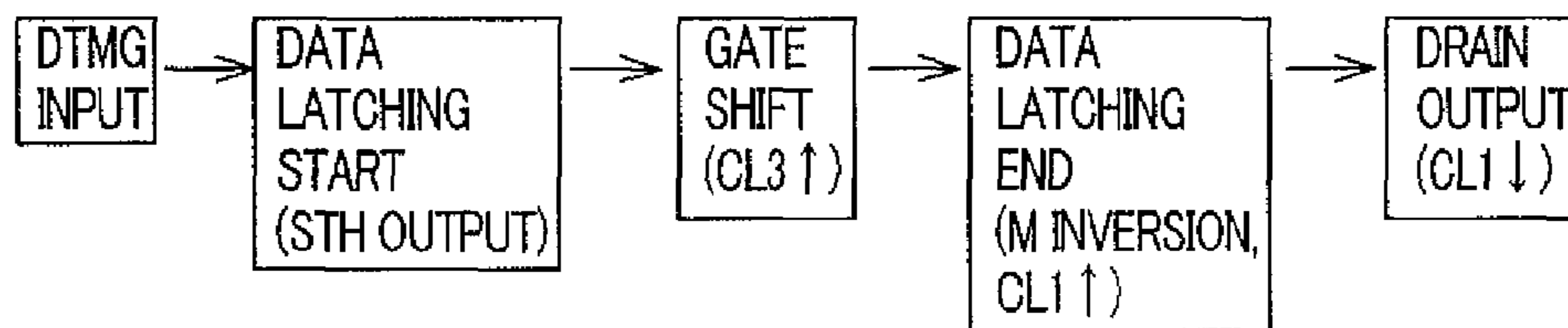
SEQUENCE OF THE LIQUID CRYSTAL DRIVER (EXAMPLE)
