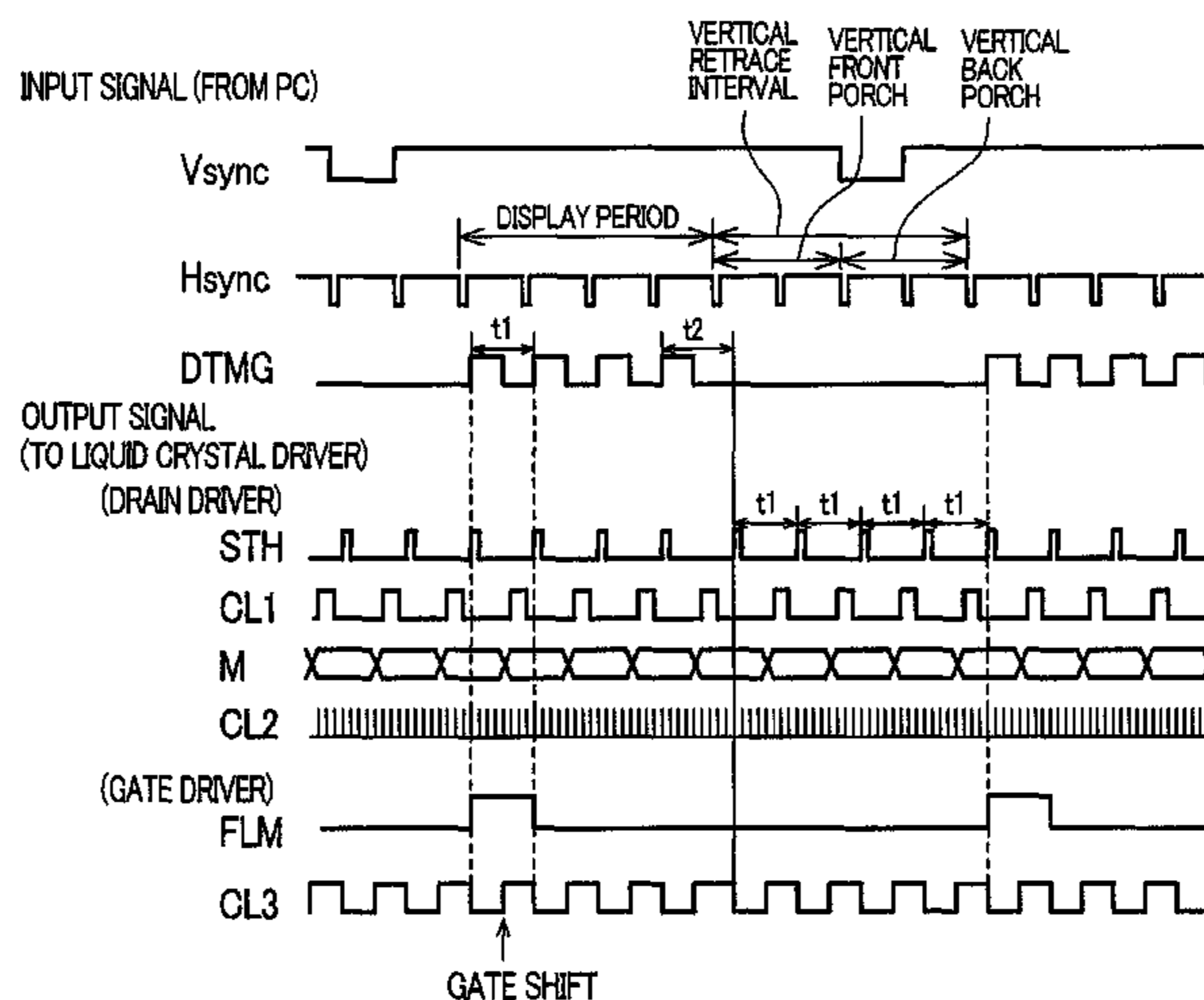
SEQUENCE OF THE LIQUID CRYSTAL DRIVER (EXAMPLE)
