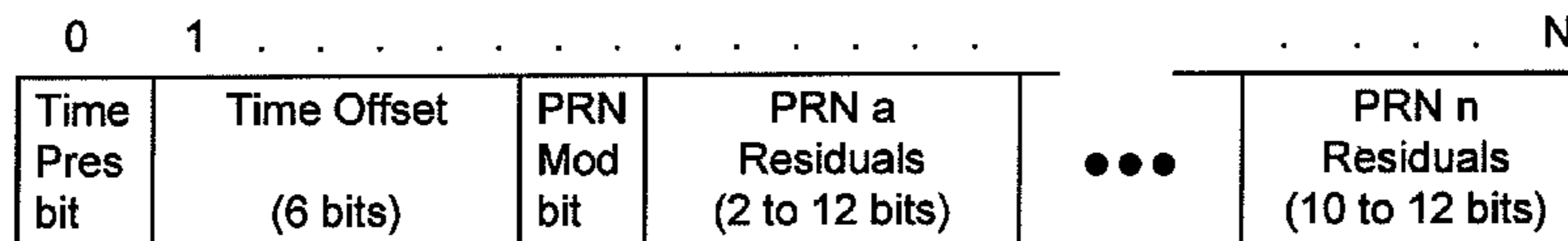
Figure 21. VRS Network Residuals Block
