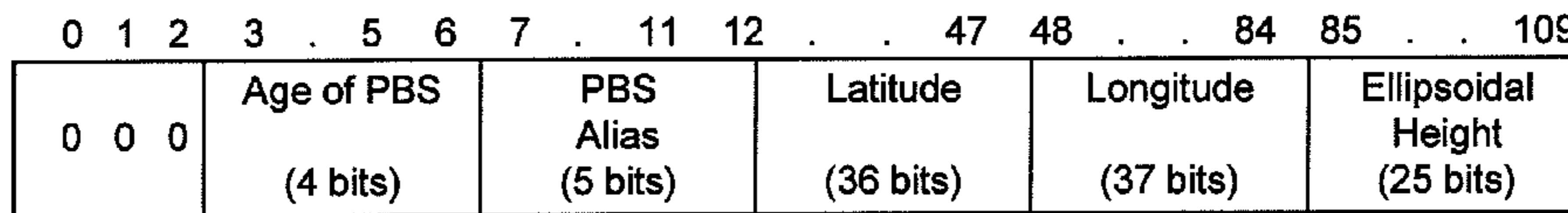
Figure 20. Full PBS Position per Message
