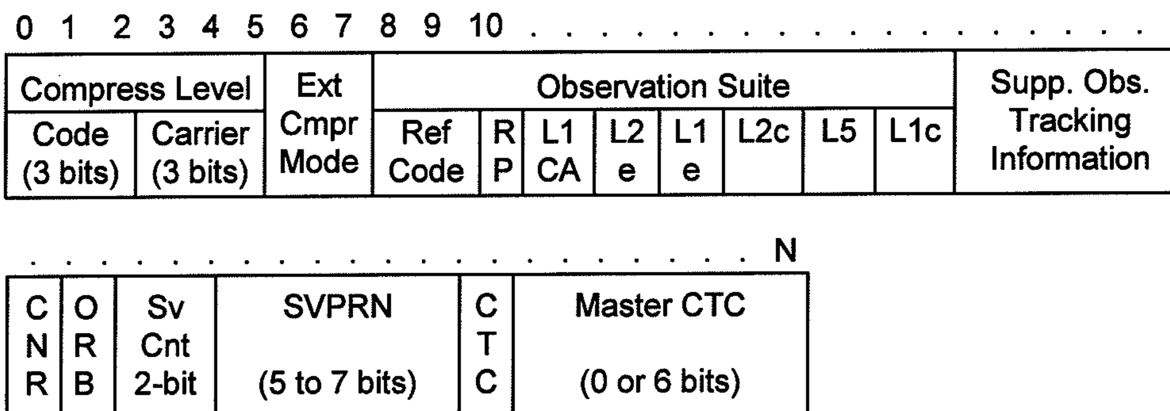
Figure 24. Observation Block Definition Bits
