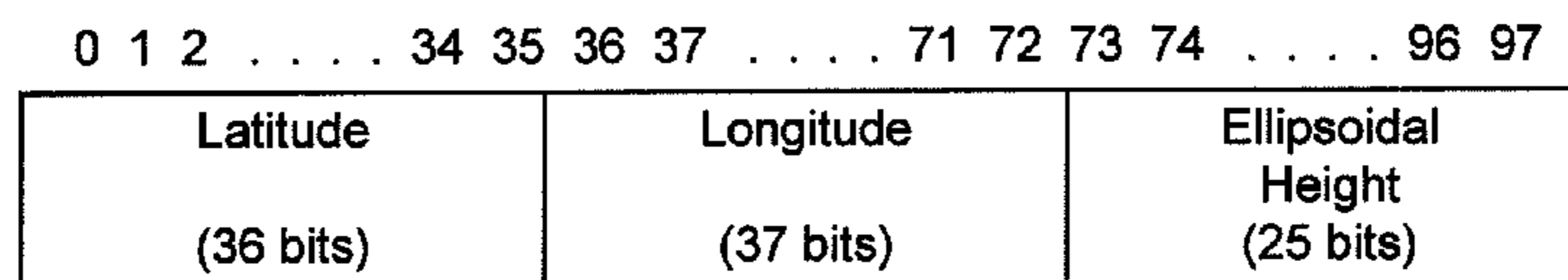
Figure 10. Unsegmented Position Construct
