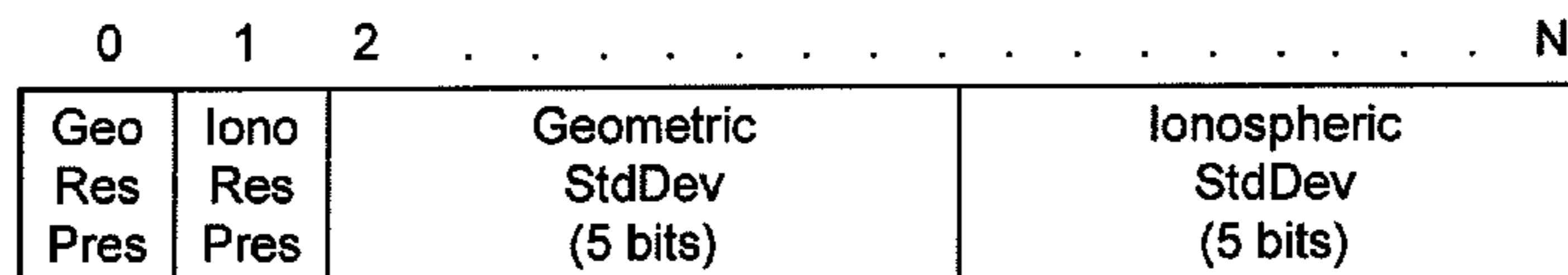
Figure 22. Per Satellite VRS Network Residuals
