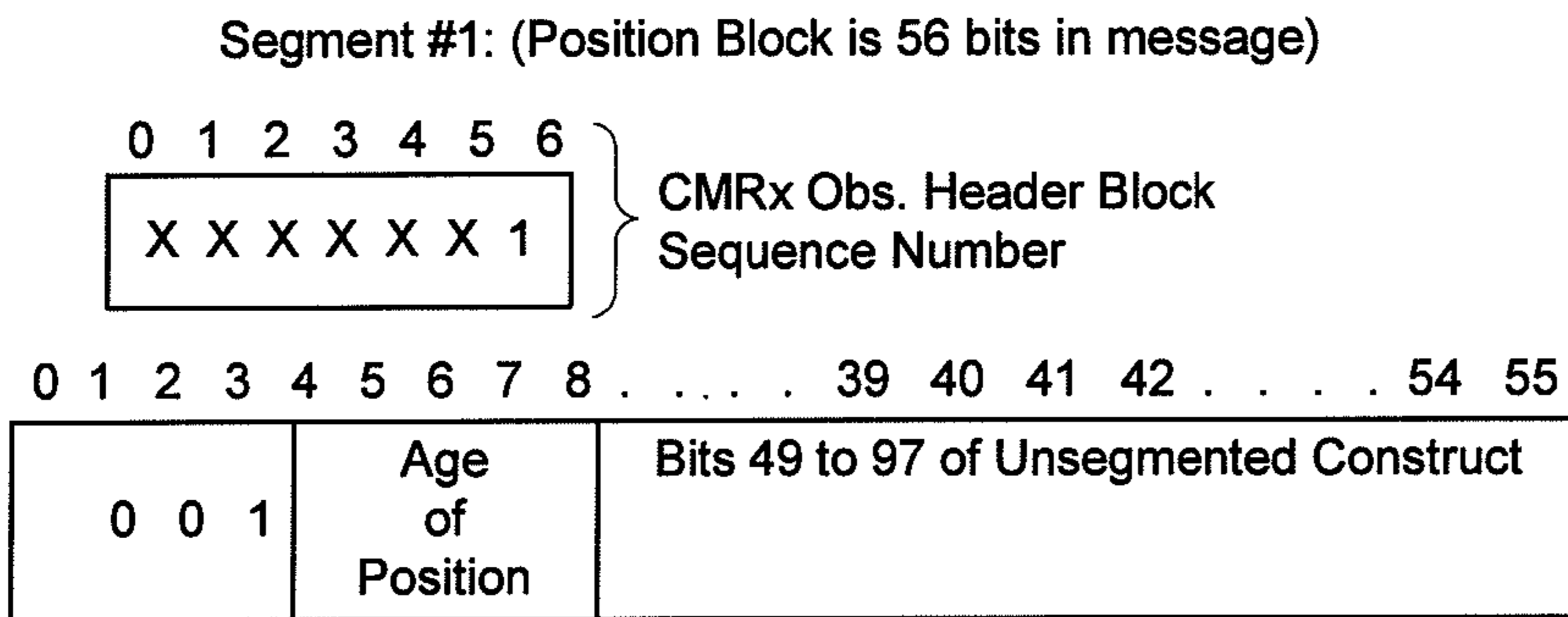
Figure 12. Position Message Sent Over 2 Epochs
