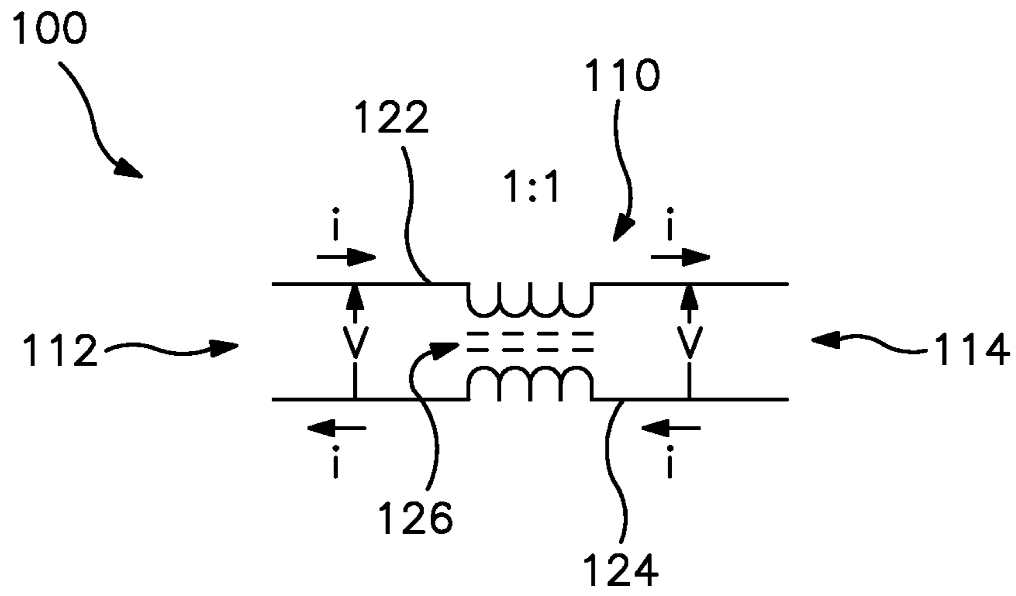
FIG. 1 PRIOR ART
