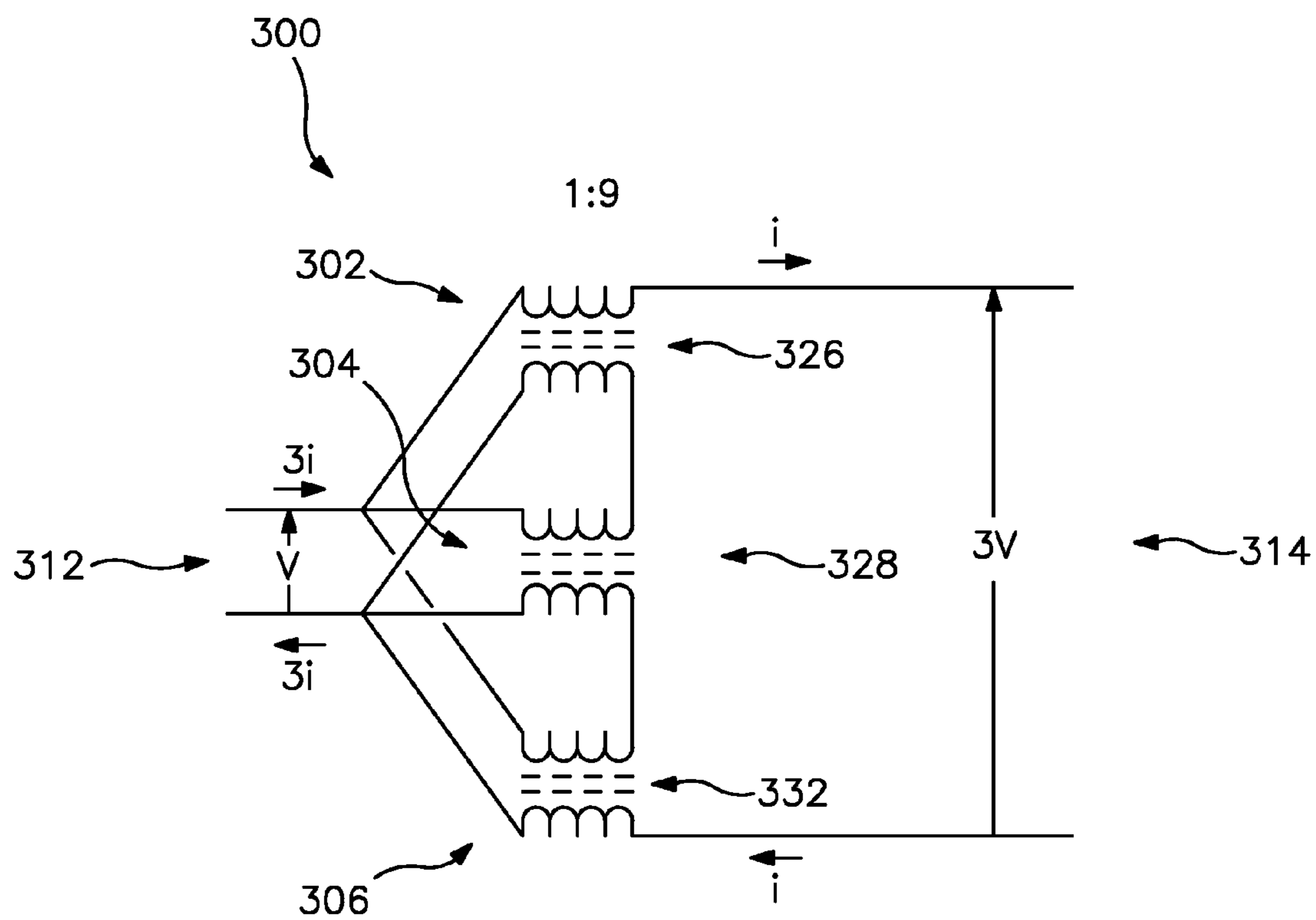
FIG. 3 PRIOR ART
