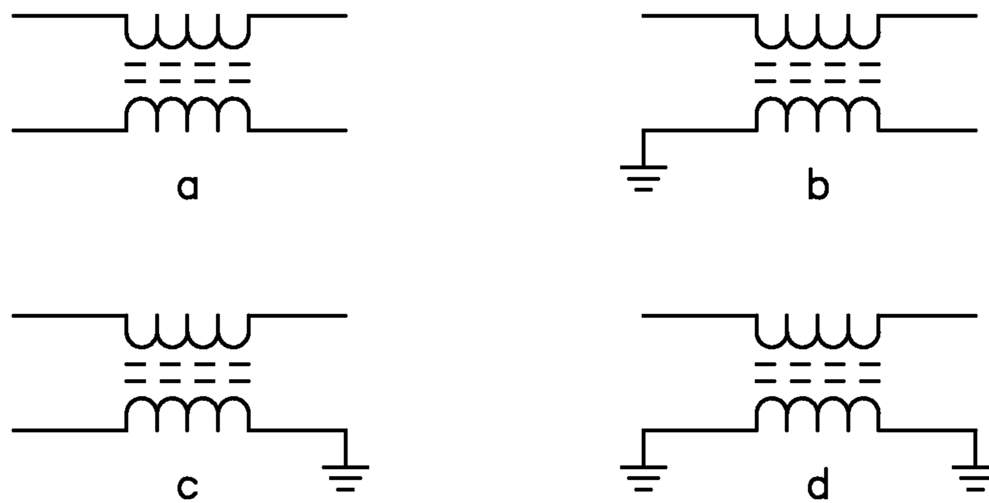
FIG. 2 PRIOR ART
