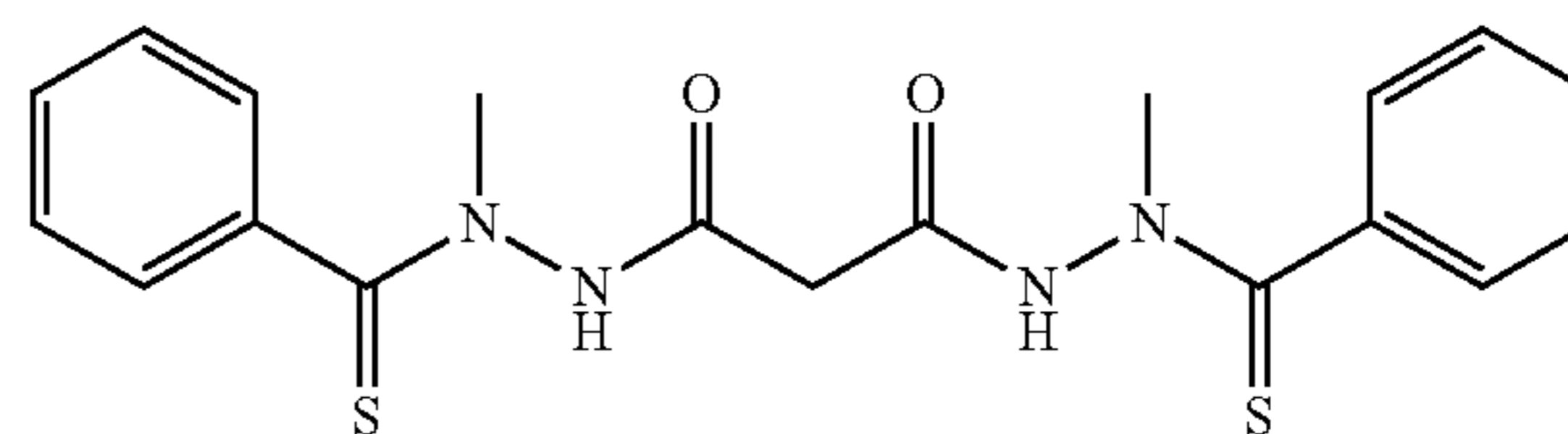
Compound A:
