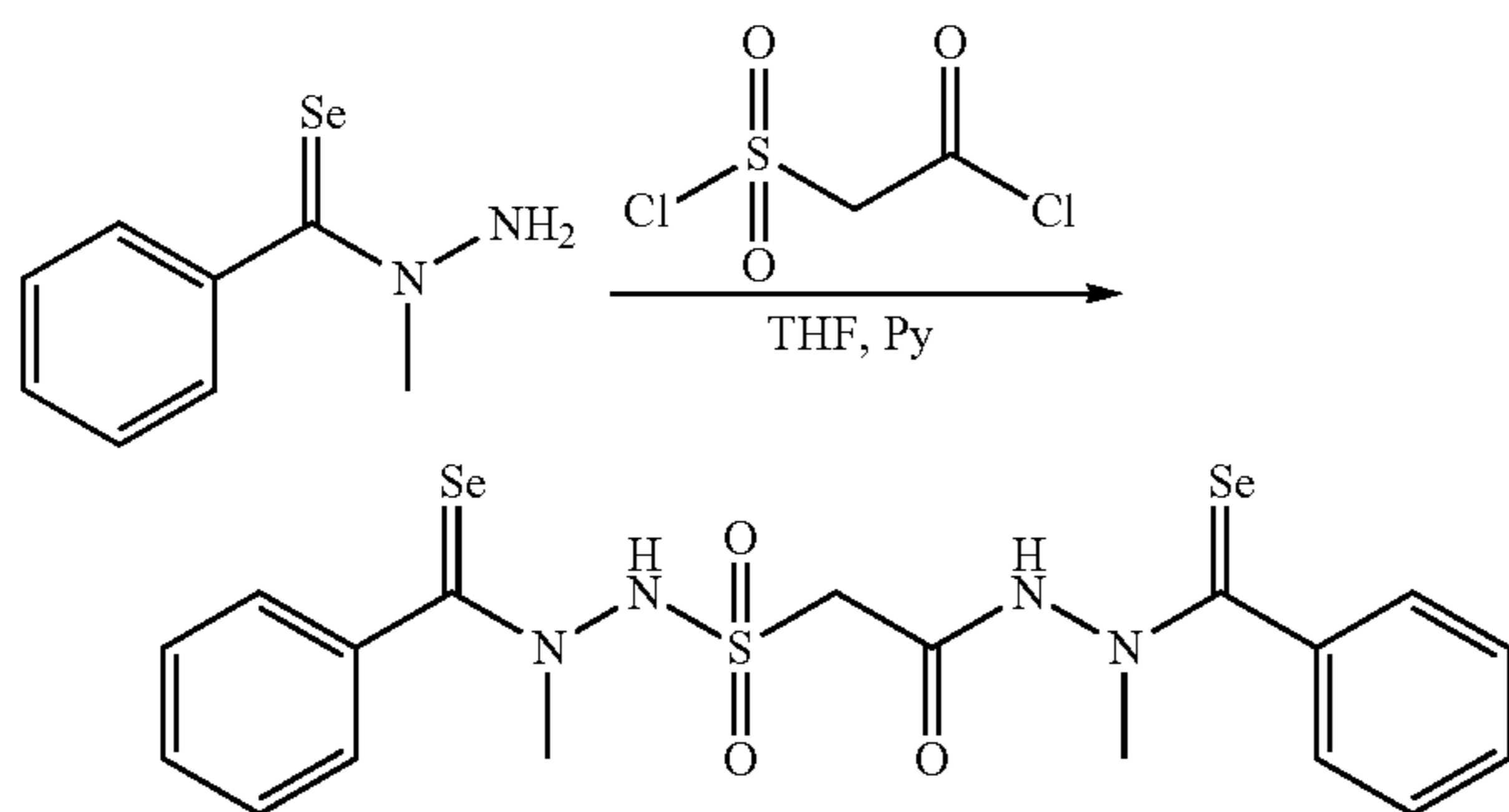
Compound 14
