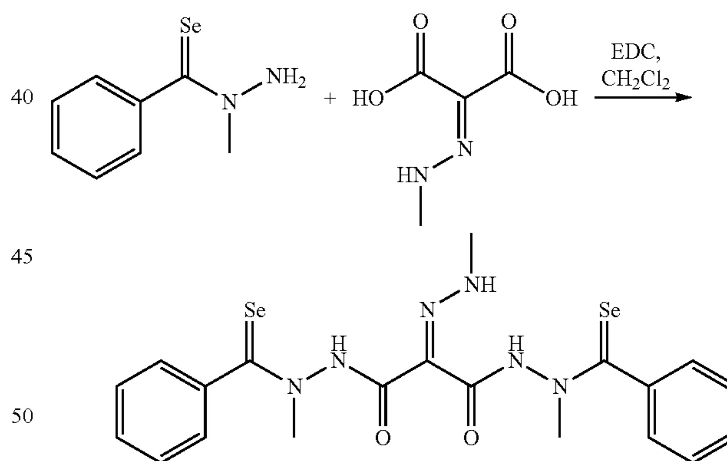
Compound 13
