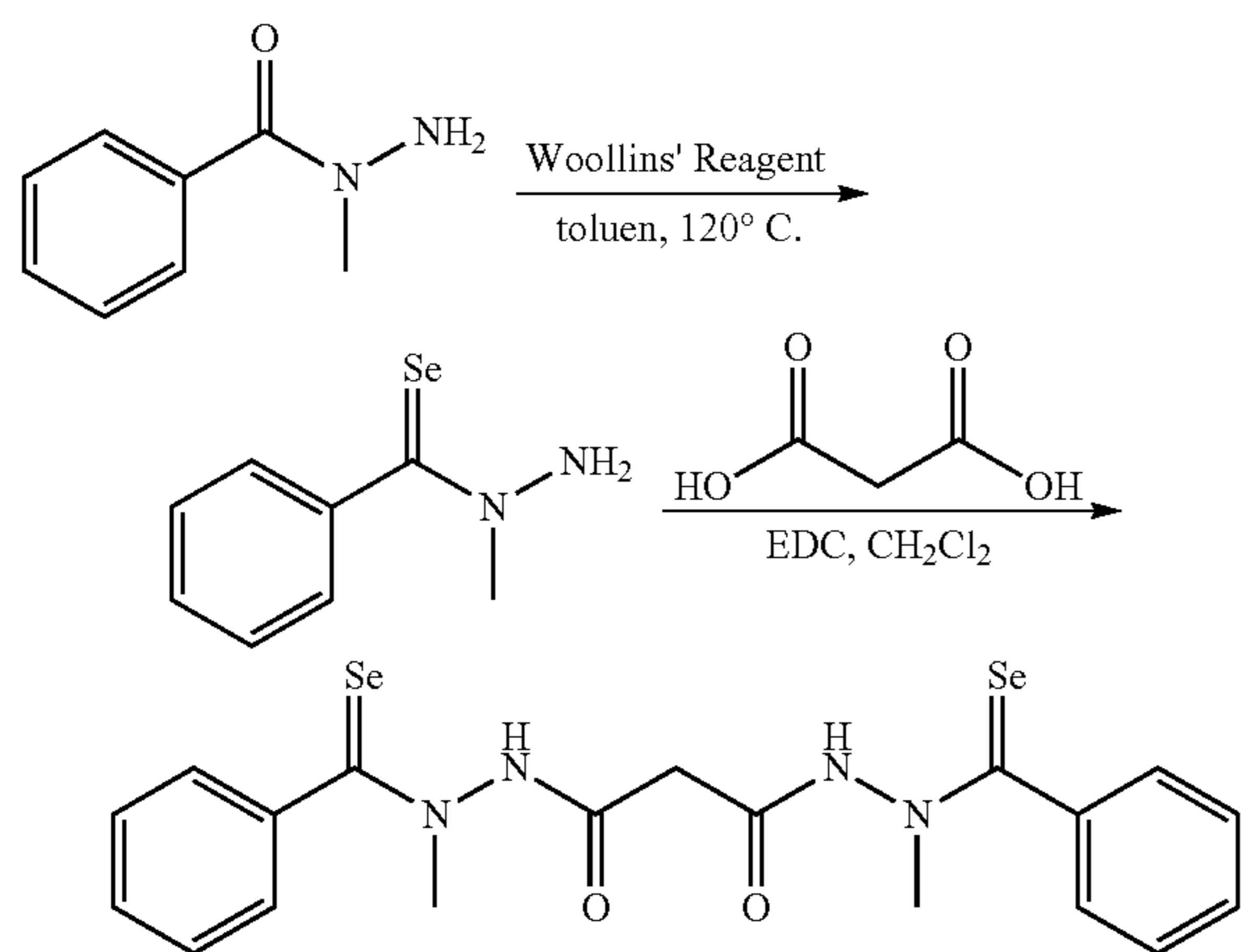
Compound 1
