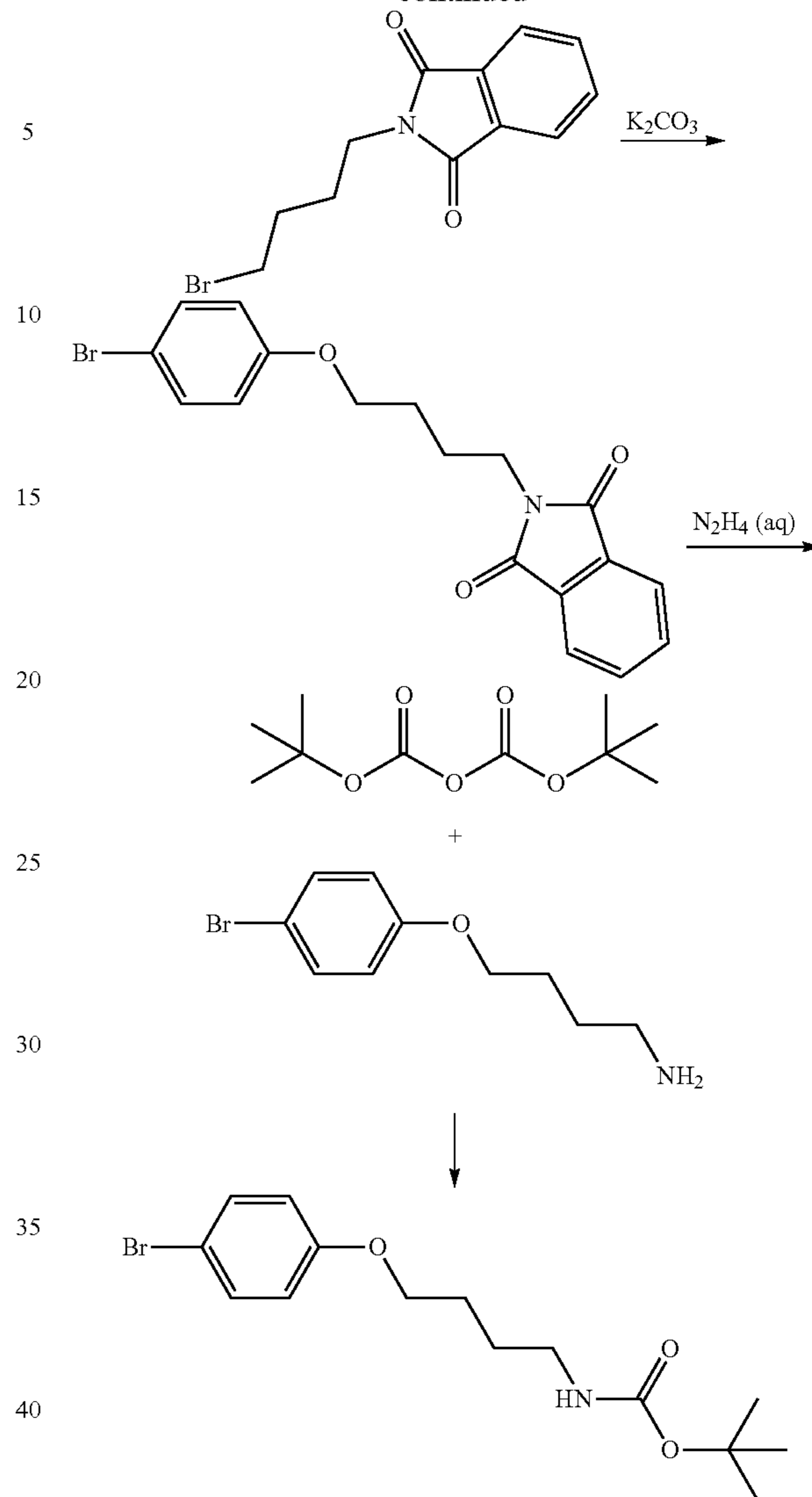
Step 1: N(4-(4-bromophenoxy)butyl)phthalimide
