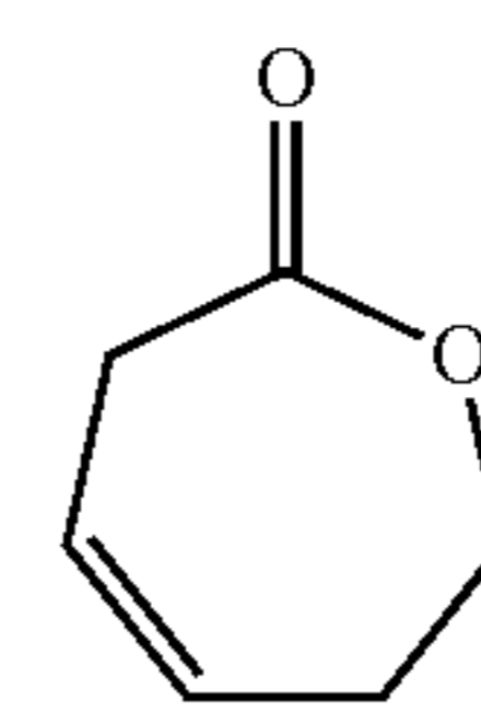
(Z)-6,7-Dihydrooxepan-2(3H)-one (DHXO)
