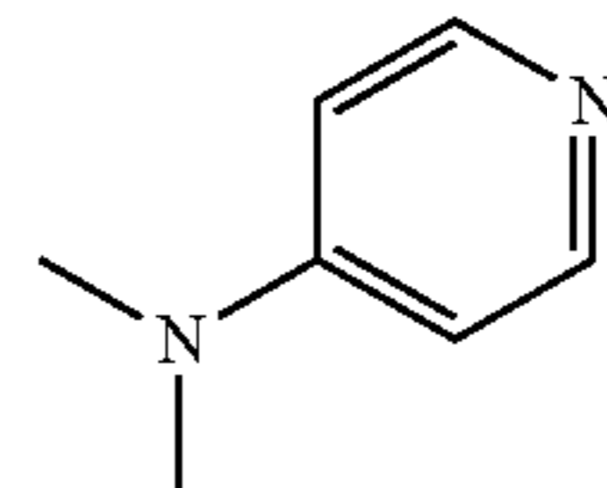
4-N,N-Dimethylaminopyridine (DMAP)
