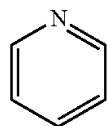
Pyridine (Py)
