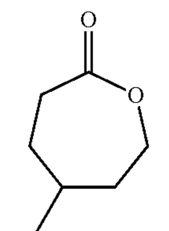
5-Methyloxepan-2-one (MXO)
