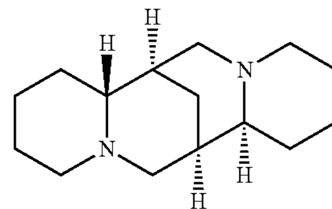
(-)-Sparteine (Sp)
