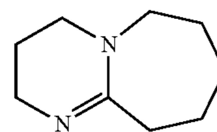
1,8-Diazabicyclo[5.4.0]undec-7-ene (DBU)
