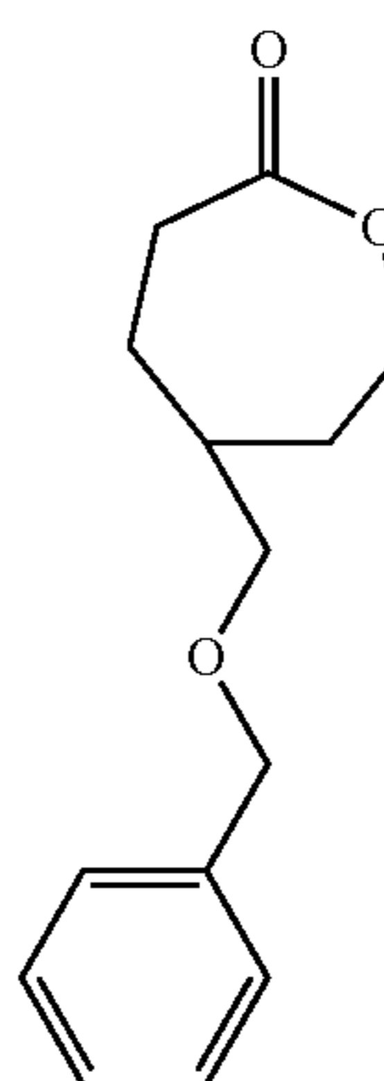
5-(Benzyloxymethyl)oxepan-2-one (BOMXO)
