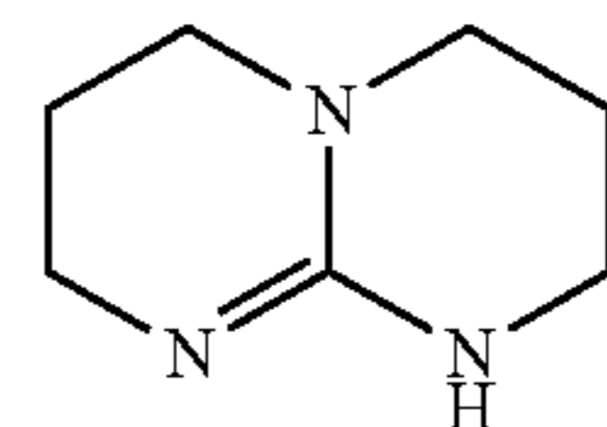
1,5,7-Triazabicyclo[4.4.0]dec-5-ene (TBD)
