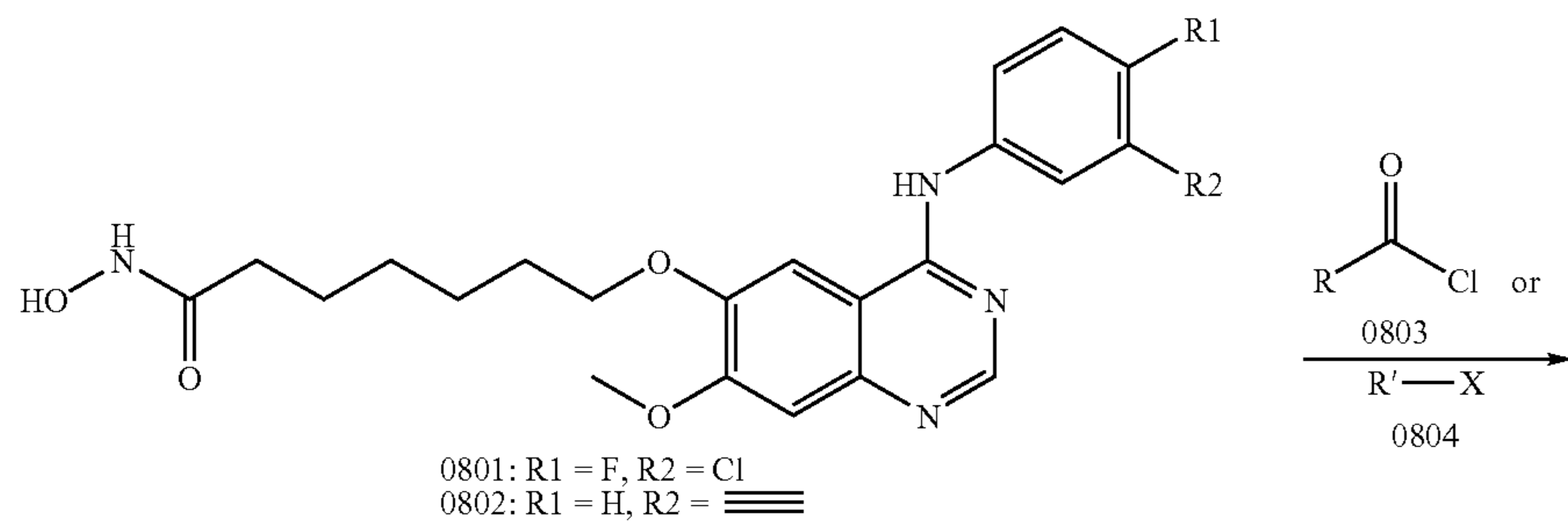
Scheme 8
