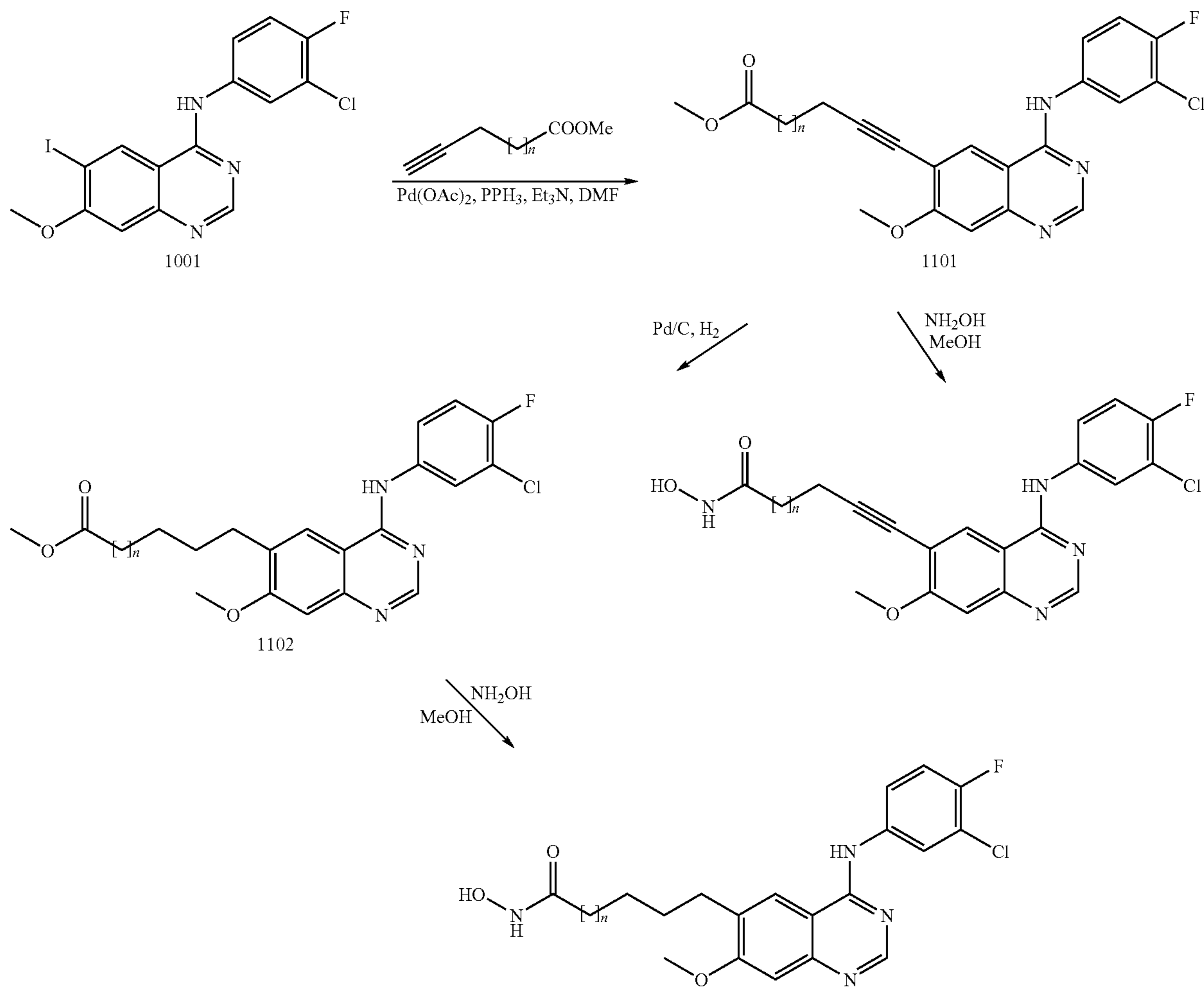
Scheme 11
