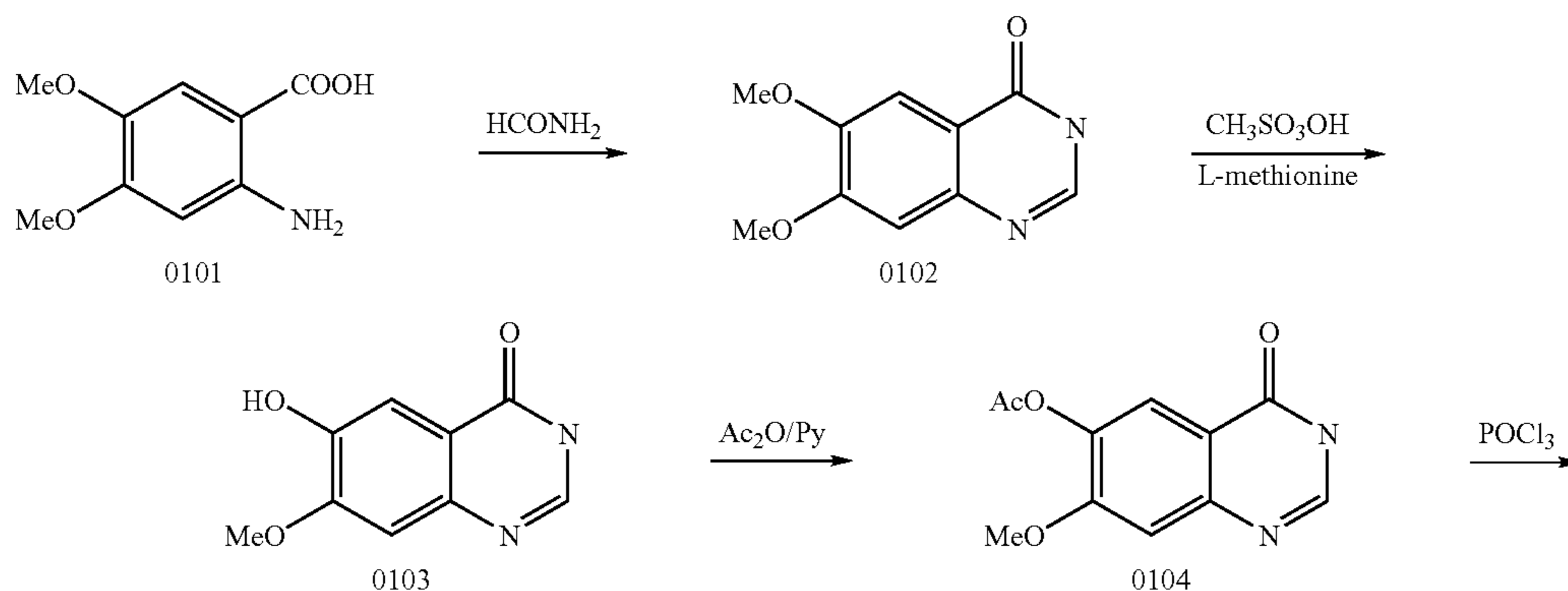
Scheme 1
