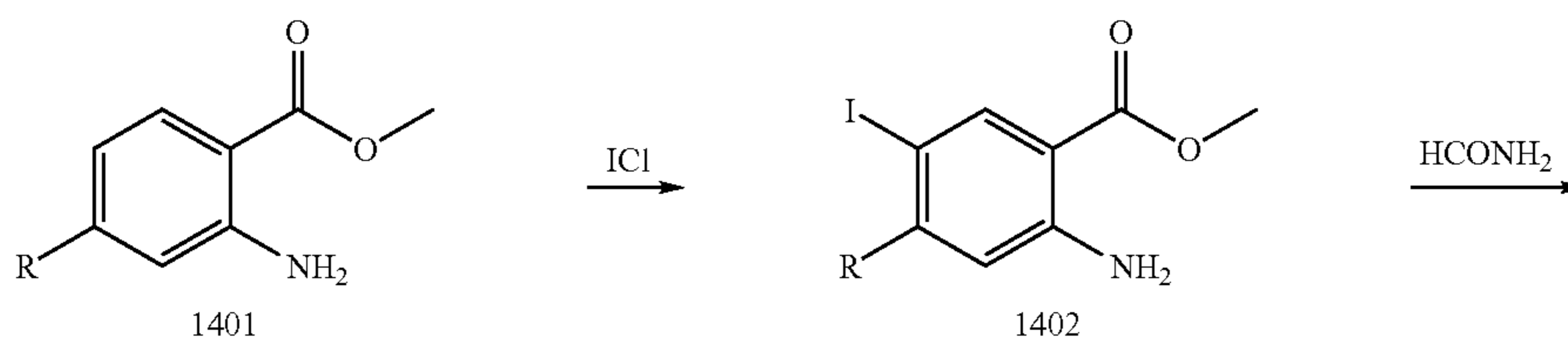
Scheme 14
