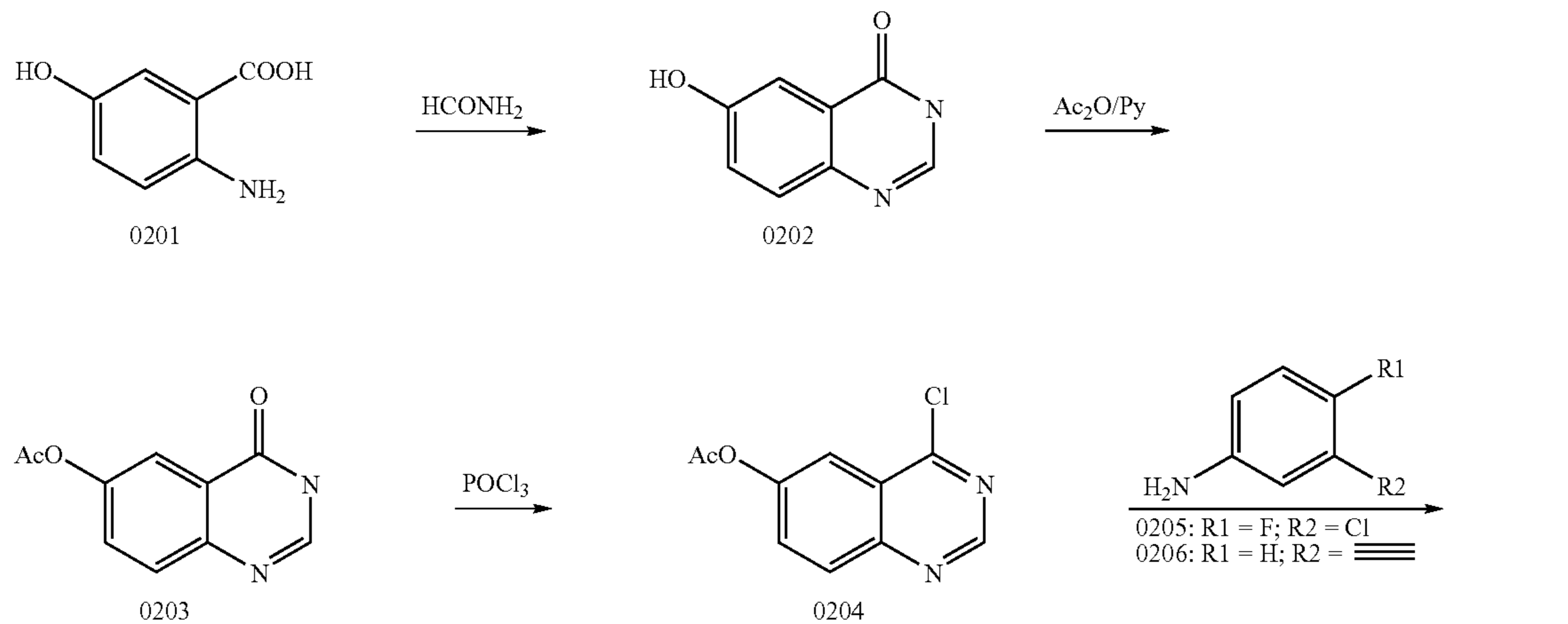
Scheme 2
