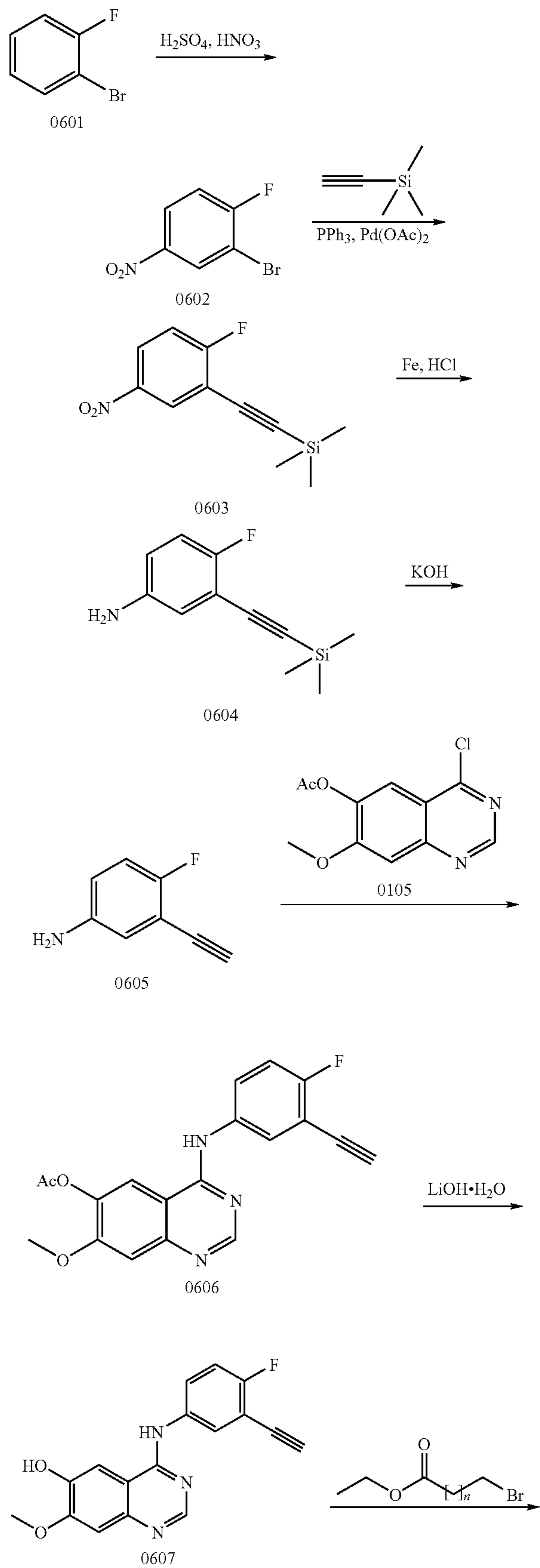
Scheme 6
