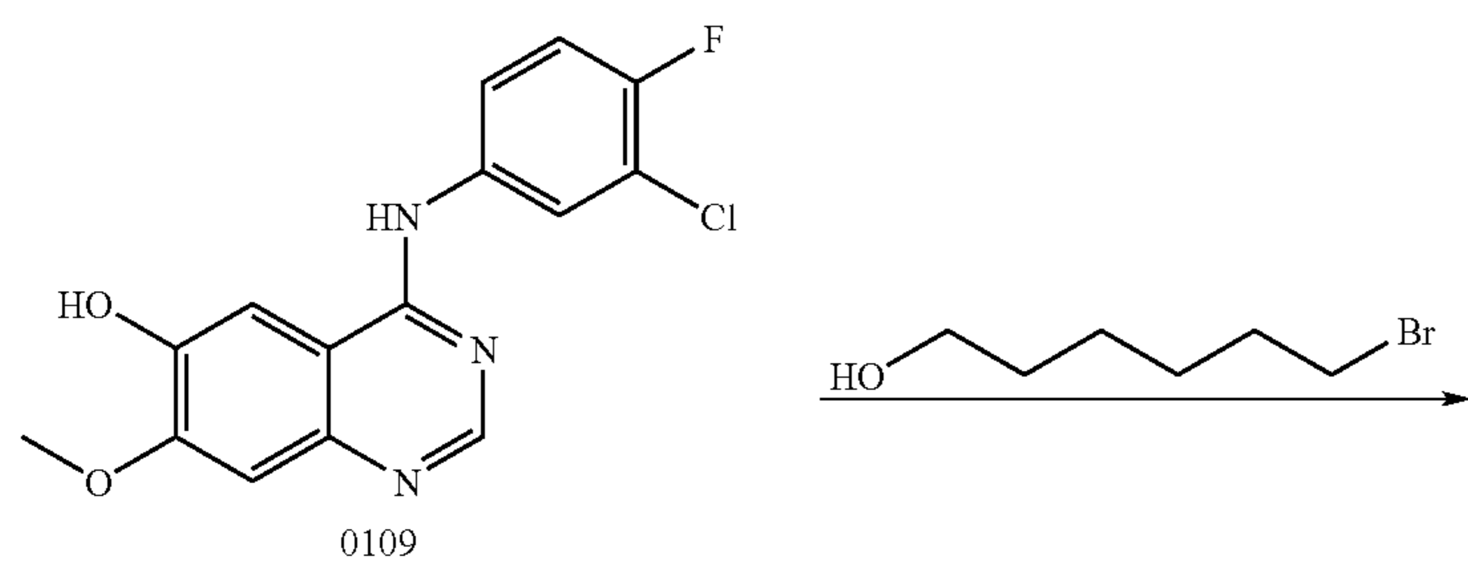
Scheme 9
