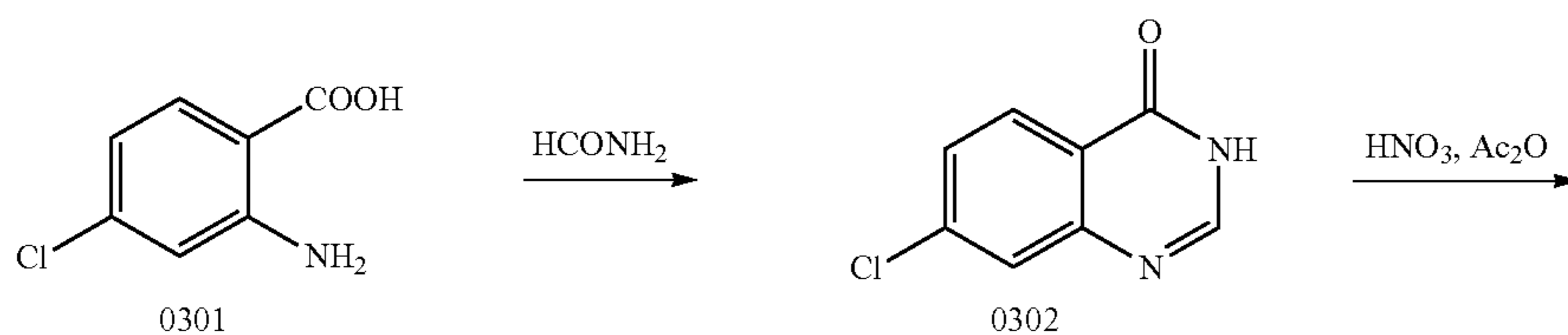
Scheme 3
