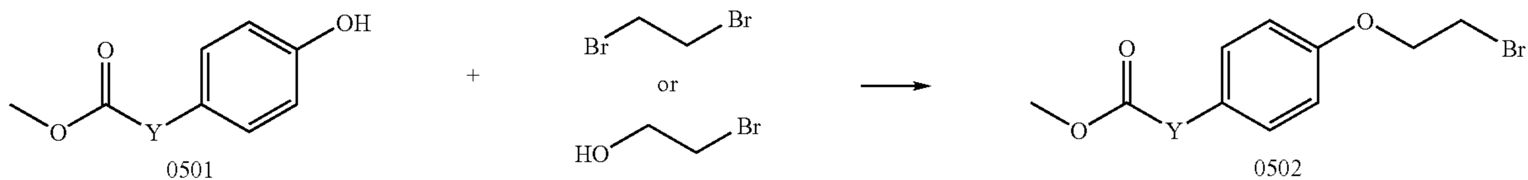
Scheme 5
