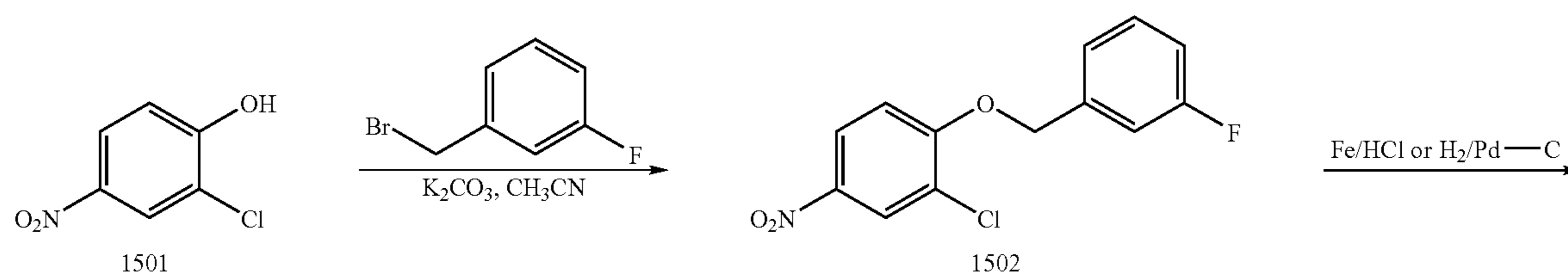
Scheme 15
