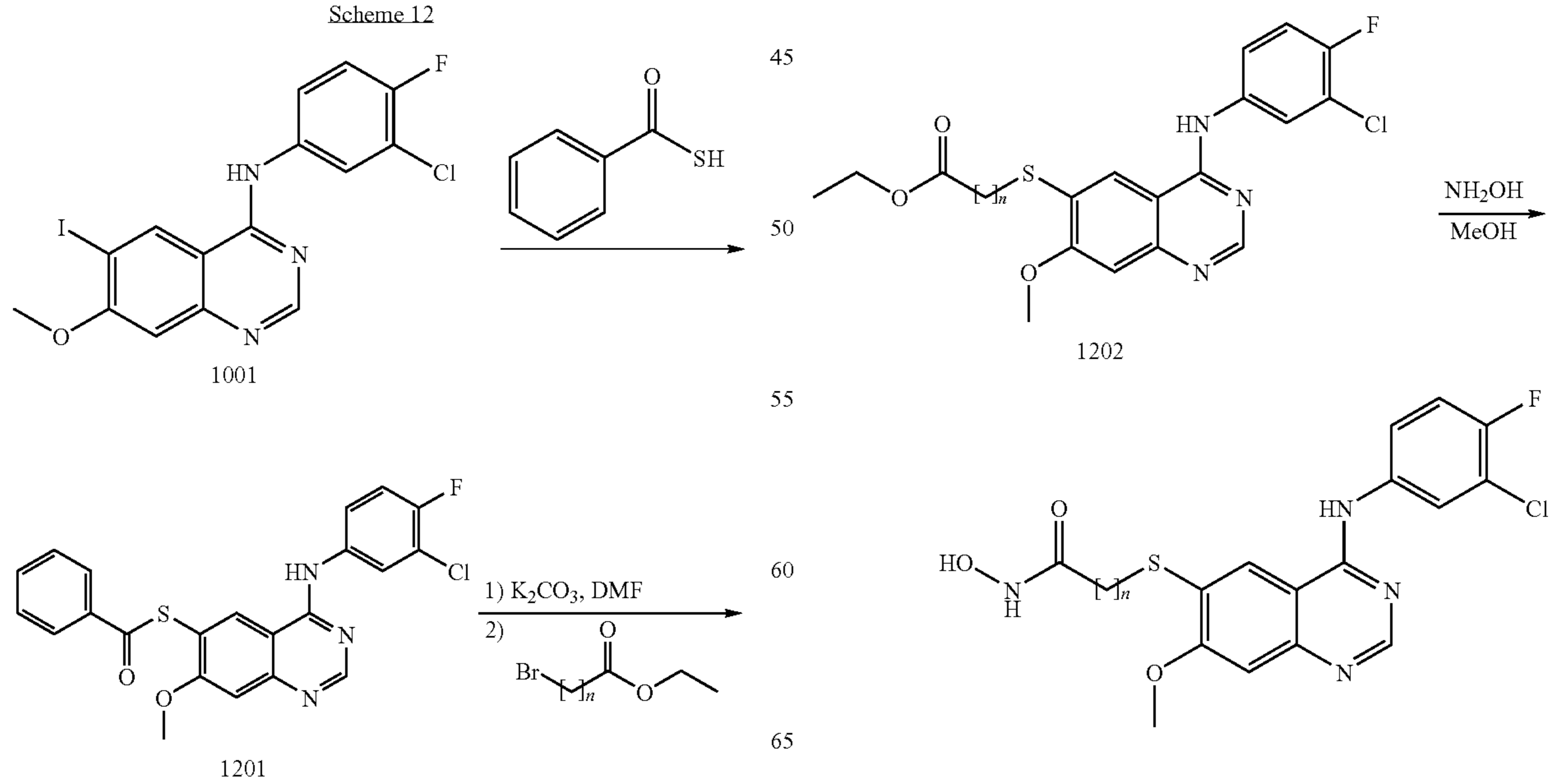
Scheme 12
