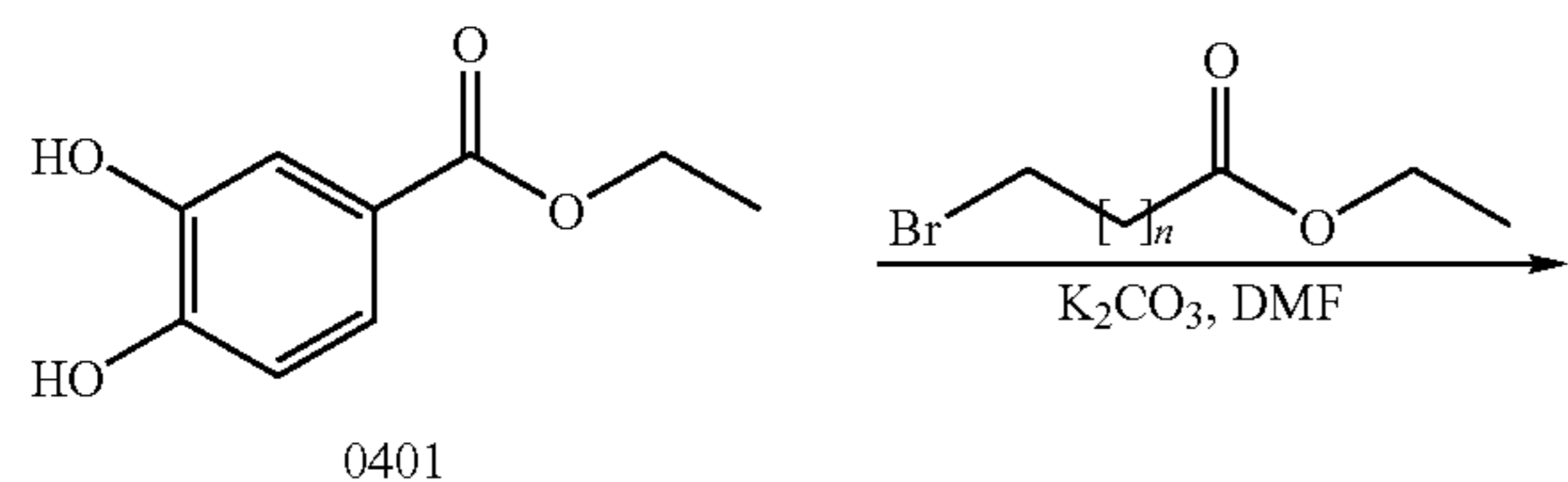
Scheme 13
