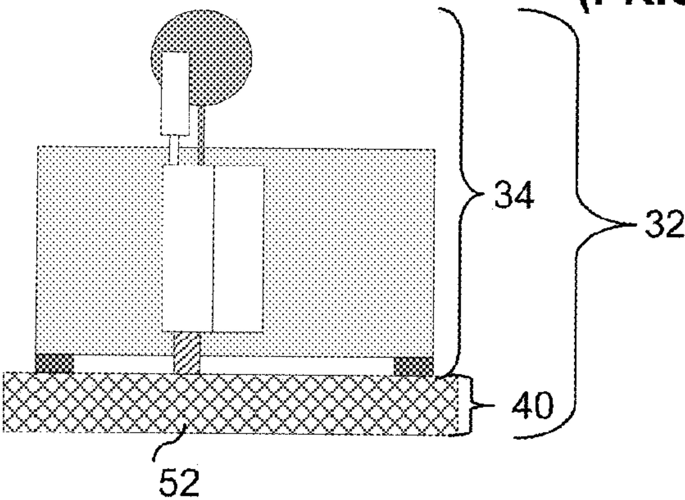
FIG. 3C (PRIOR ART)
