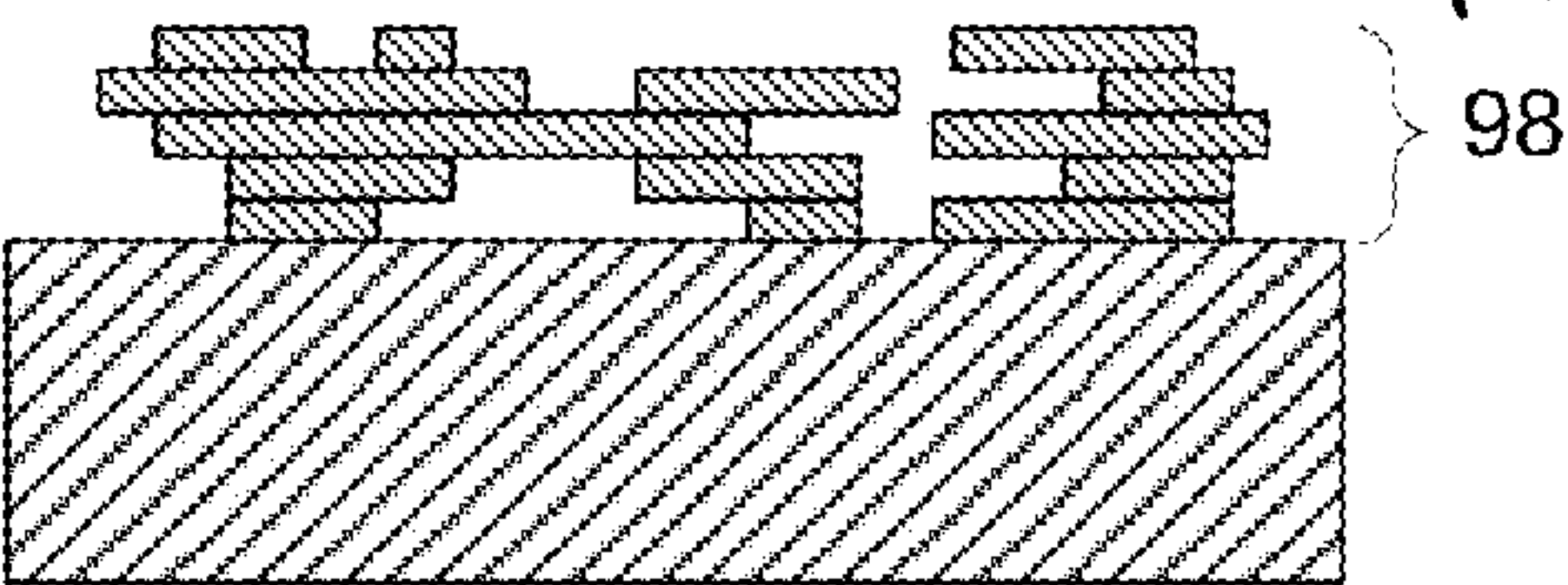
FIG. 4I (PRIOR ART)
