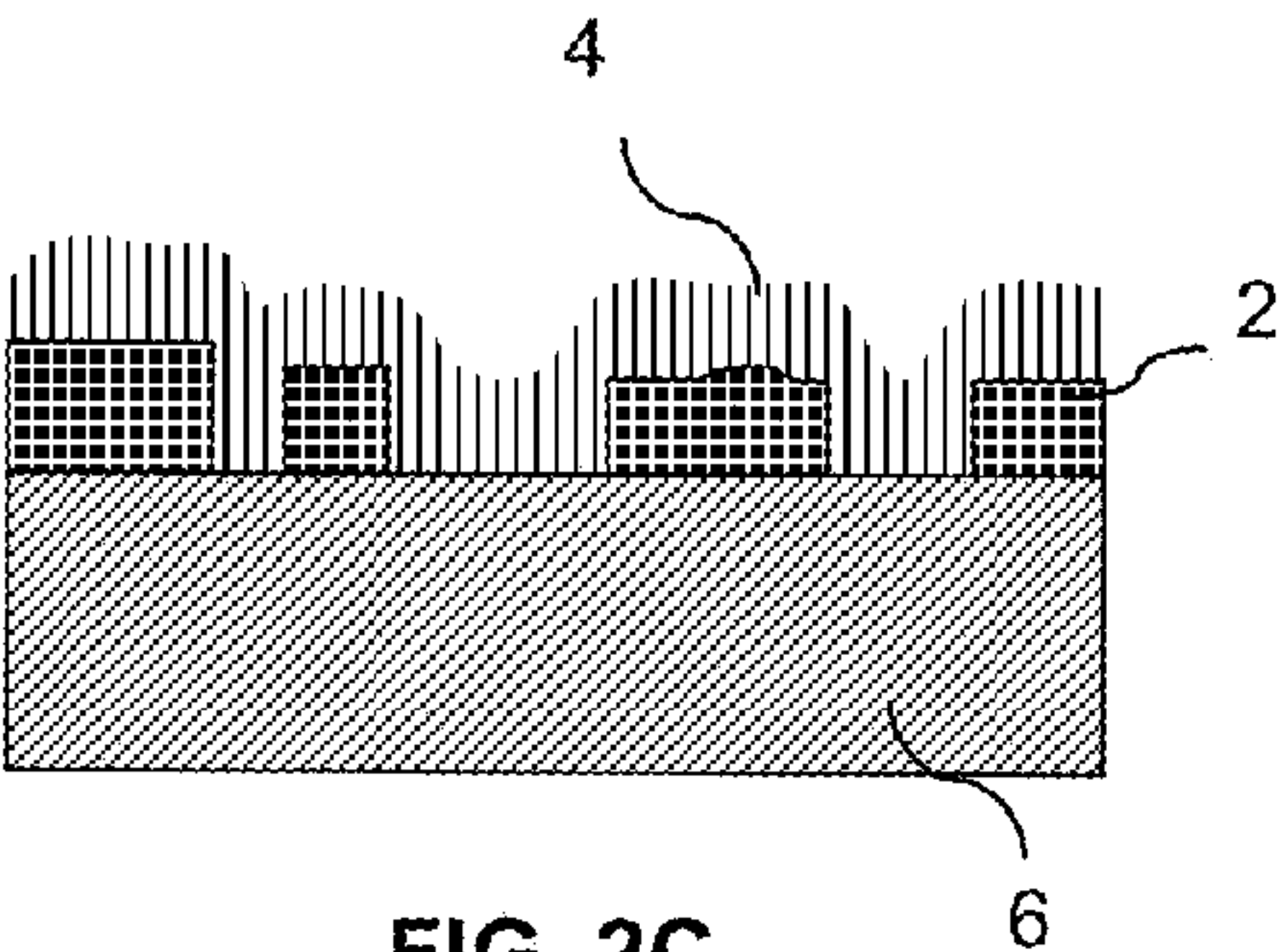
FIG. 2C (PRIOR ART)
