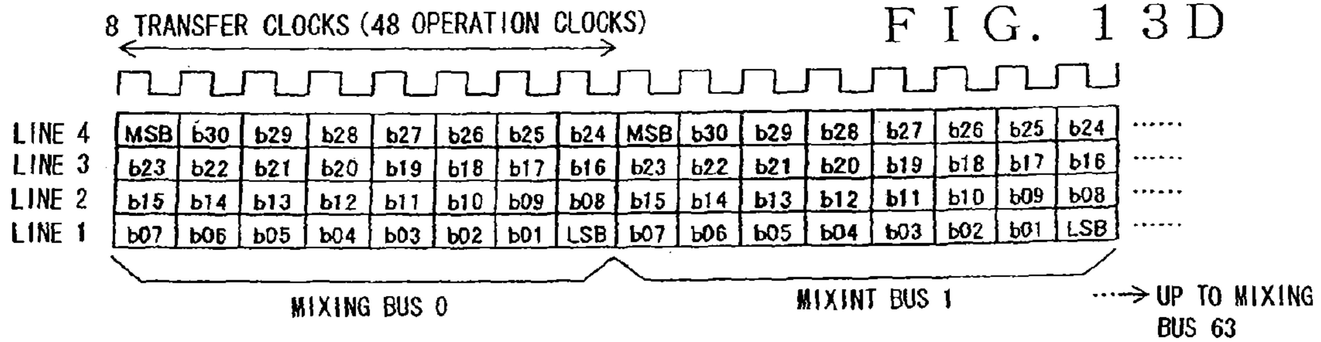
MODE 4 (48ch × 64bus), 4-LINE TRANSFER, TRANSFER CLOCK : 166/6MHz
