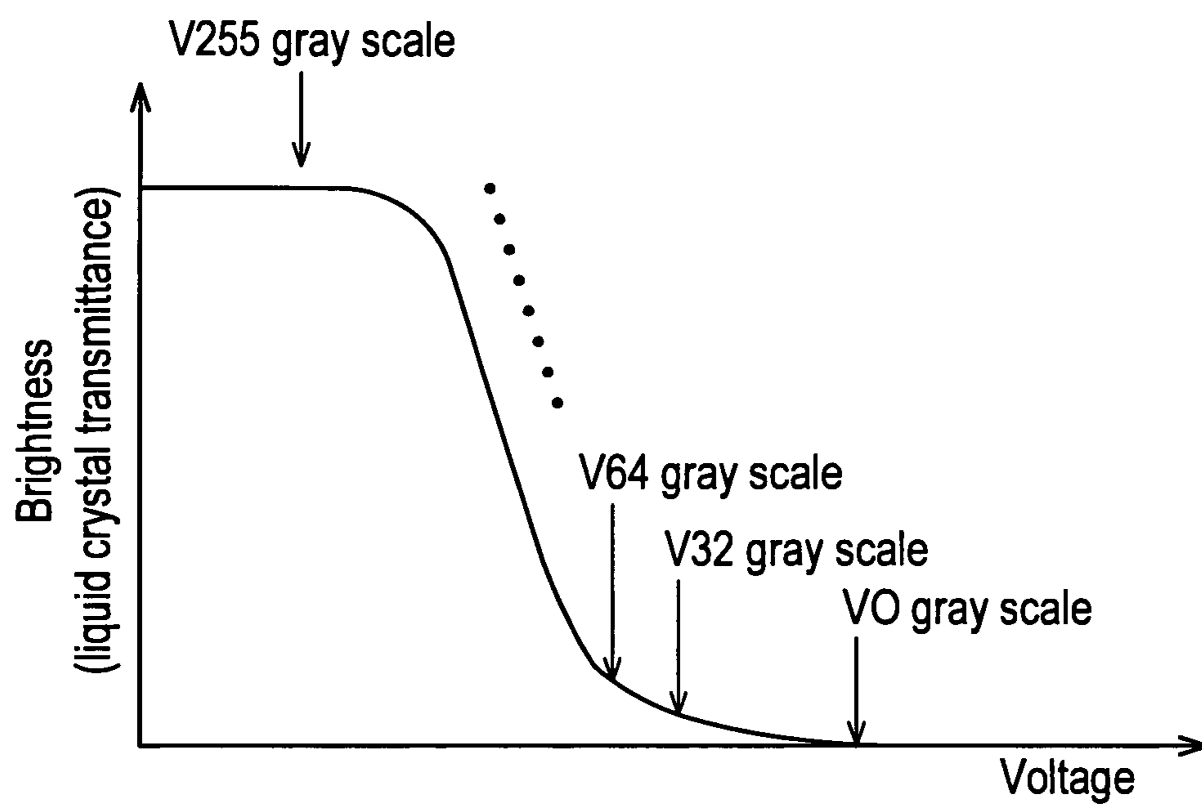
V-T characteristic voltage of a LCD panel
