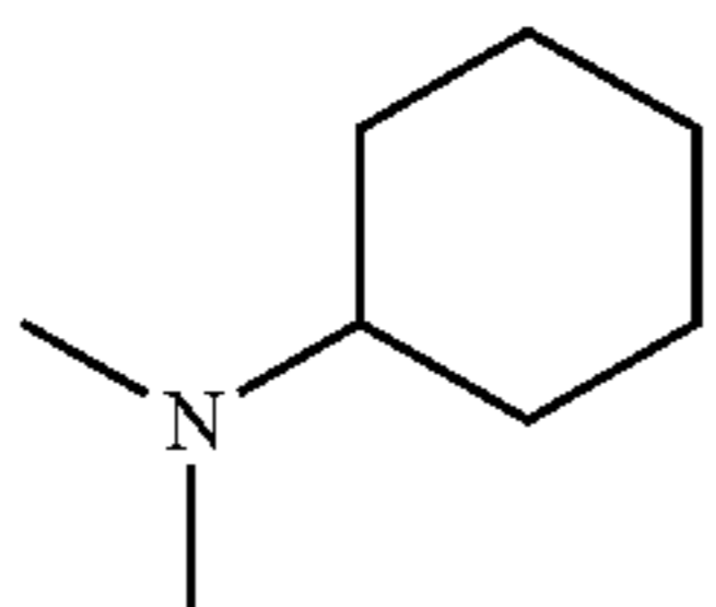
N,N-Dimethylaminocyclohexane (Me2NCy)
