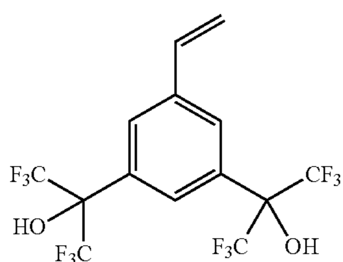
3,5-HFA-St
