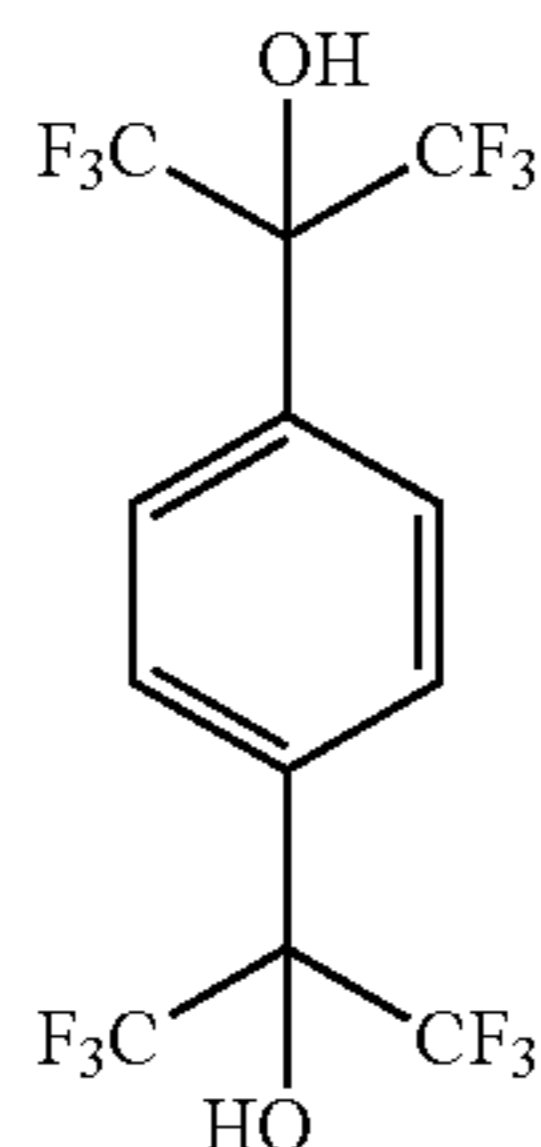
1,4-HFAB
