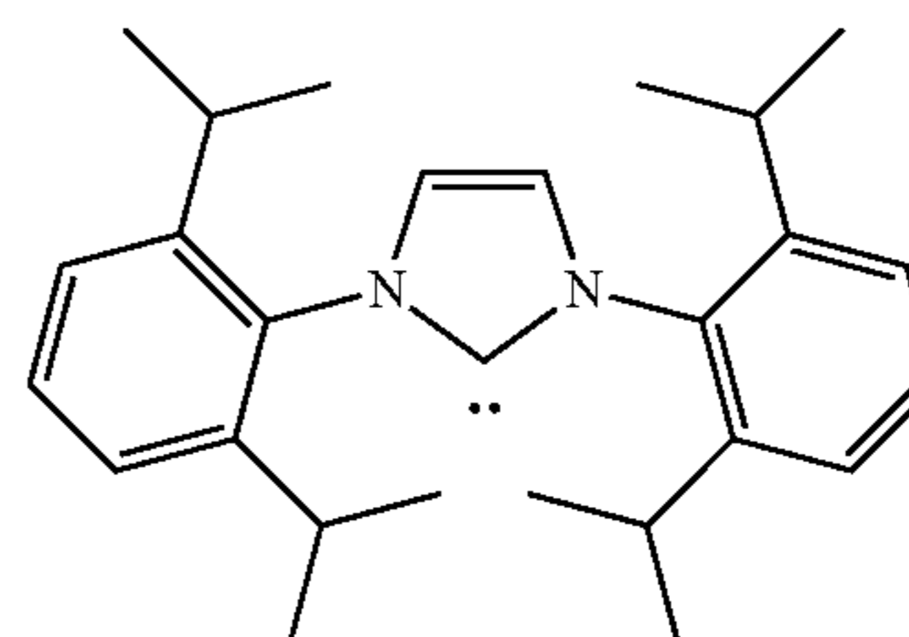
1,3-Bis(2,6-di-i-propylene)imidazol- 2-ylidene (Im-3)
