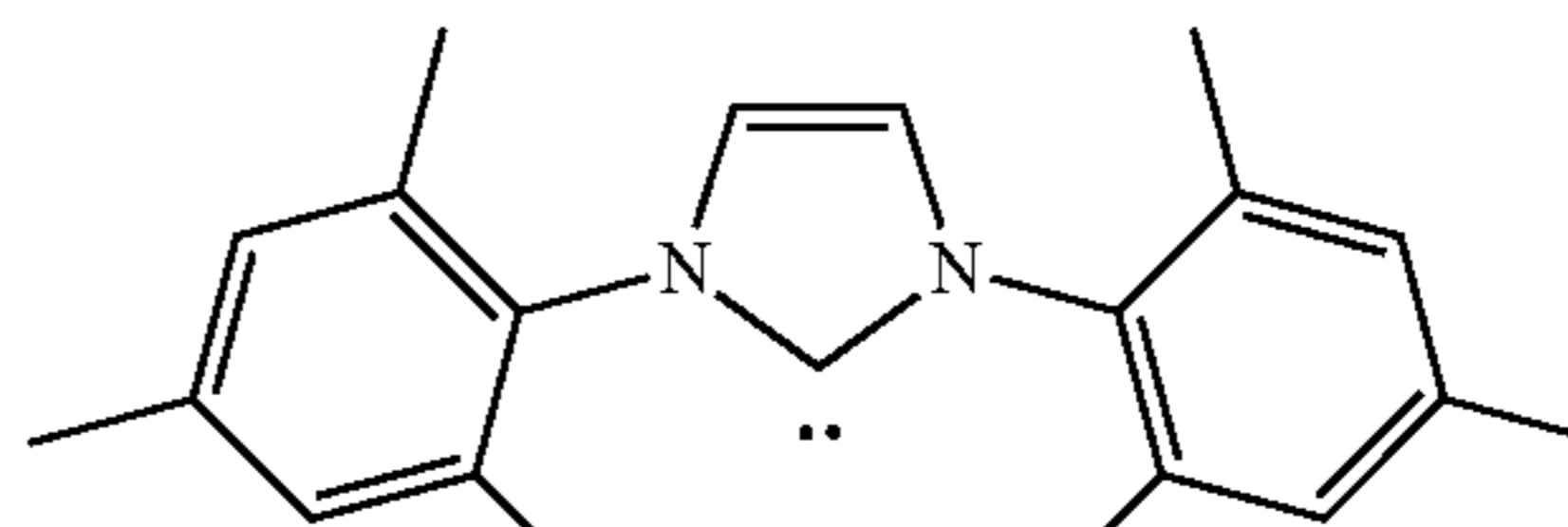
1,3-Bis(2,4,6-trimethylphenyl)imidazol-2- ylidene (Im-2)
