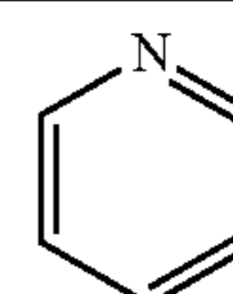
Pyridine (Py)
