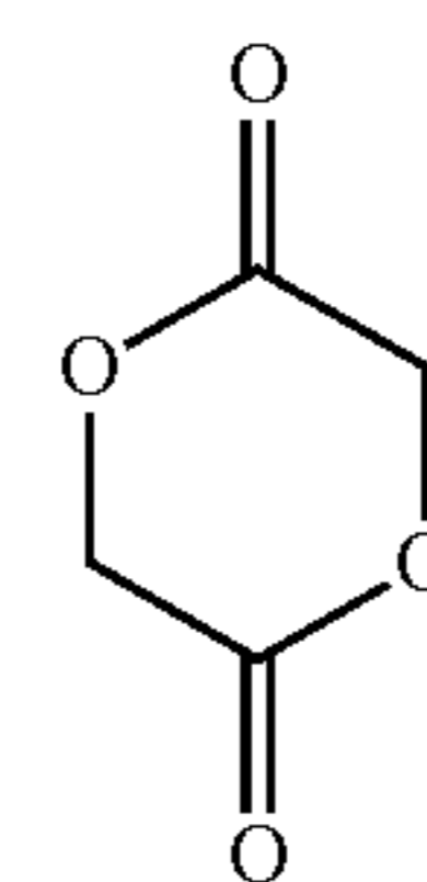
Glycolide (GLY)
