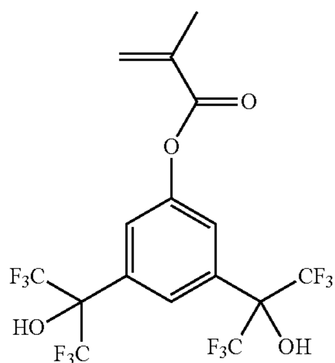
3,5-HFA-MA
