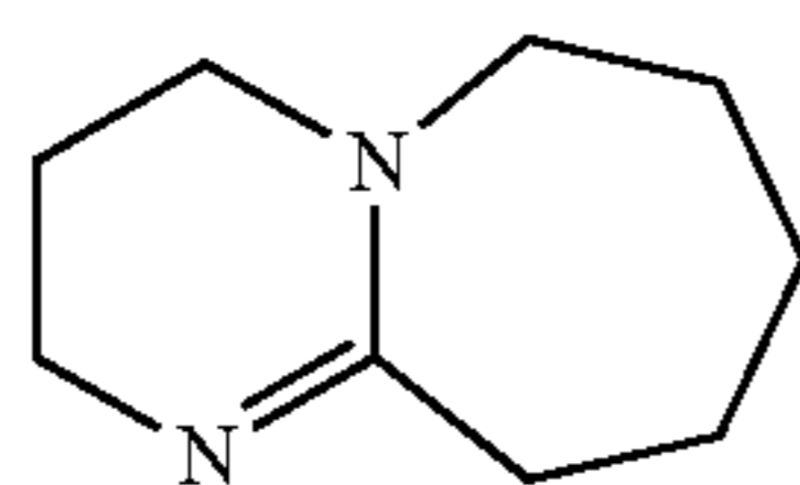
1,8-Diazabicyclo[5.4.0]undec-7-ene (DBU)
