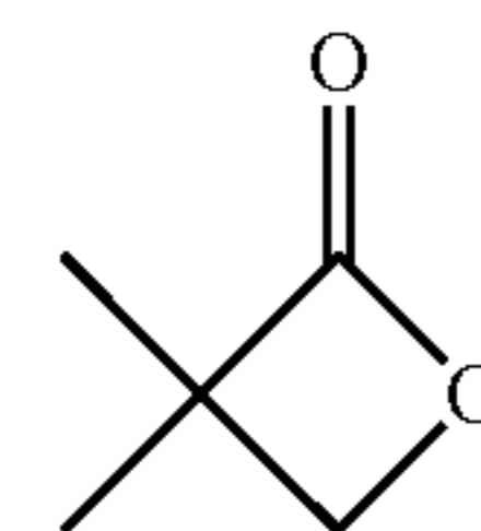
Pivalolactone (PVL)
