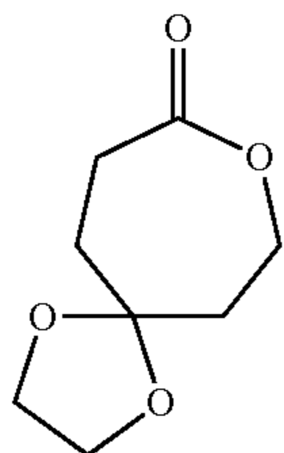
1,4,8-Trioxa(4,6)spiro-9-undecane (TOSU)
