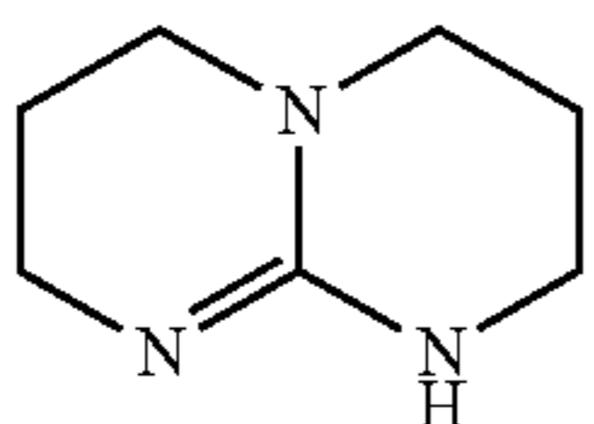
1,5,7-Triazabicyclo[4.4.0]dec-5-ene (TBD)
