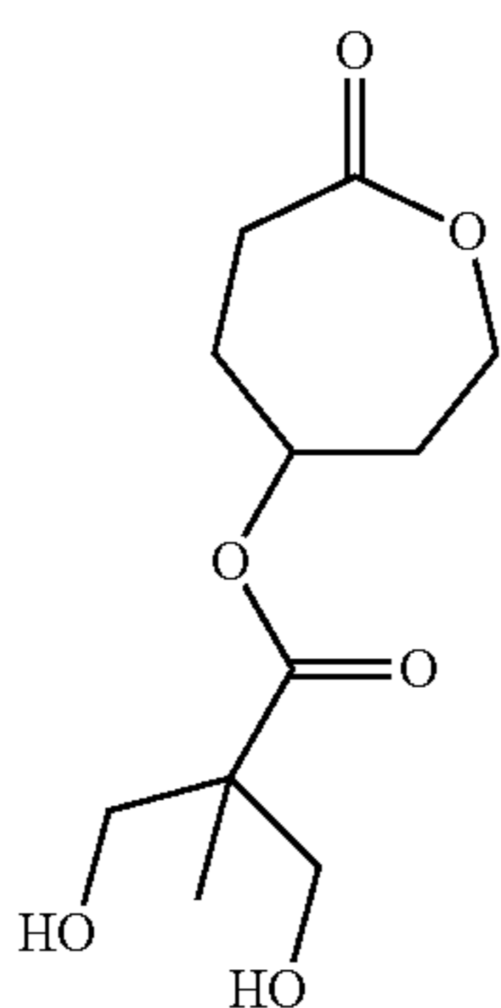
7-Oxooxepan-4-yl 3-hydroxy-2- (hydroxymethyl)-2-methylpropanoate
