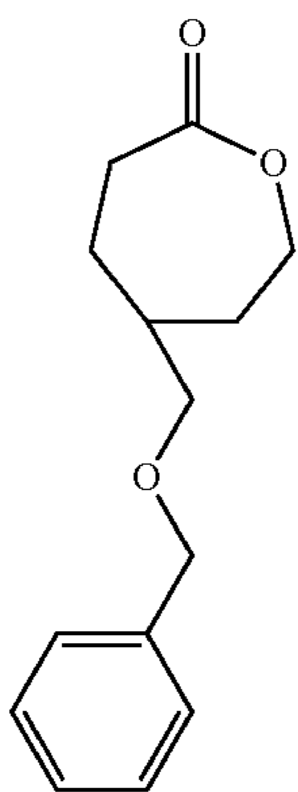
5-(Benzyloxymethyl)oxepan-2-one (BOMXO)
