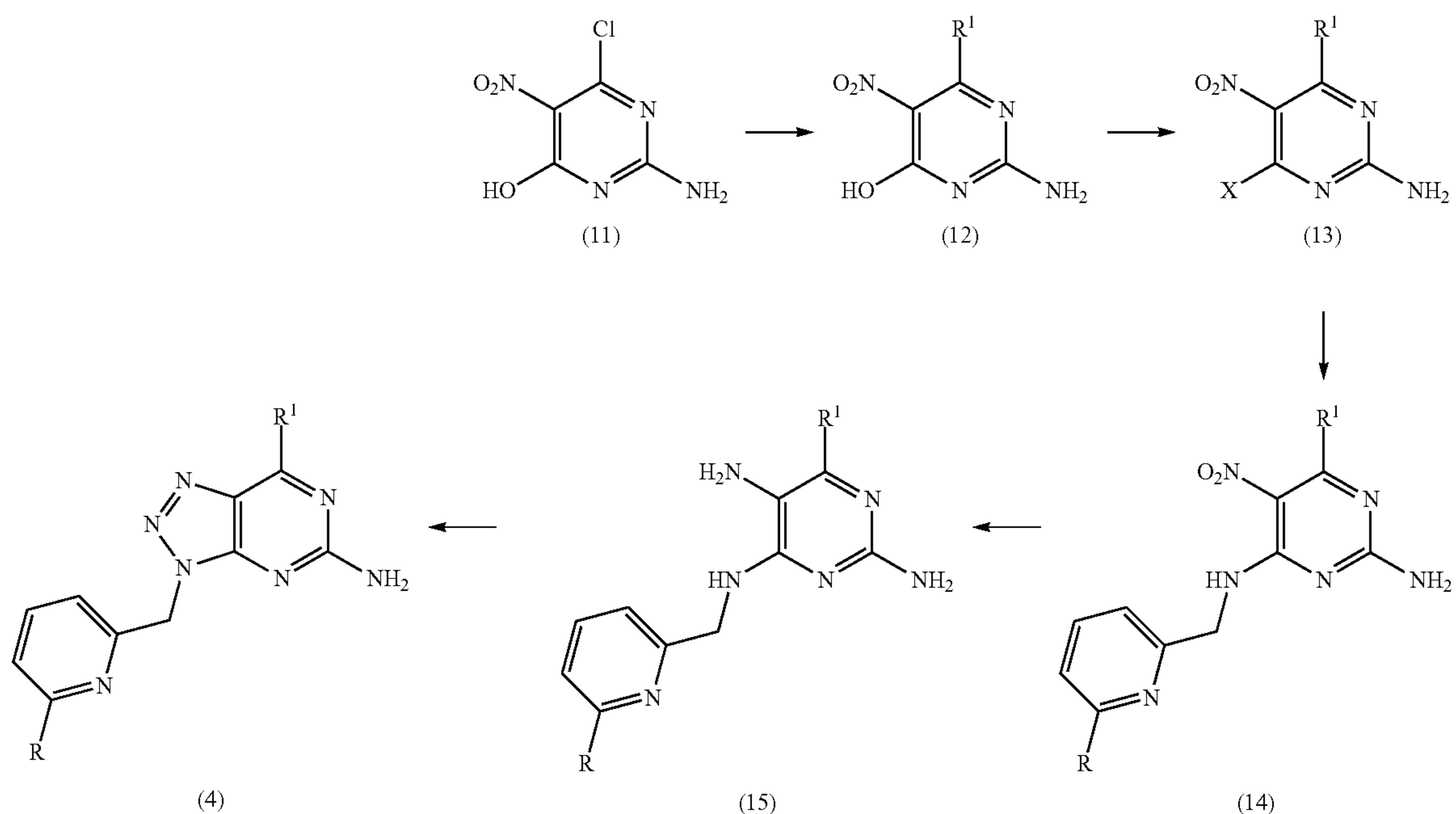
Reaction Scheme 3
