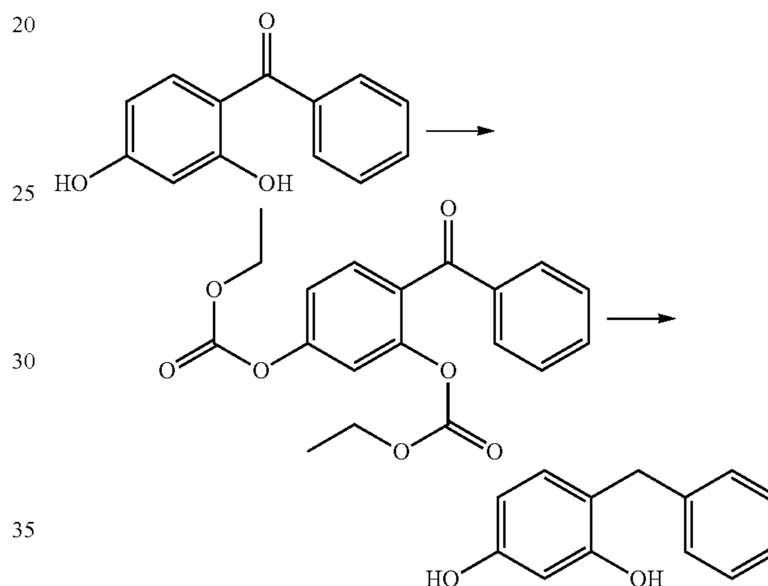
Carbonic acid 2-benzoyl-5-ethoxycarbonyloxy-phenyl ester ethyl ester
