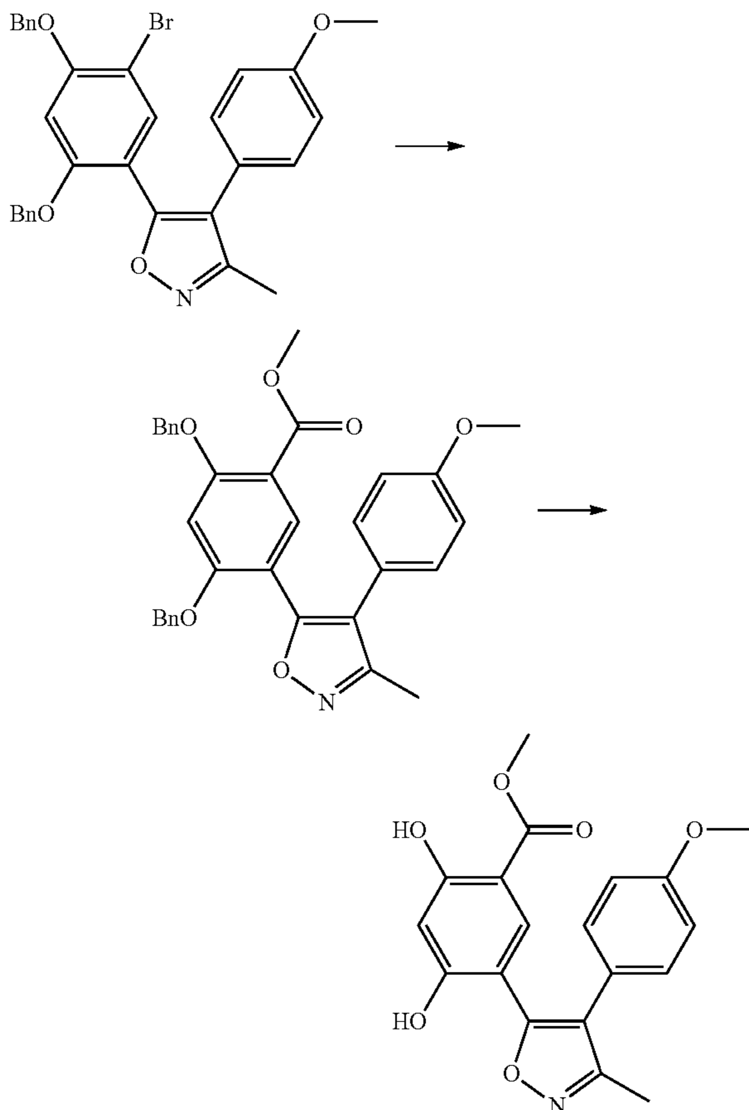
Scheme 3: formation of ester
