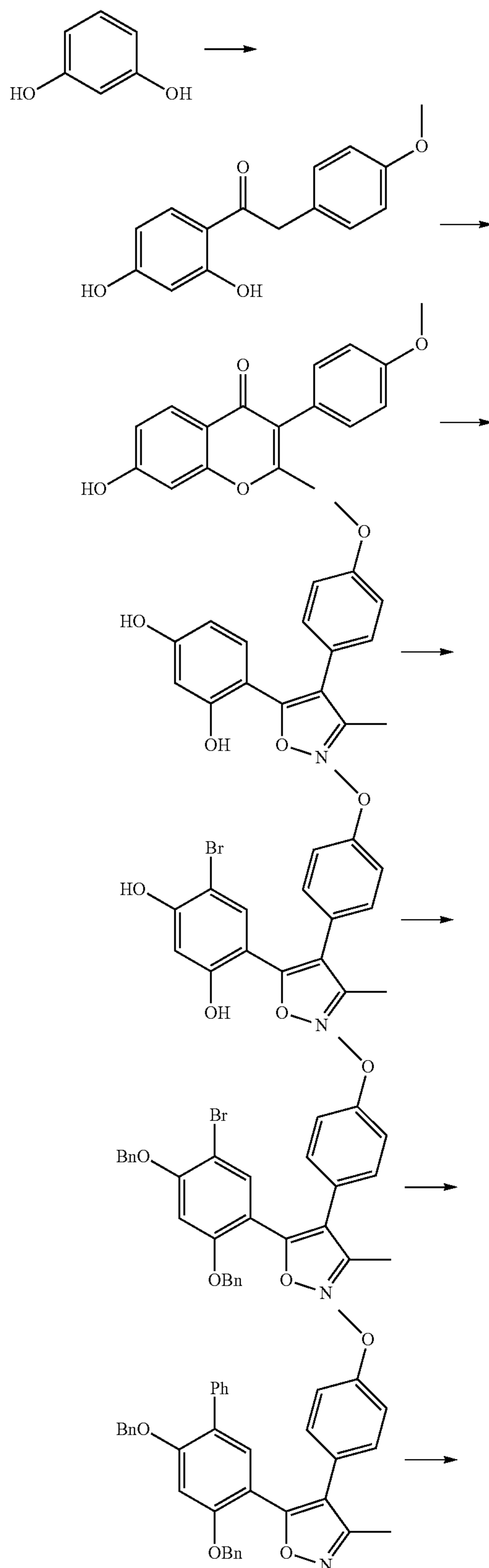
Scheme 1: preparation of bromo intermediate and subsequent arylation
