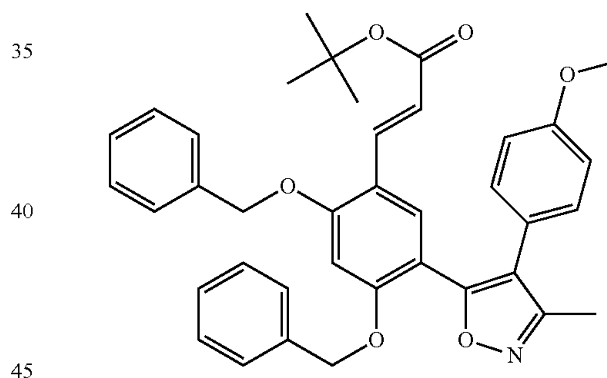
3-{2,4-Dihydroxy-5-[4-(4-methoxy-phenyl)-3-methyl-isoxazol-5-yl]phenyl}-acrylic acid
