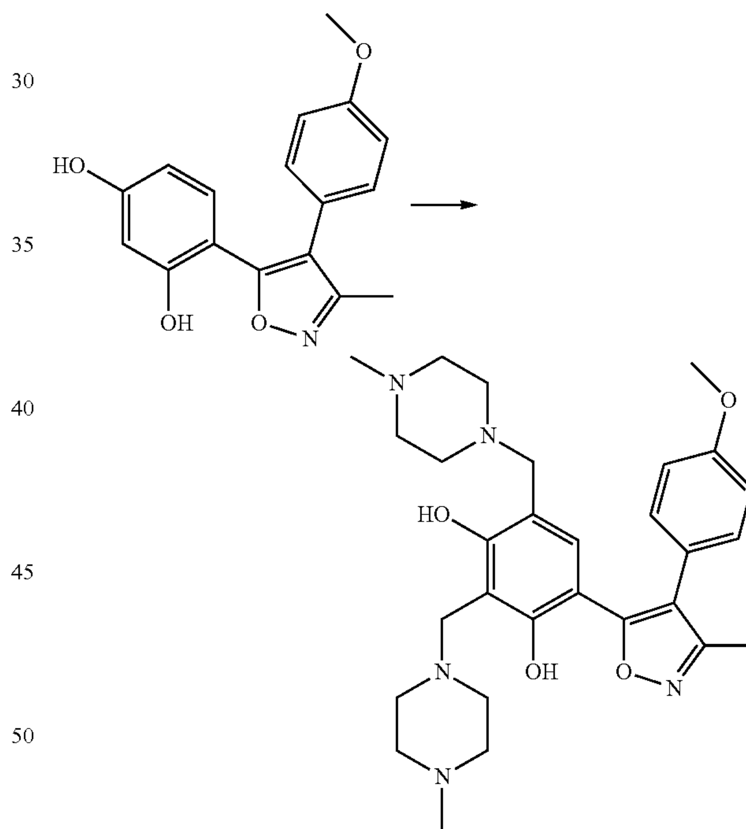
Scheme 2: Mannich reaction
