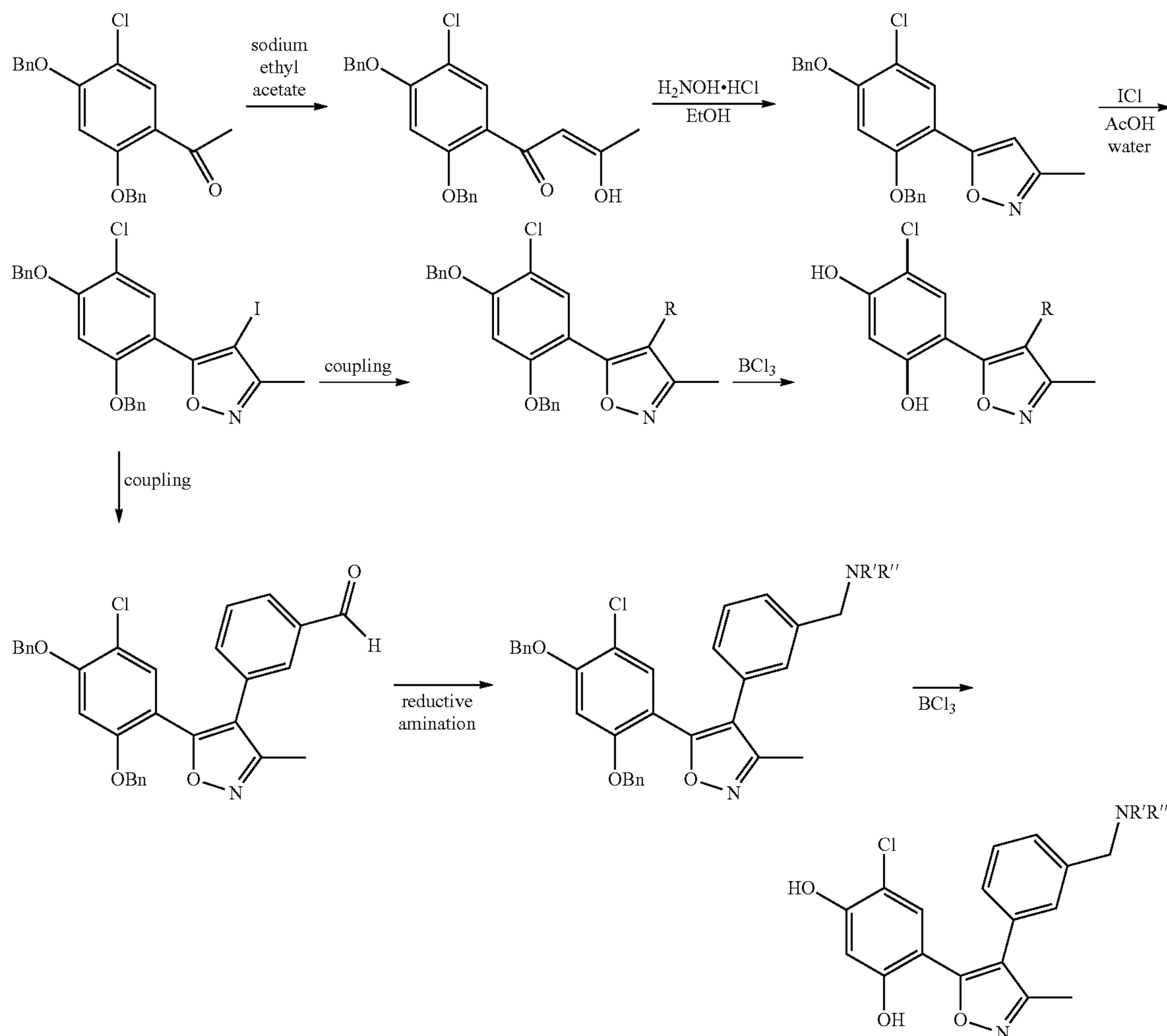
Scheme 7: Preparation of 5-(2,4-bis-benzyloxy-5-chloro-phenyl)-4-iodo-3-methyl-isoxazole intermediate
