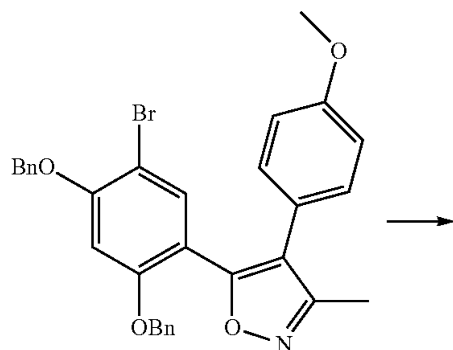
Scheme 5: Heck reaction and boron trichloride deprotection
