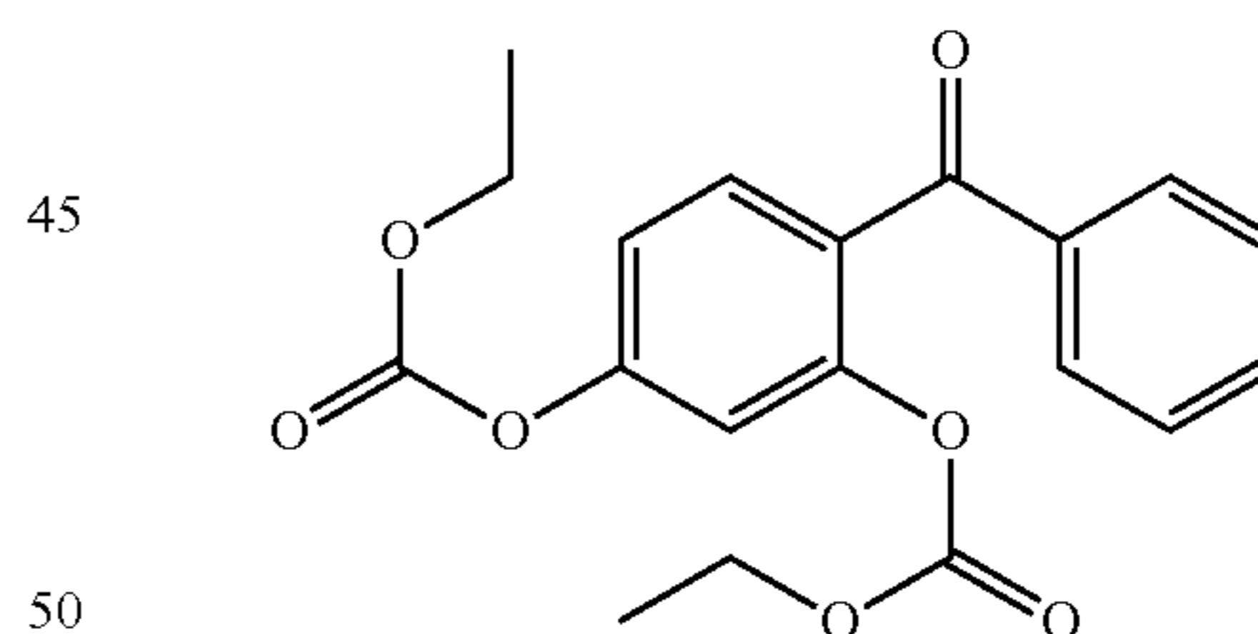
Carbonic acid 2-benzoyl-5-ethoxycarbonyloxy-phenyl ester ethyl ester
