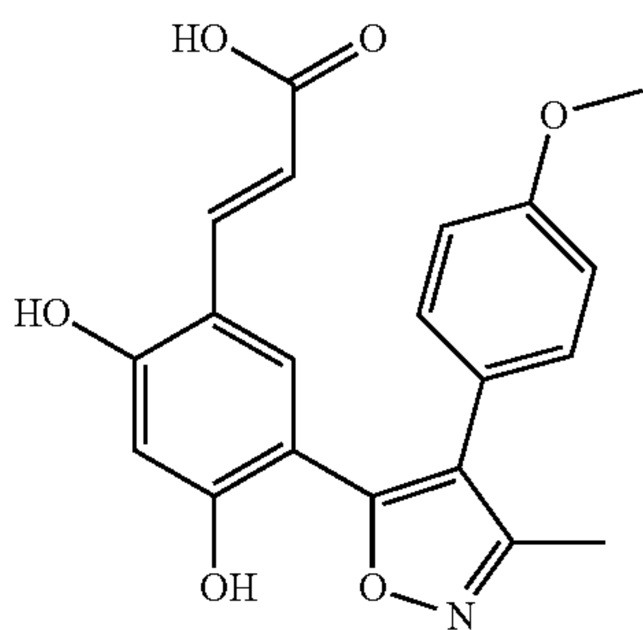
3-{2,4-Dihydroxy-5-[4-(4-methoxy-phenyl)-3-methyl-isoxazol-5-yl]phenyl}-acrylic acid
