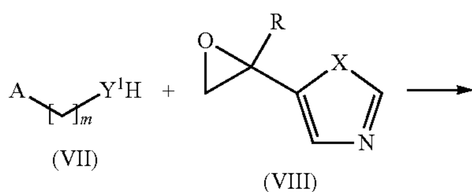
Scheme 3: Process C (n = 0, R 1 = H)
