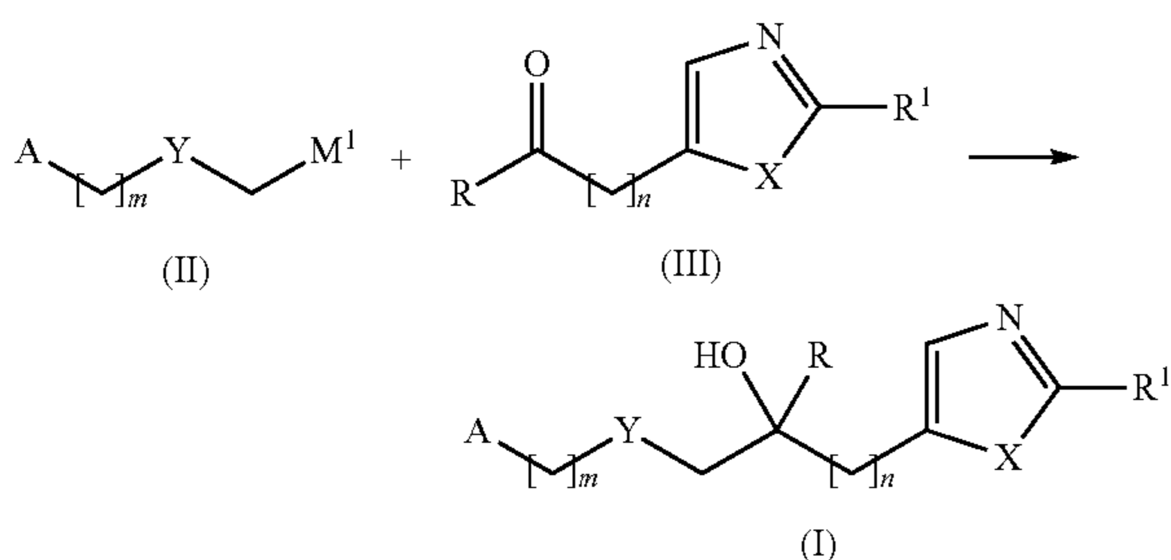
Scheme 1: Process A
