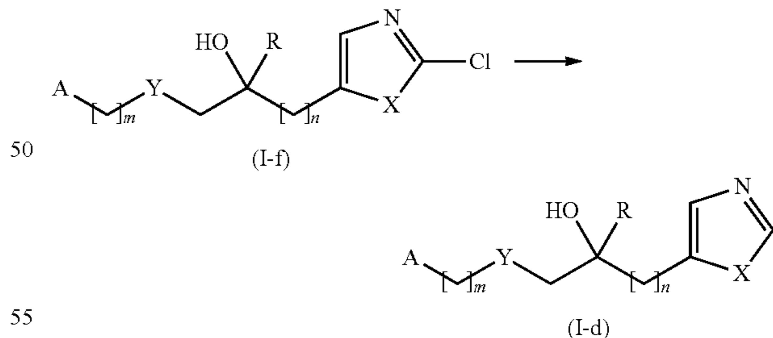
Scheme 6: Process F
