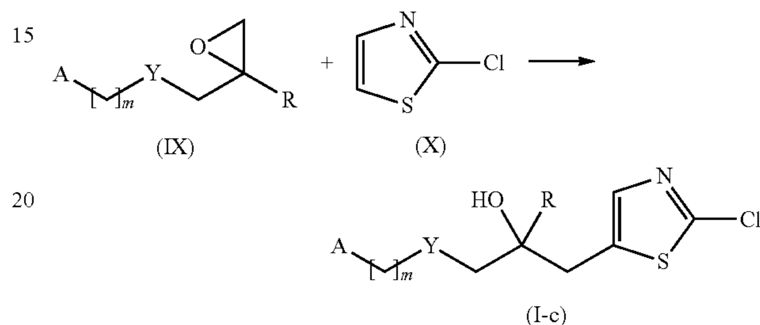
Scheme 4: Process D (X = S, n = 1, R 1 = chlorine)
