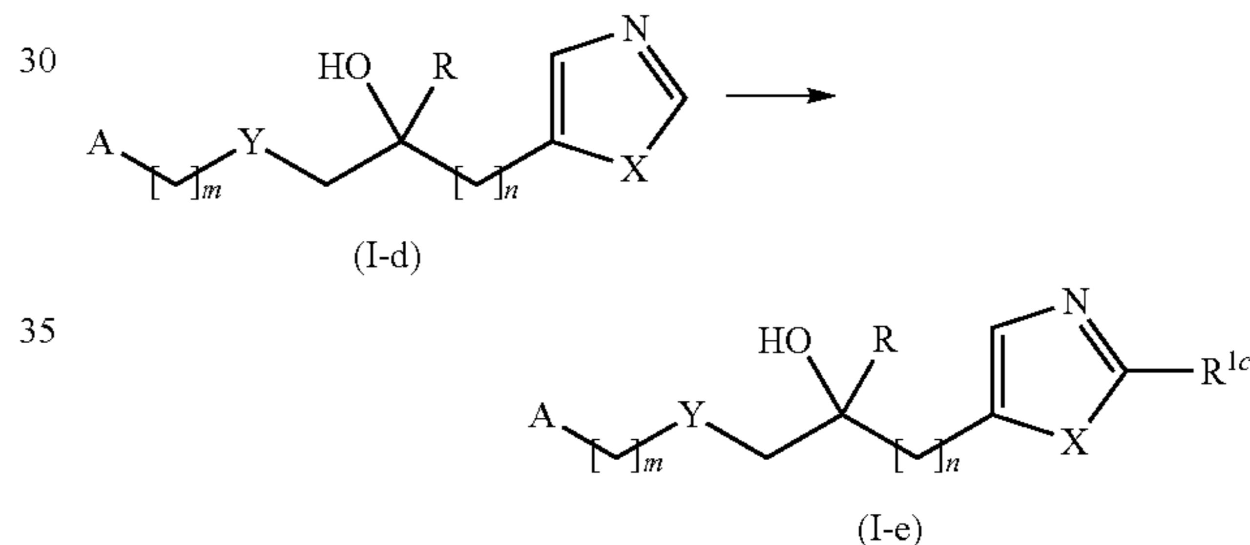
Scheme 5: Process E
