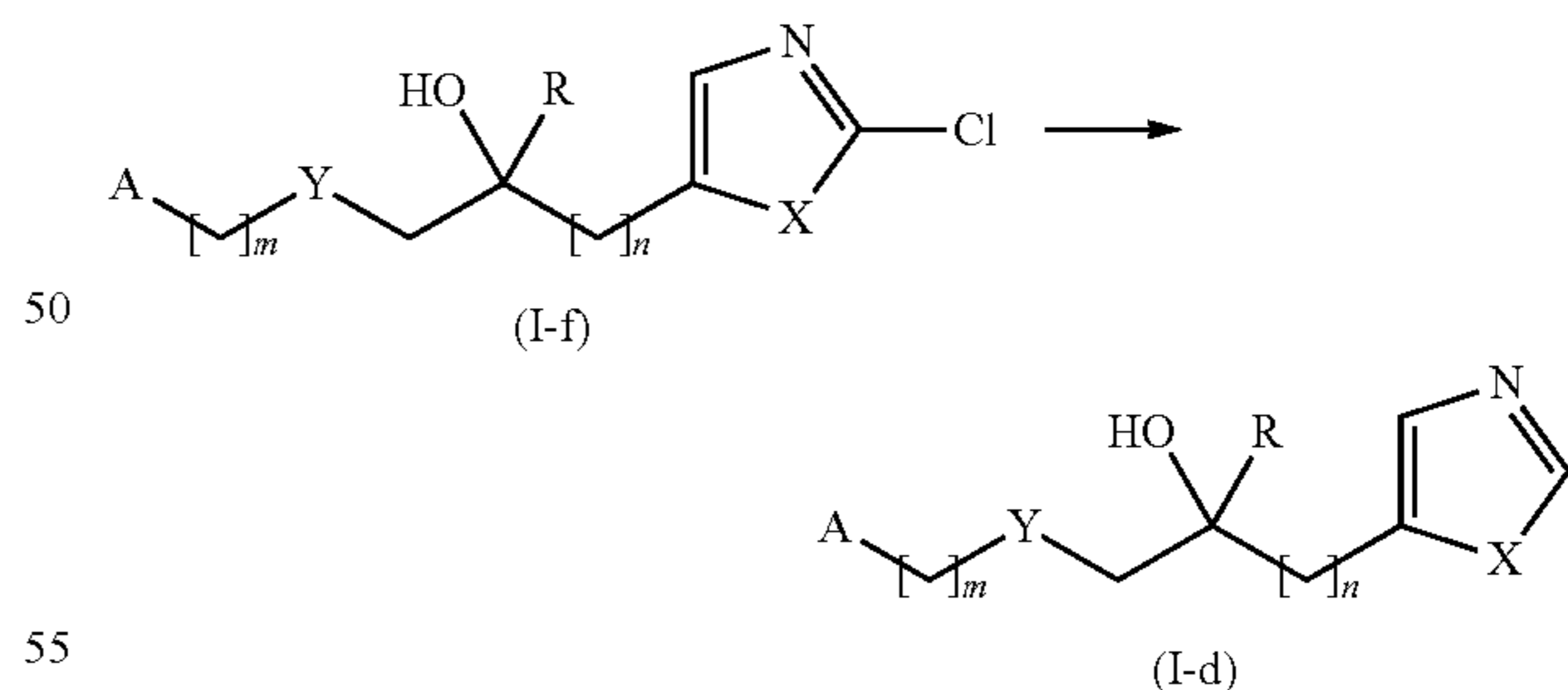
Scheme 6: Process F
