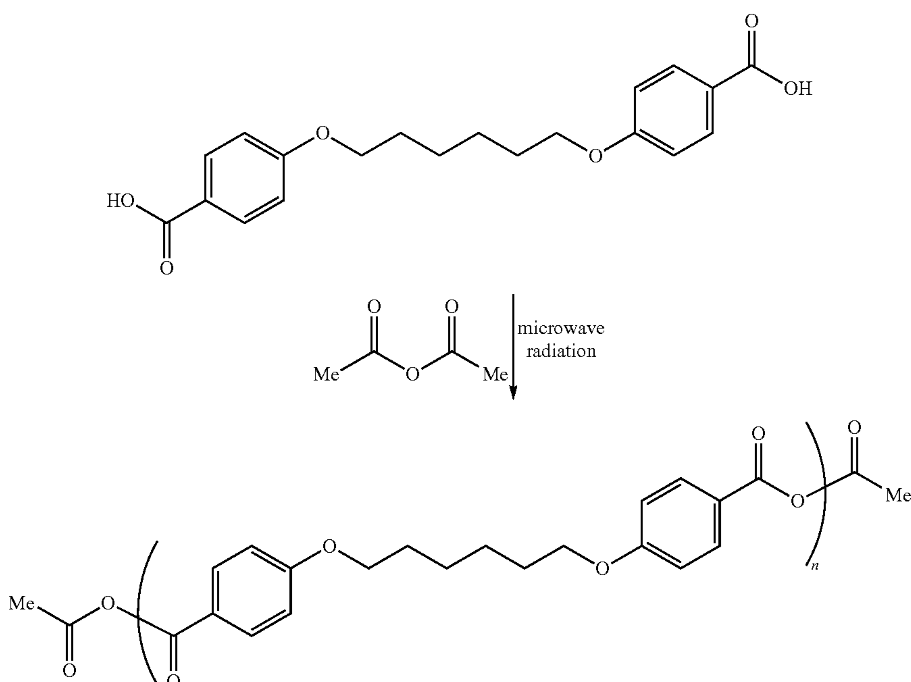
Scheme 3. Prepolymer Preparation.
