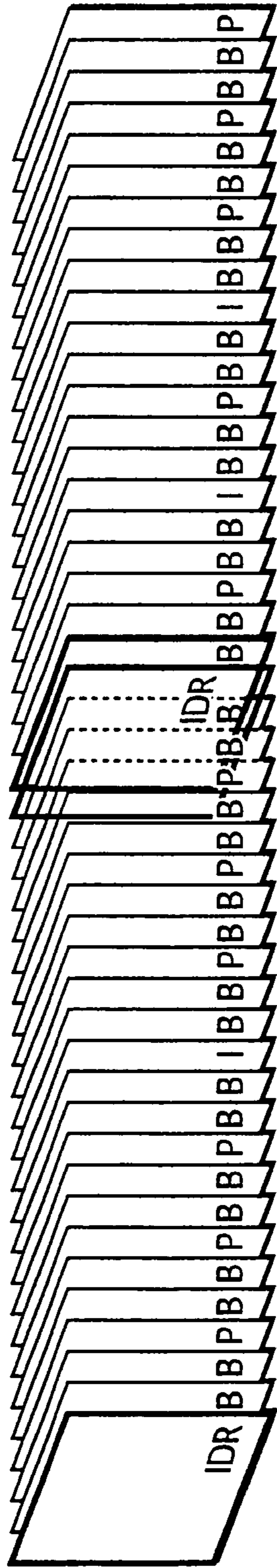
FIG. 5A MPEG4-AVC Video Stream (Coding Order)
