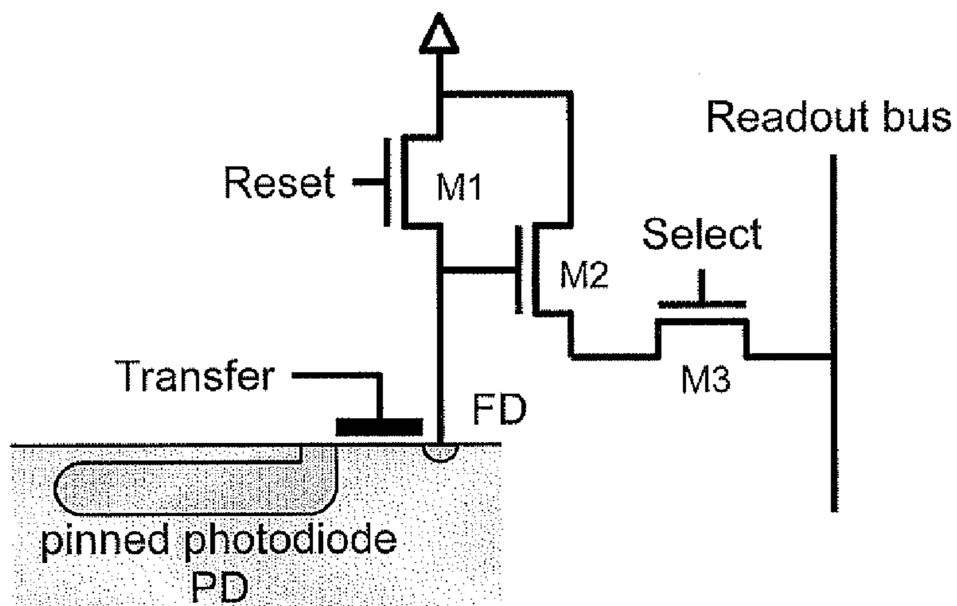
Fig. 2 (prior art)
