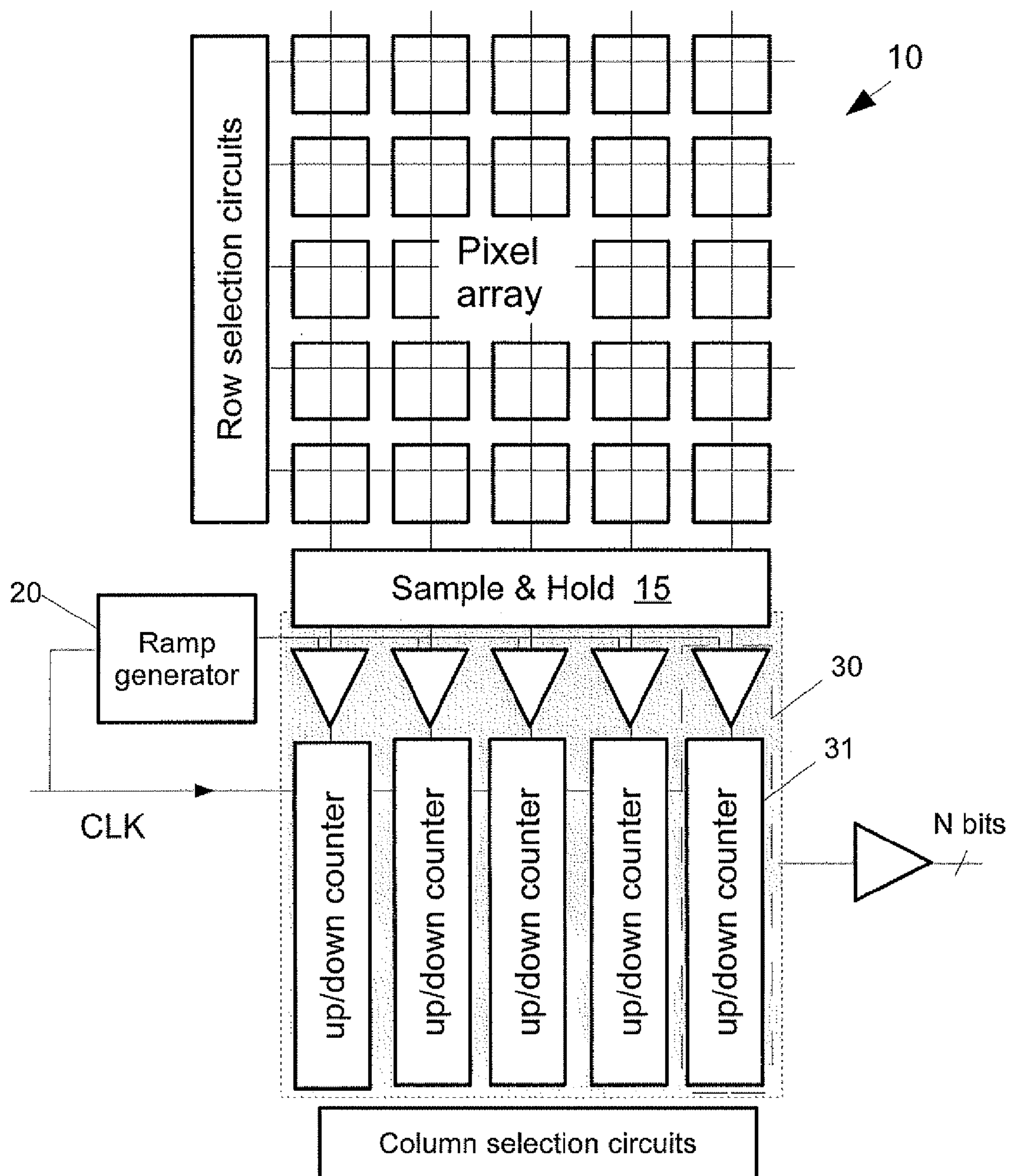
Fig. 4 (prior art)
