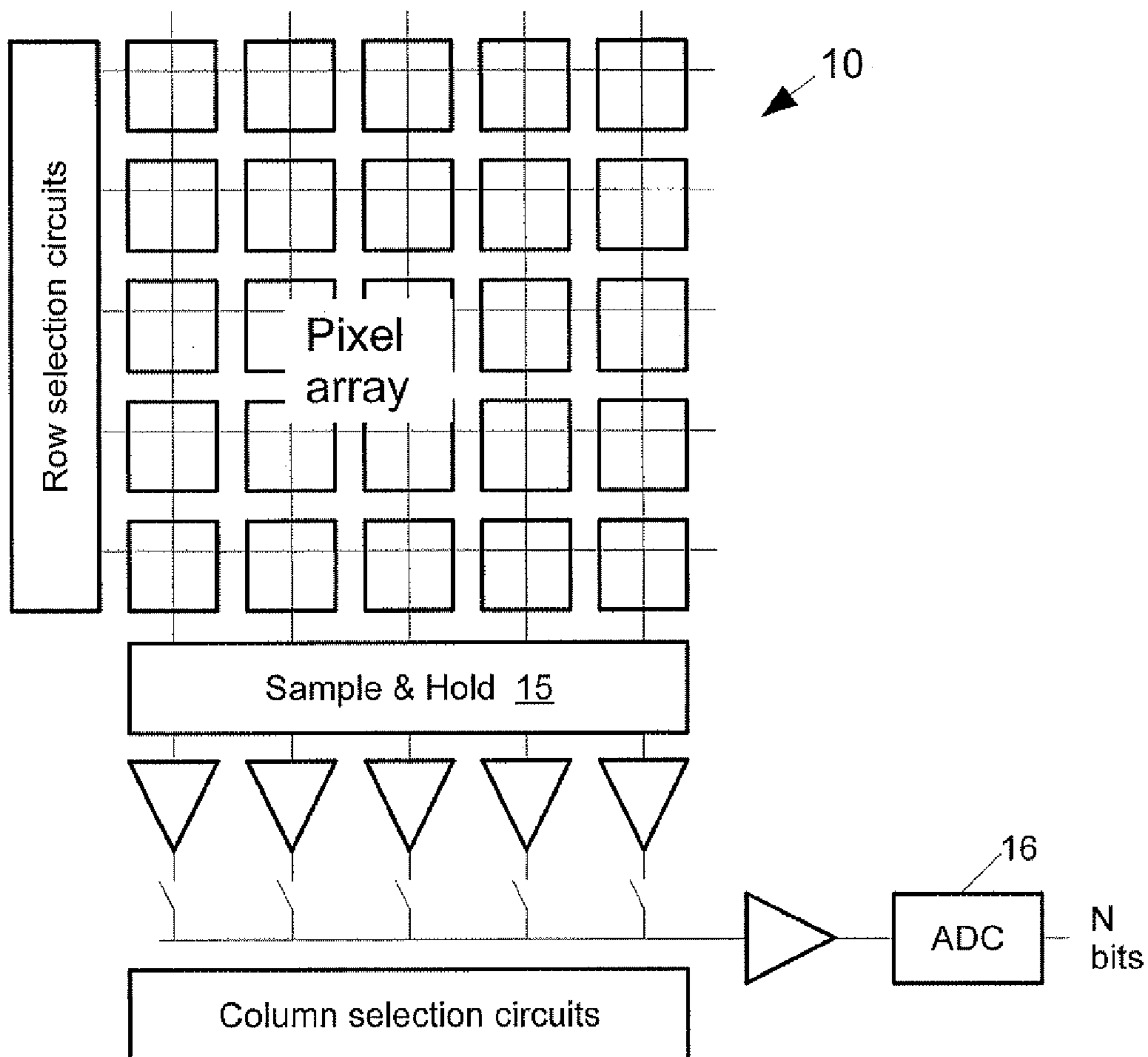
Fig. 1 (prior art)
