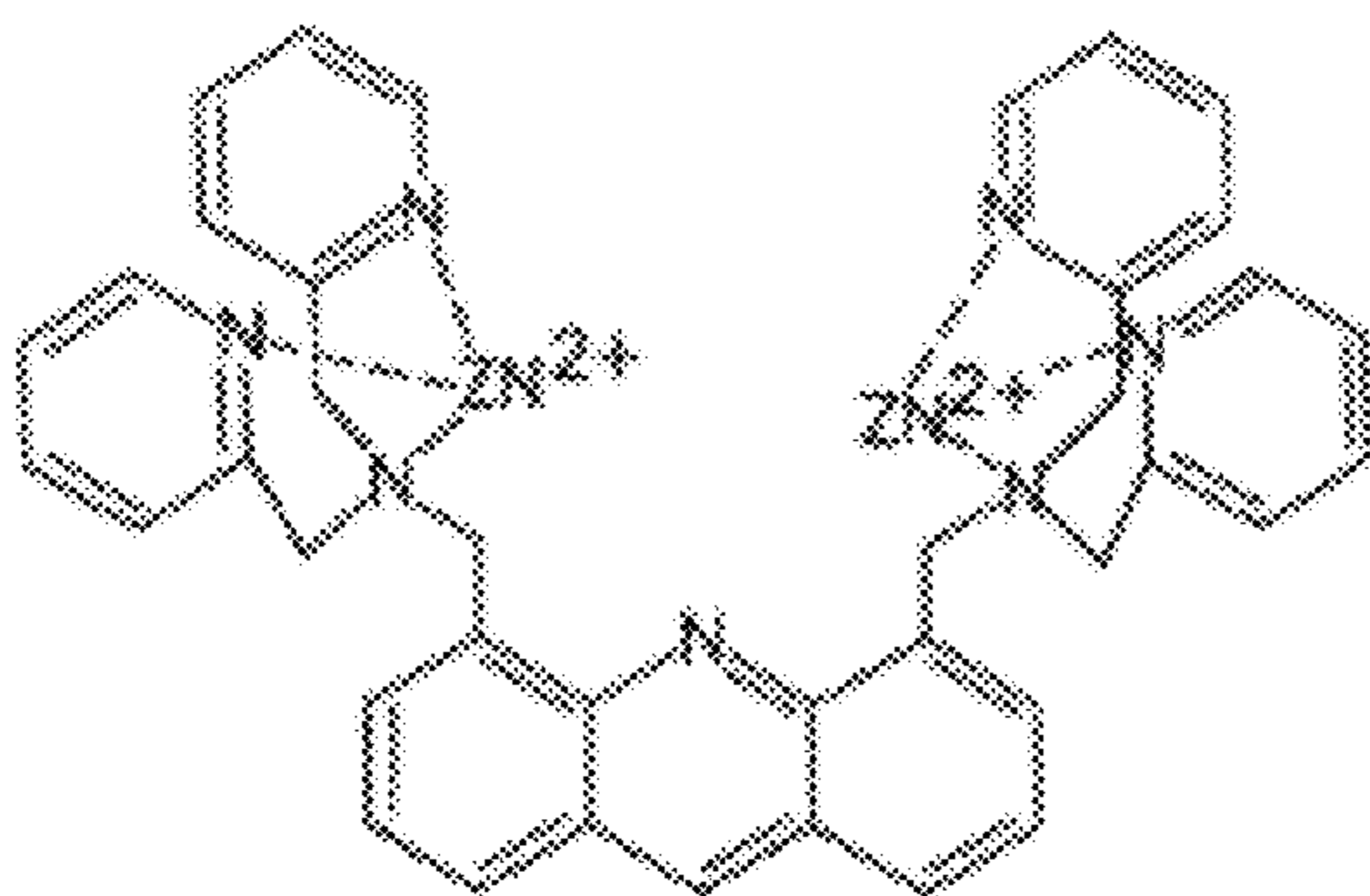
Compound 3
