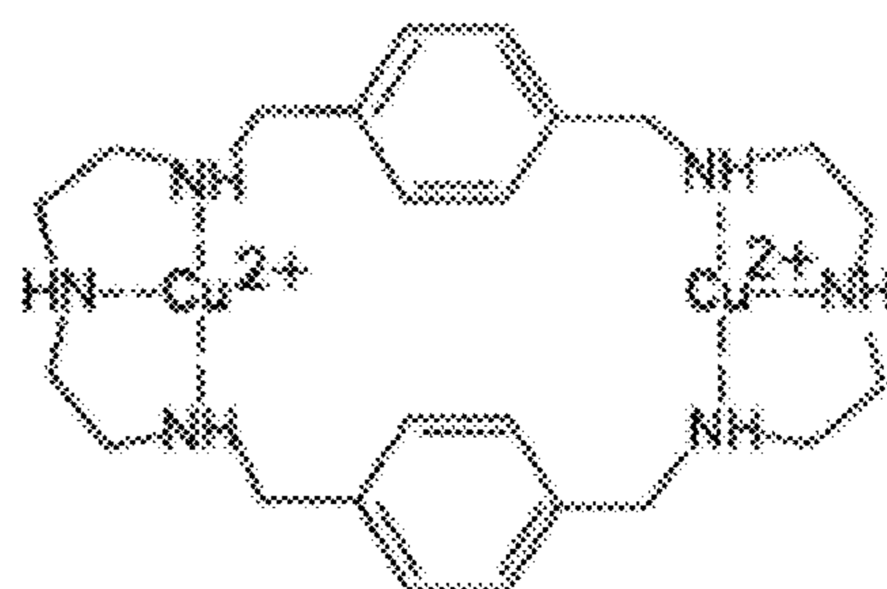
Compound 4
