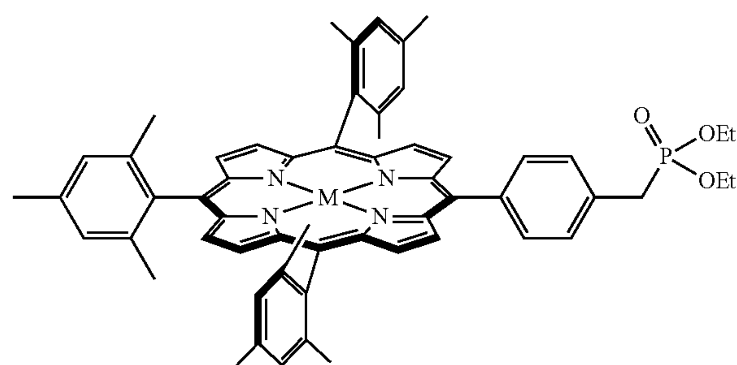
Scheme 10
