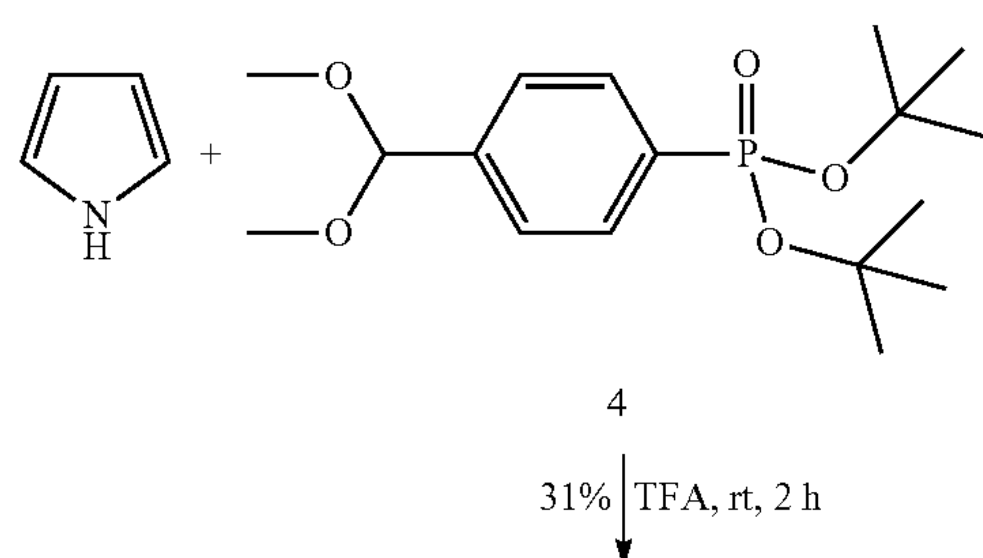
Scheme 4
