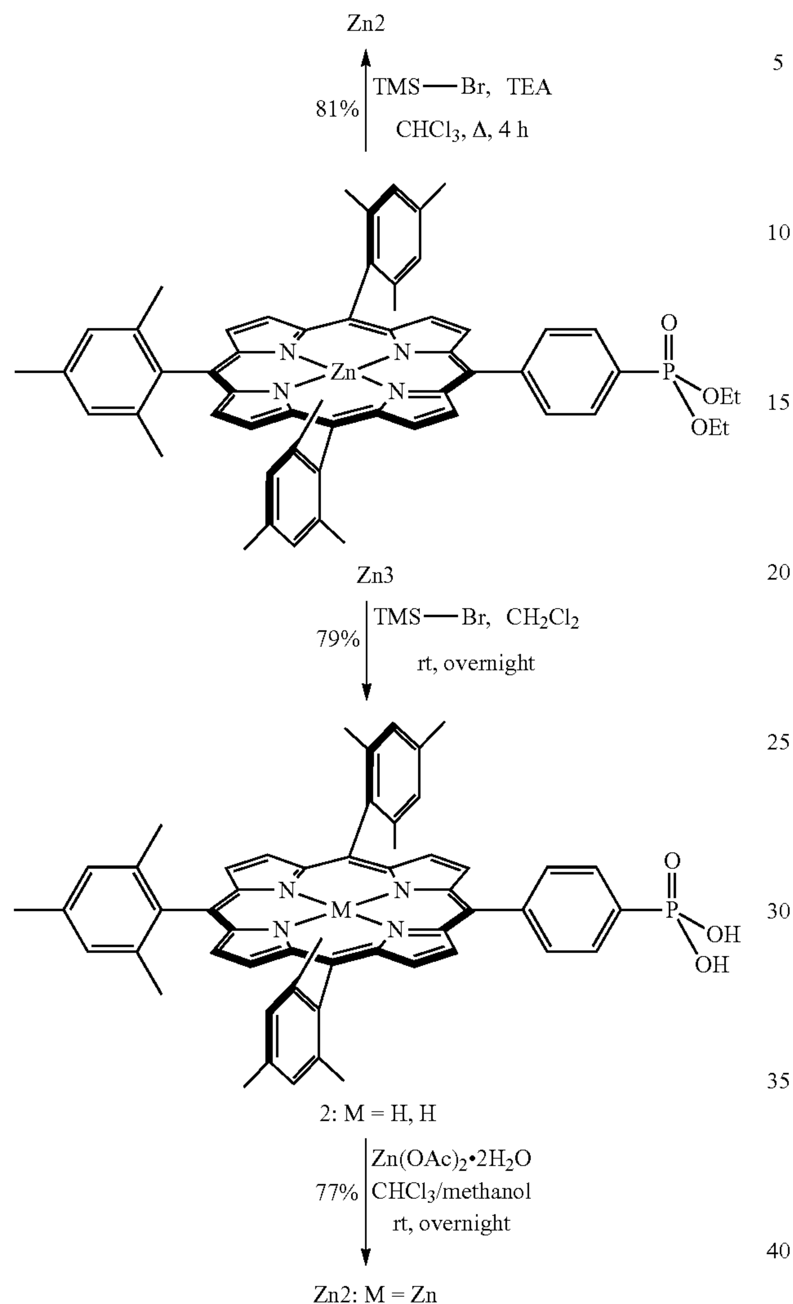
Scheme 3
