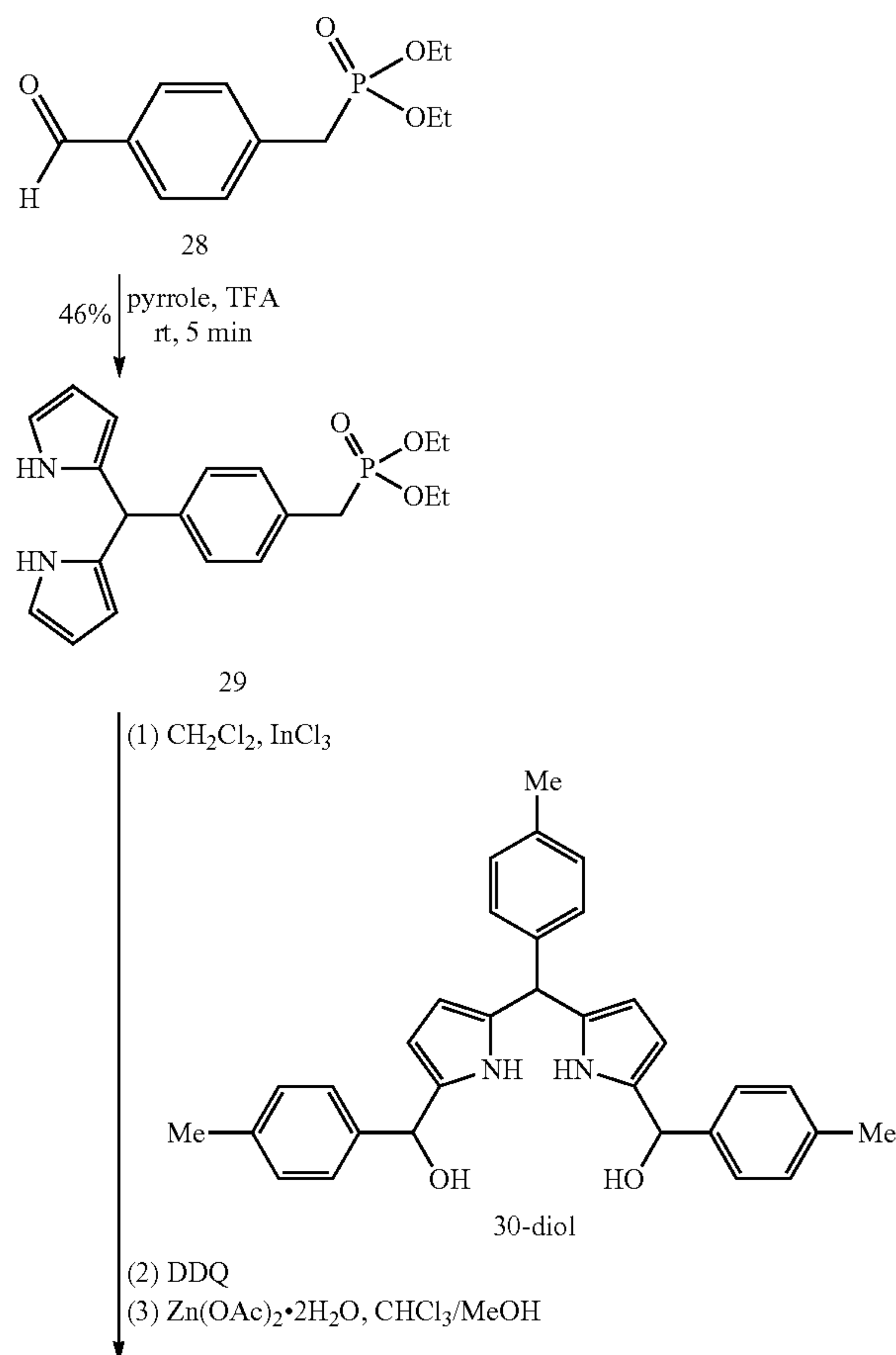
Scheme 12
