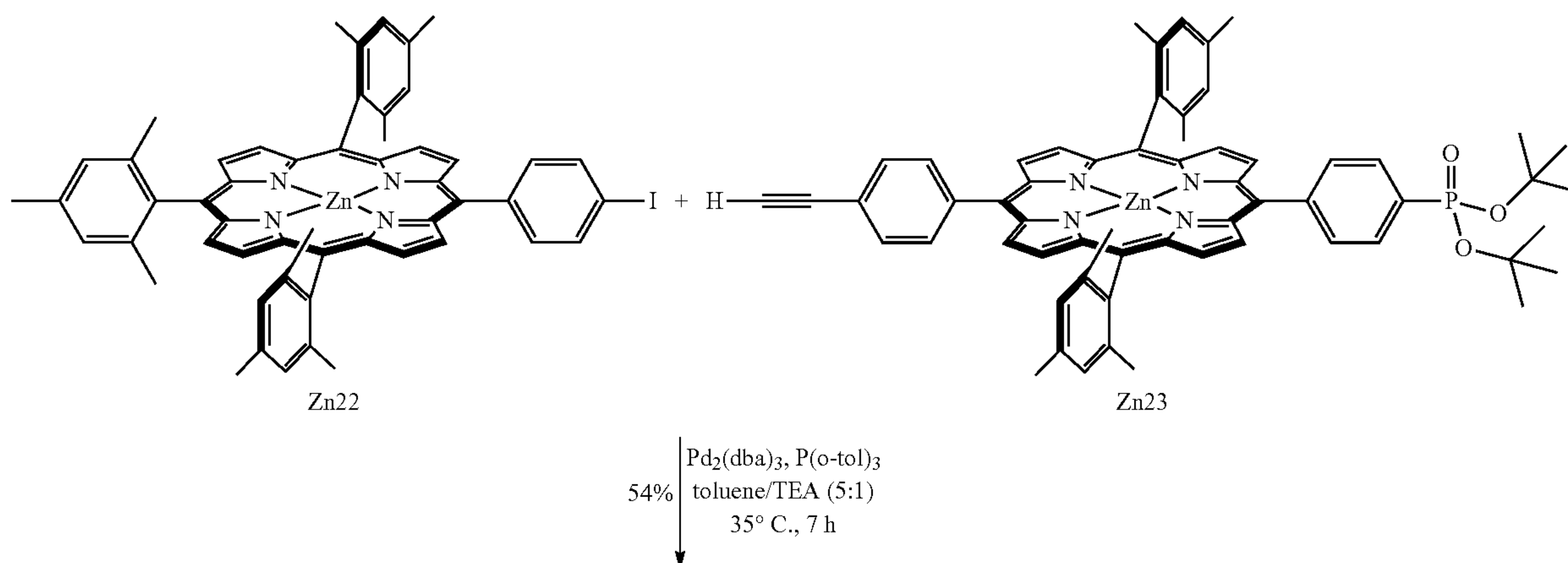
Scheme 9
