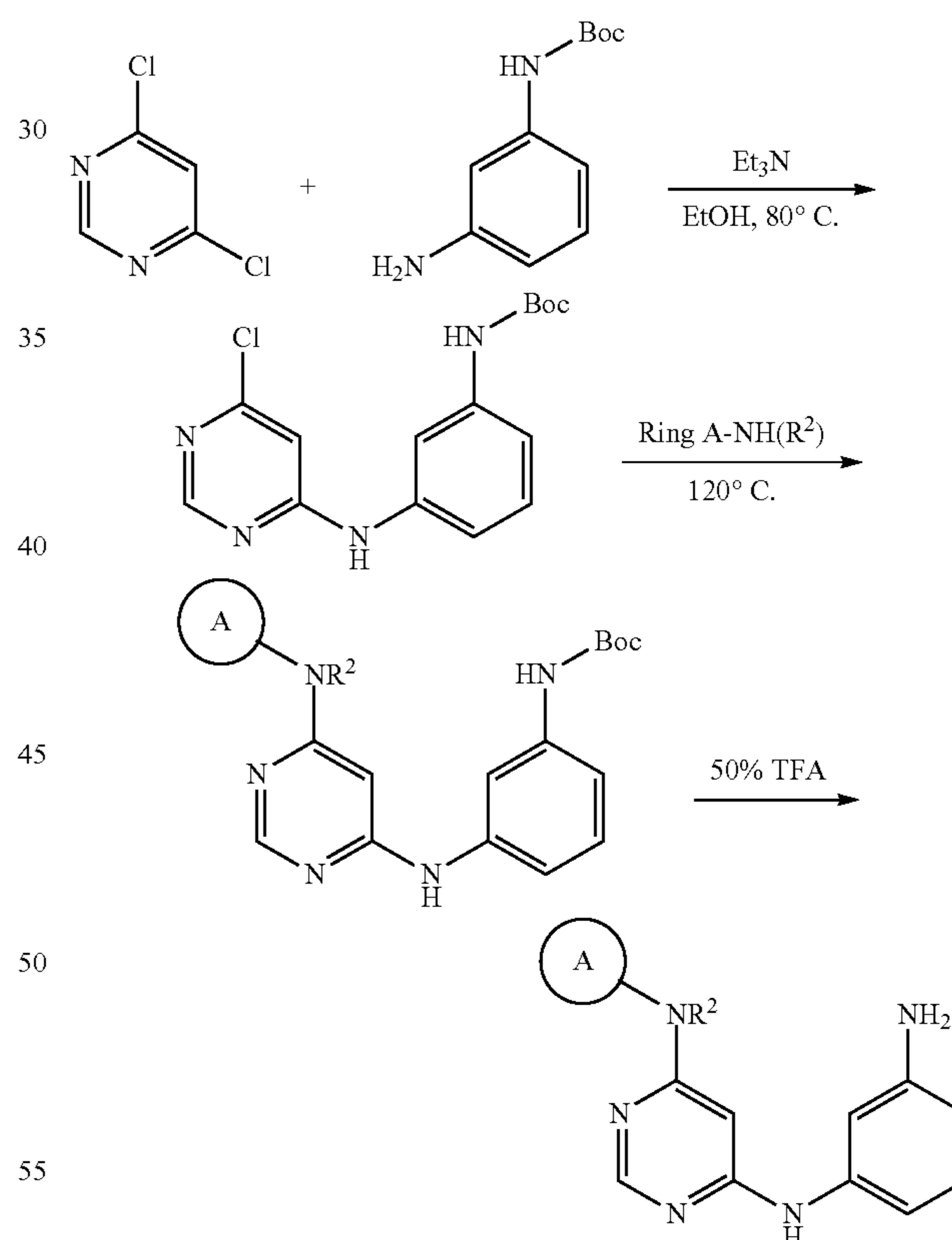
SCHEME 2a Sequence A for Synthesis of 3-(6-mono- or disubstituted-amino)pyrimidin-4-ylamino)-phenylamines
