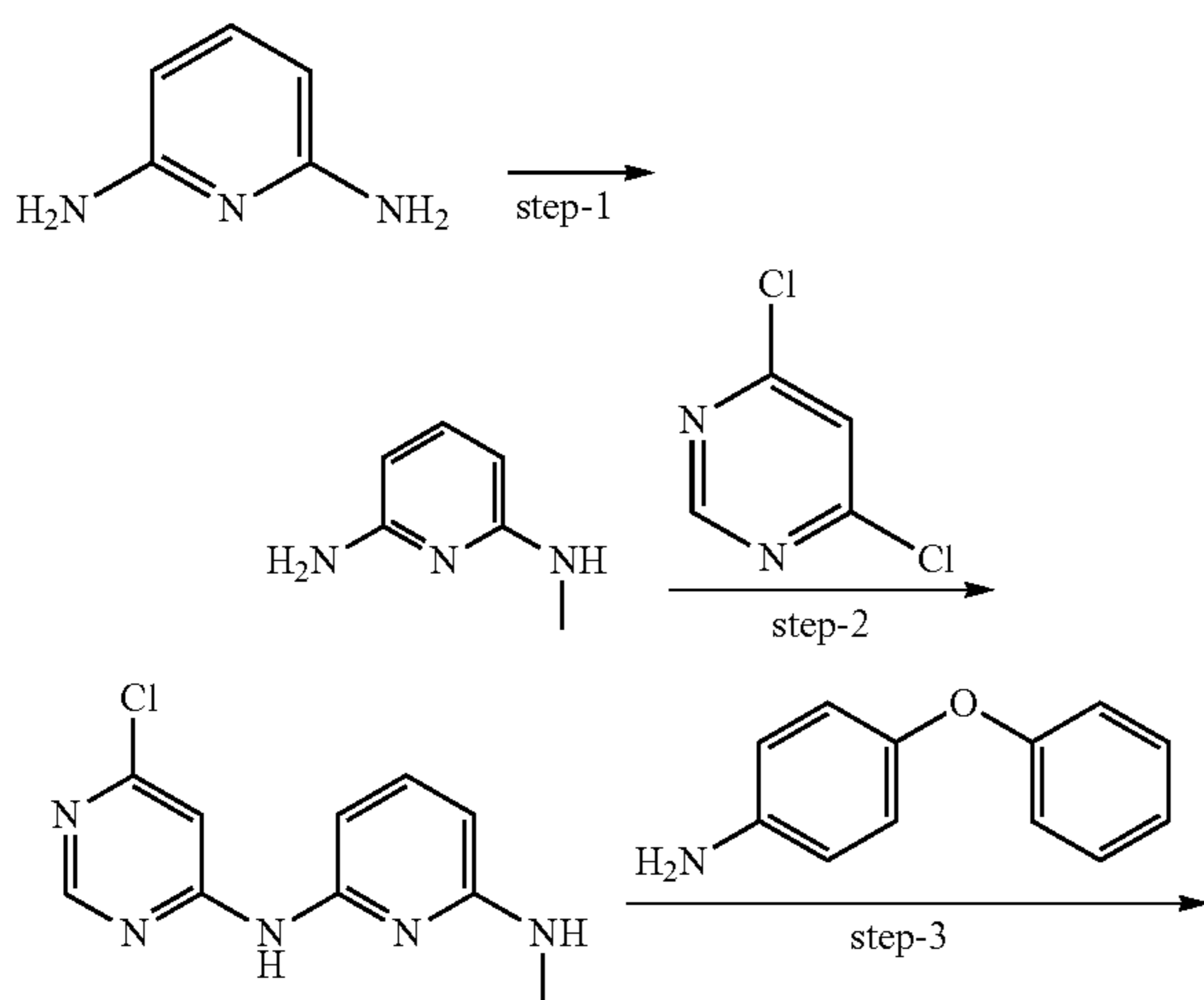
SCHEME 21a
