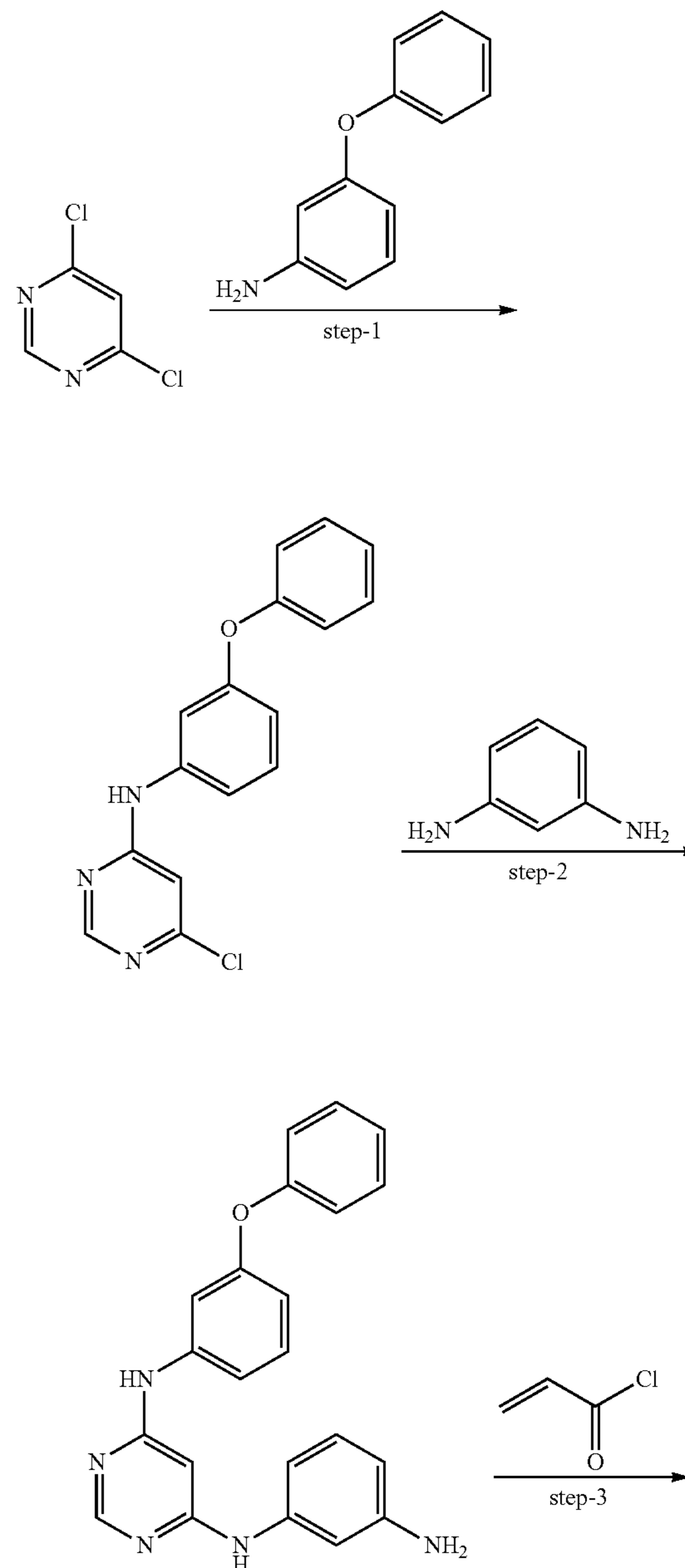
SCHEME 18a
