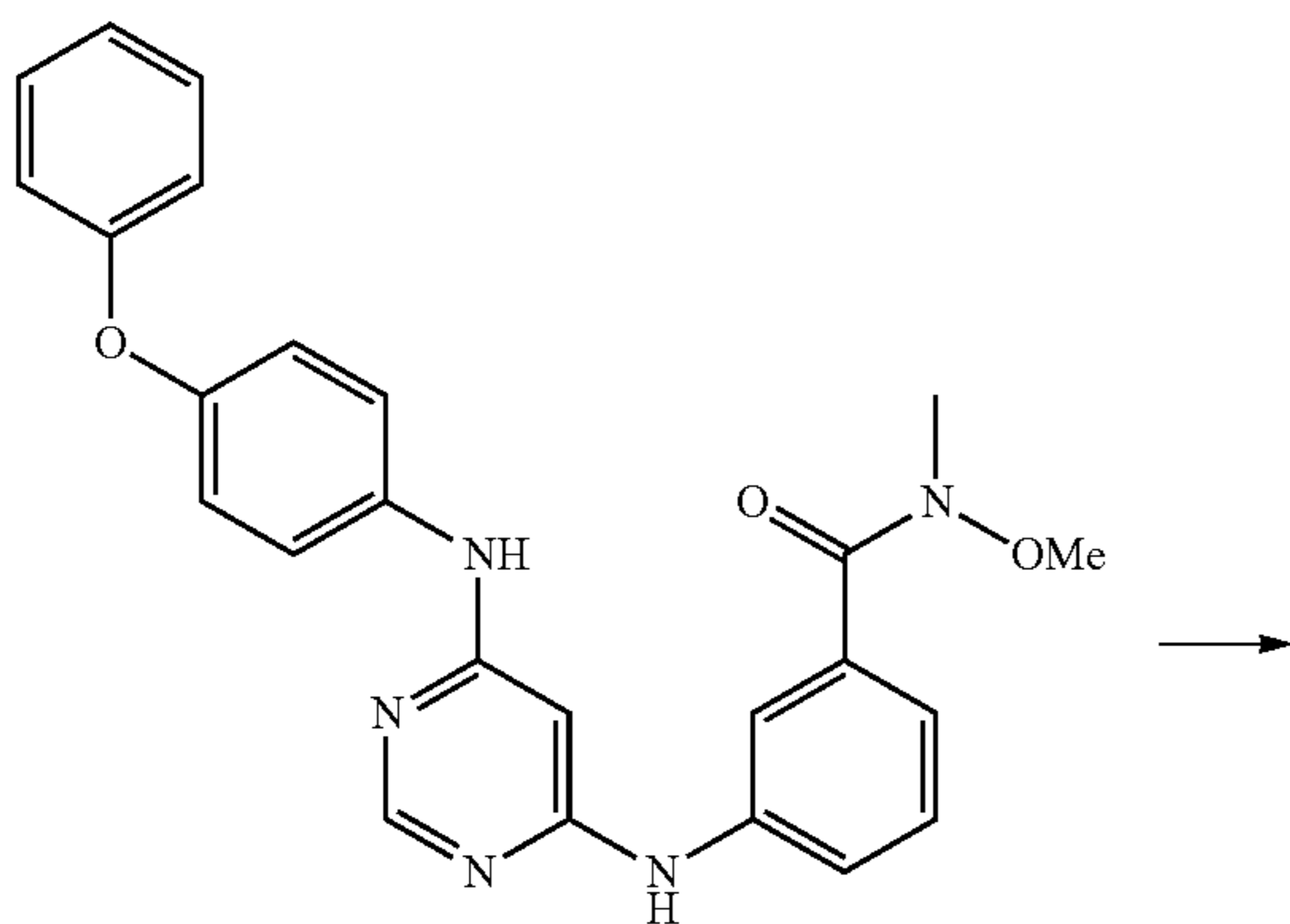
Scheme 28a
