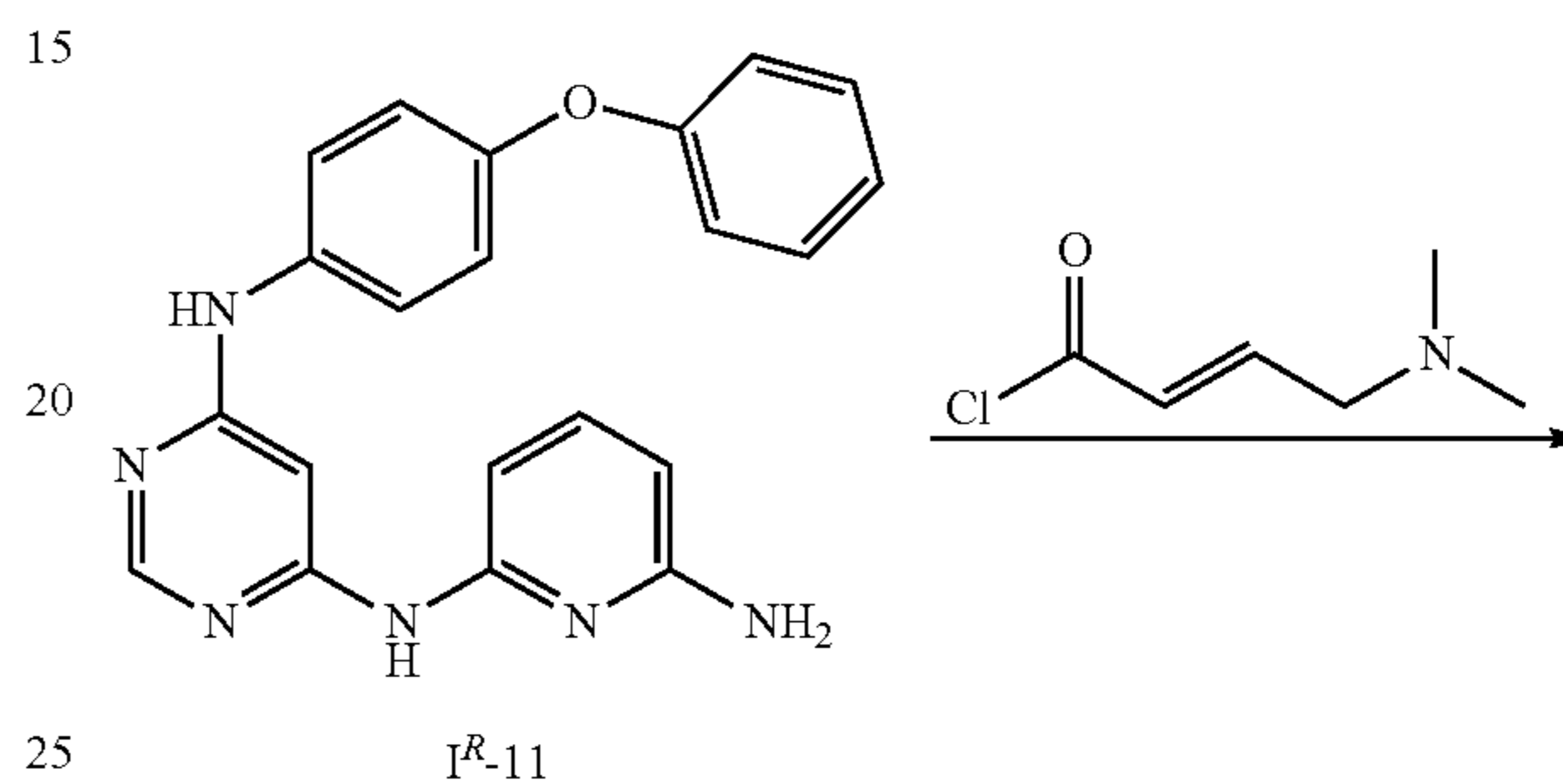
SCHEME 16a
