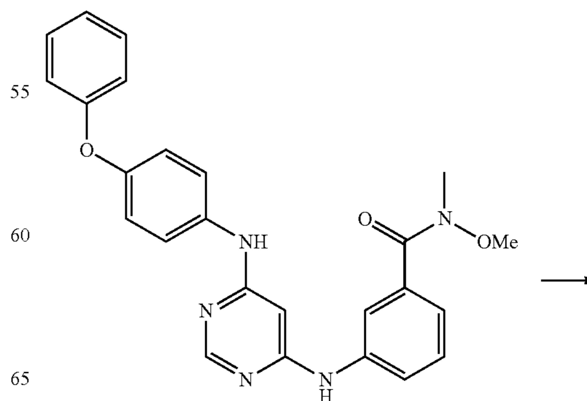
Scheme 29a
