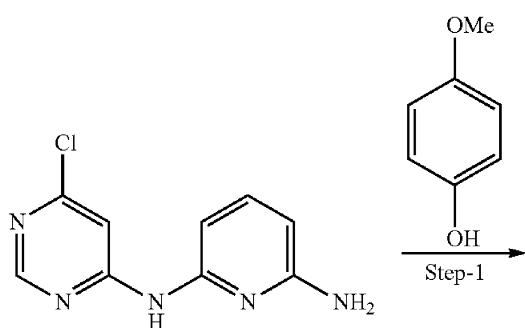
Scheme 32a
