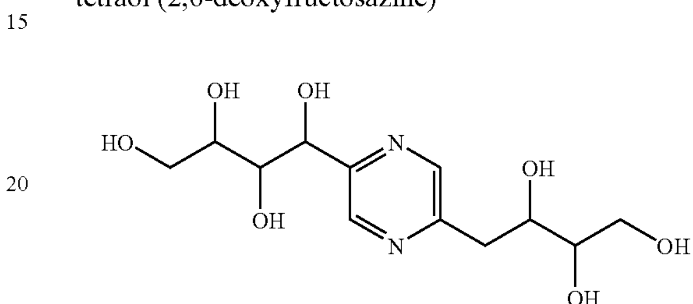
1-[6-(2,3,4-trihydroxybutyl)-pyrazin-2-yl]-butane-1,2,3,4-tetraol (2,6-deoxyfructosazine)
