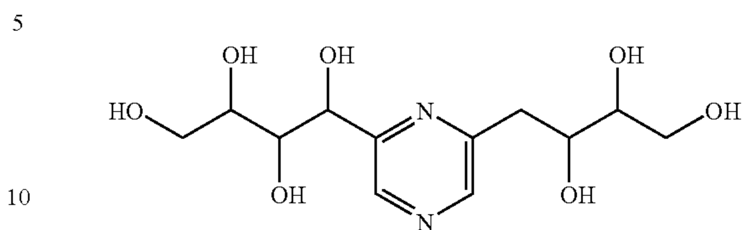
1-[6-(2,3,4-trihydroxybutyl)-pyrazin-2-yl]-butane-1,2,3,4-tetraol (2,6-deoxyfructosazine)
