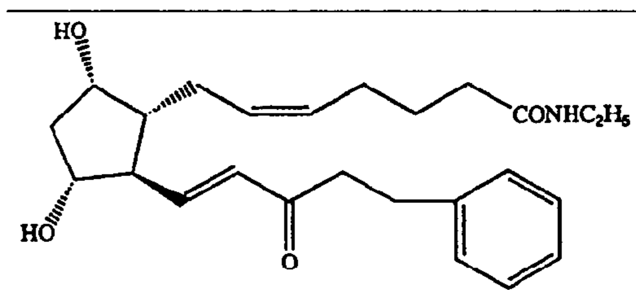
15-Keto AGN 192024 (Formerly "Impurity A")
