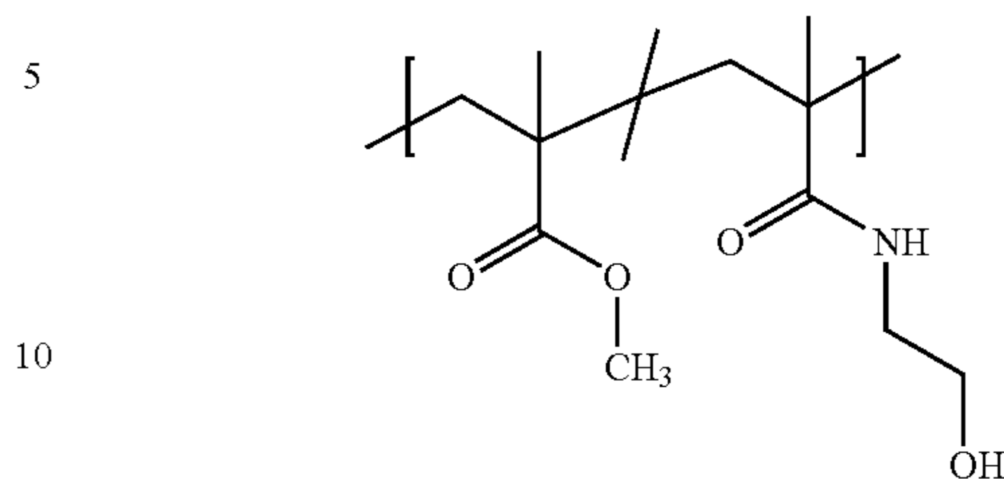
Scheme 1: Poly[(methyl methacrylate)-co-(2-hydroxyethyl methacrylamide)].
