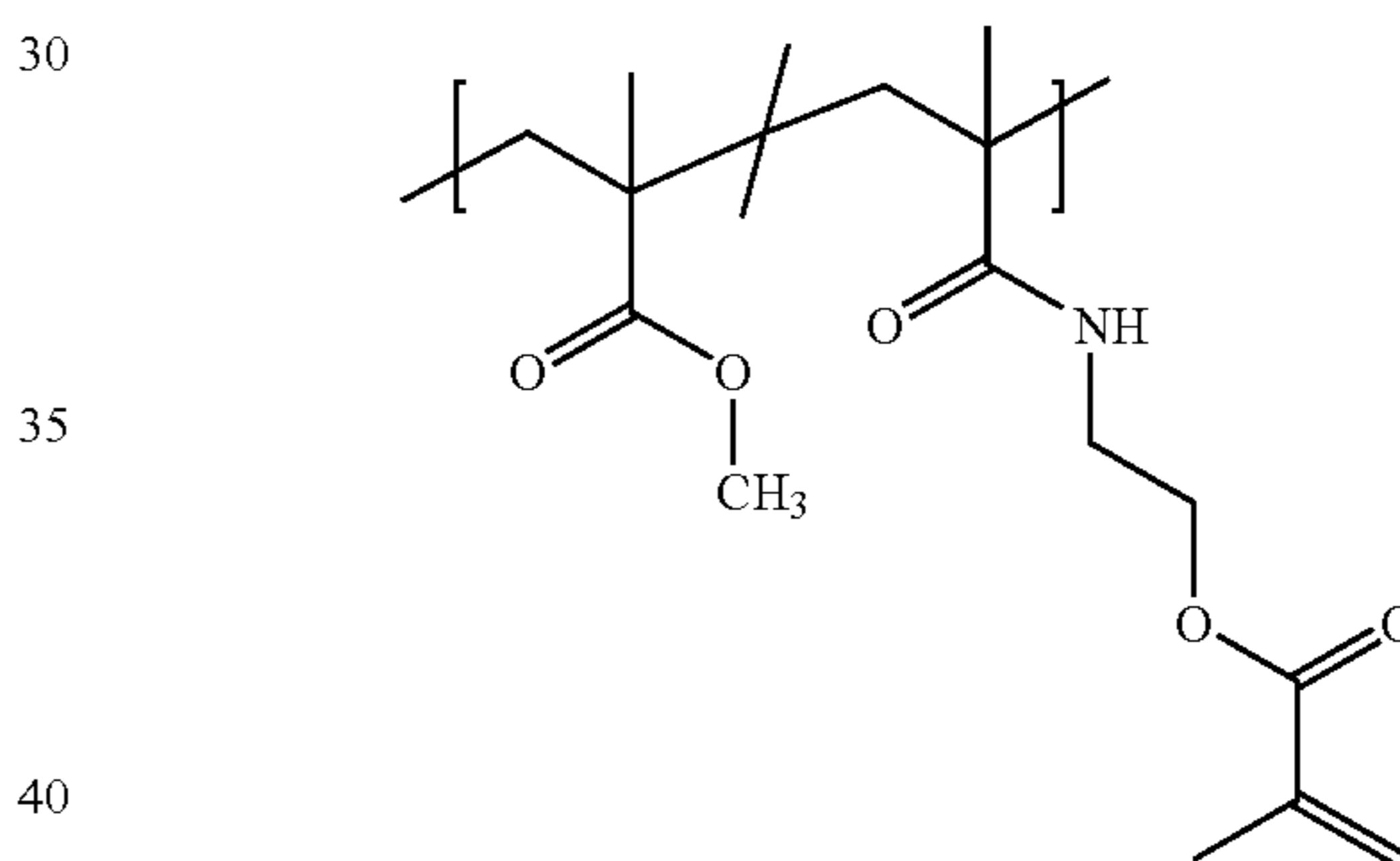
Scheme 2: Poly[(methyl methacrylate)-co-(2-[methacryloxy]ethyl methacrylamide)].
