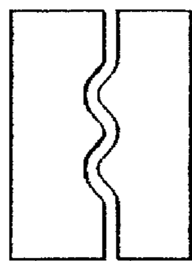
Multi-Toothed Waved
