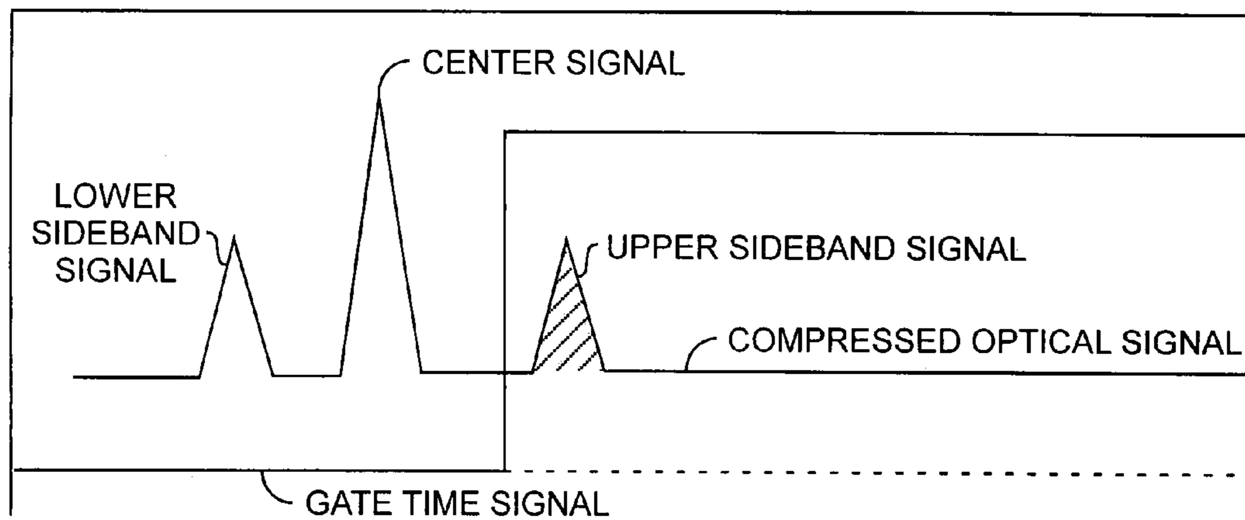
GATE TIMING
