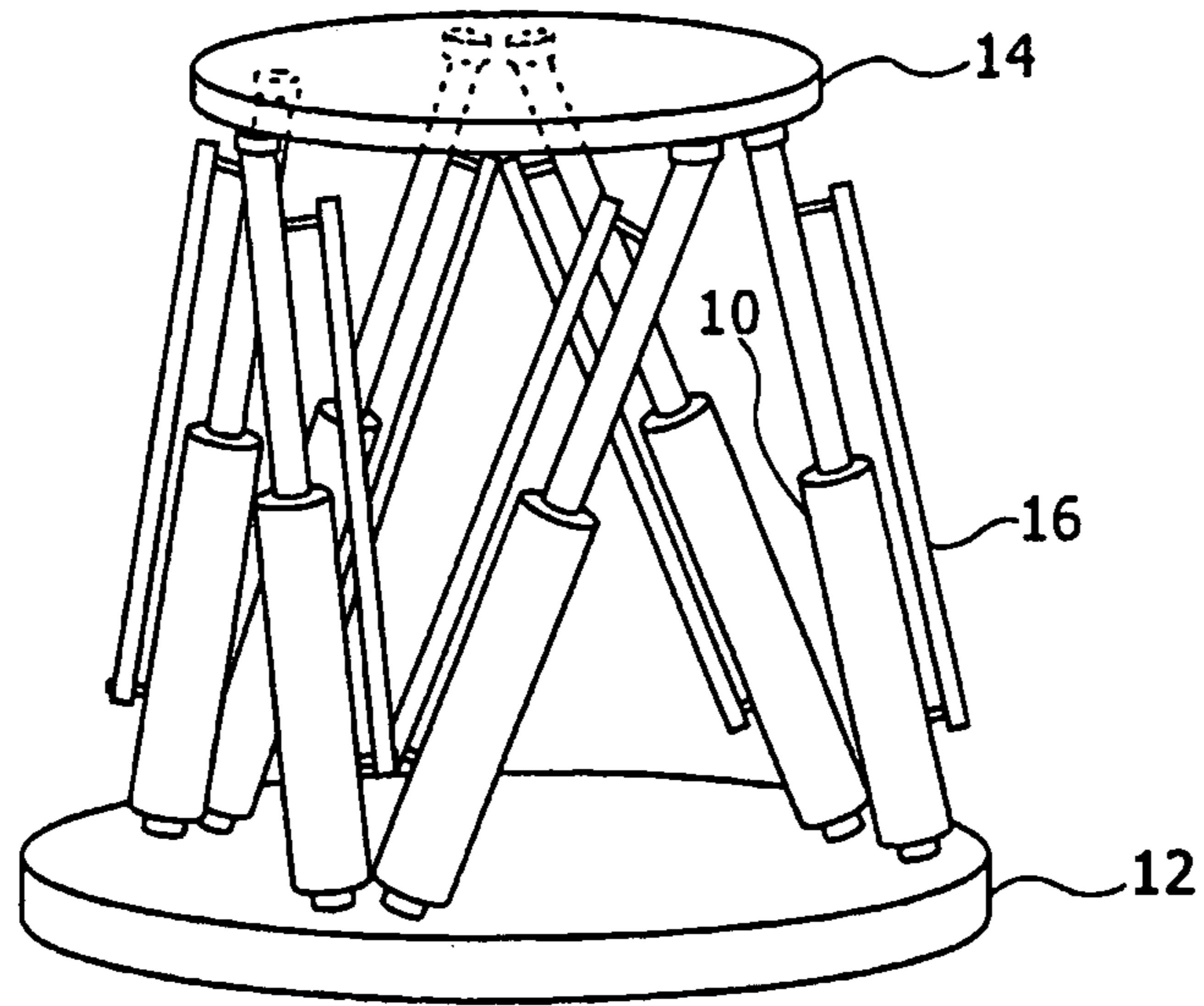
FIG. 1 (Prior Art)
