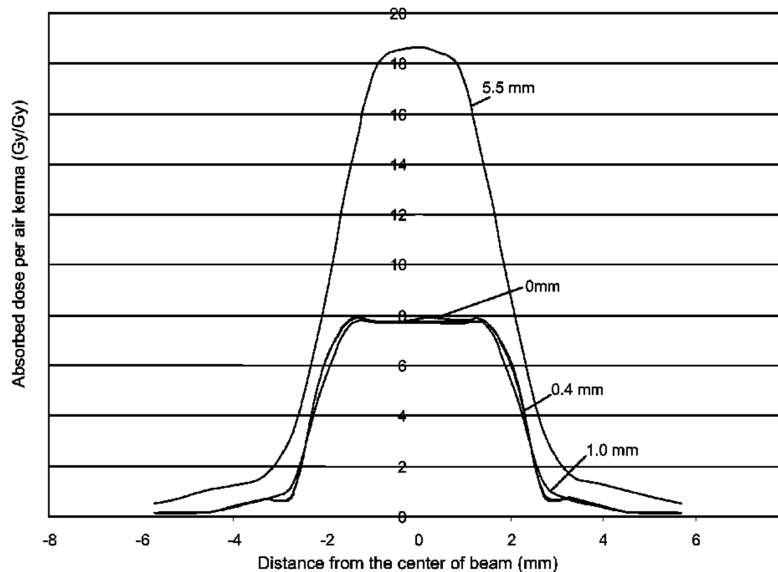
Absolute 1D dose profile (Gy/Gy) at the center of macula
