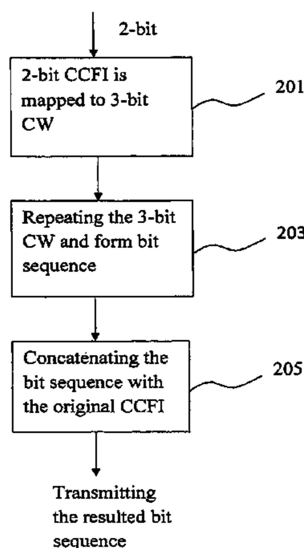
Transmission Flowchart 1
