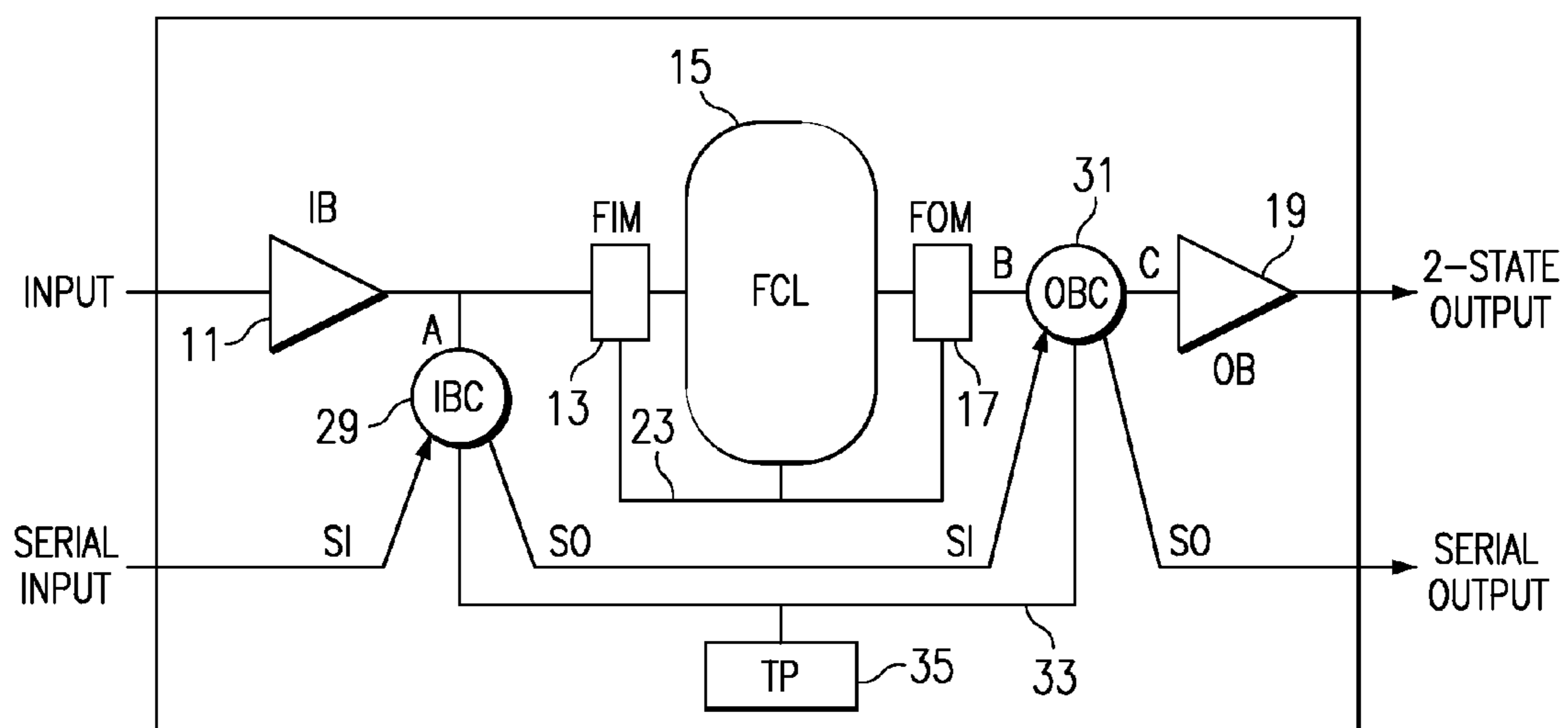
FIG. 3 (PRIOR ART)
