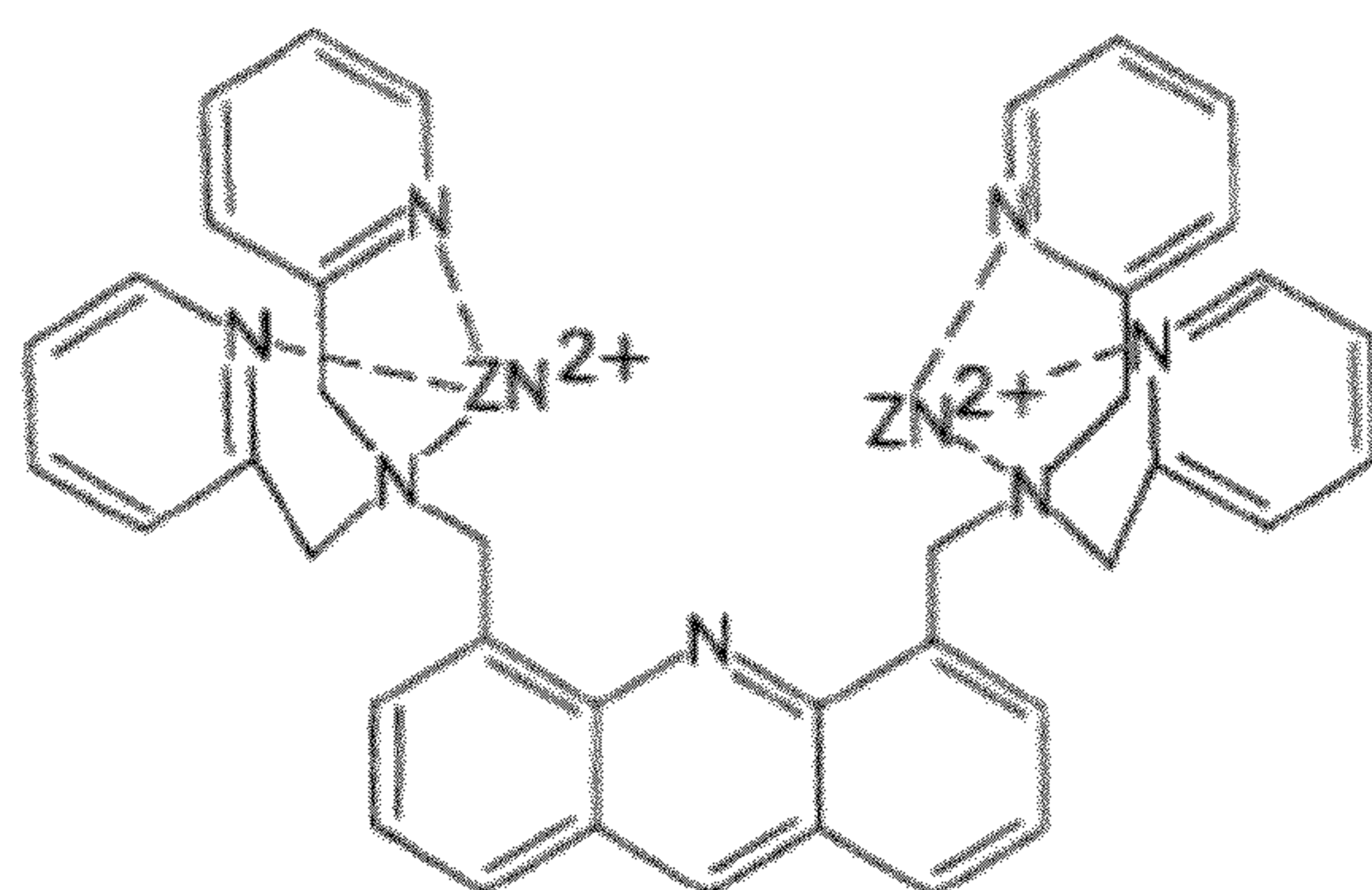
Compound 3
