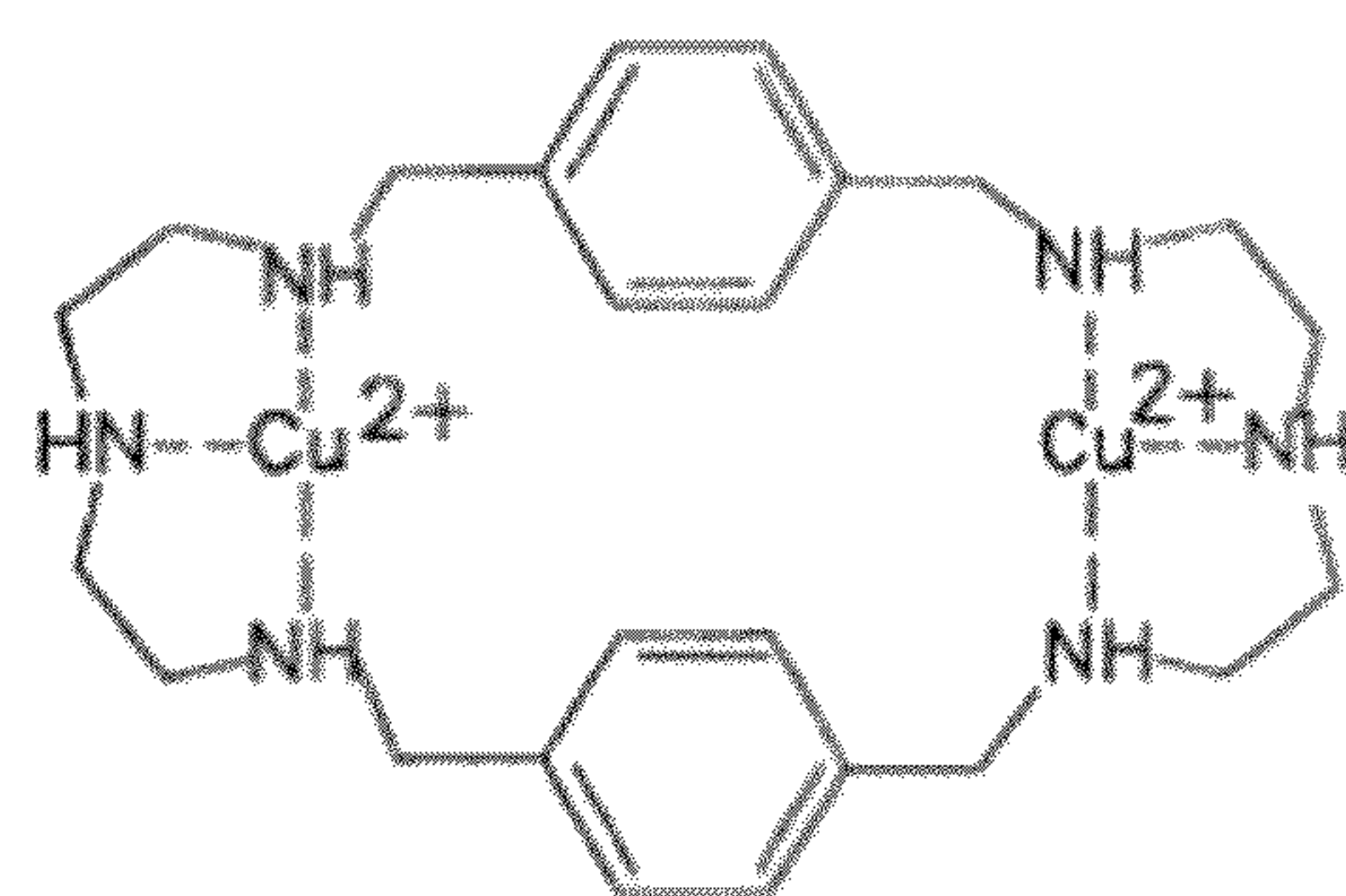
Compound 4
