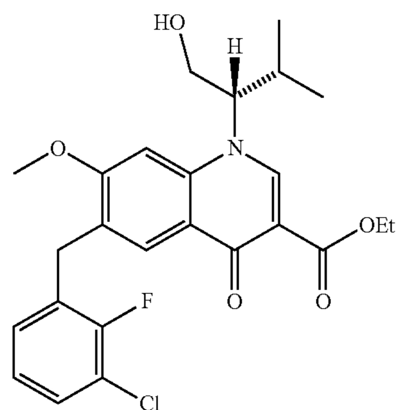
Compound 9a C_{25}H_{27}ClFNO_5 Mol. Wt.: 475.94
