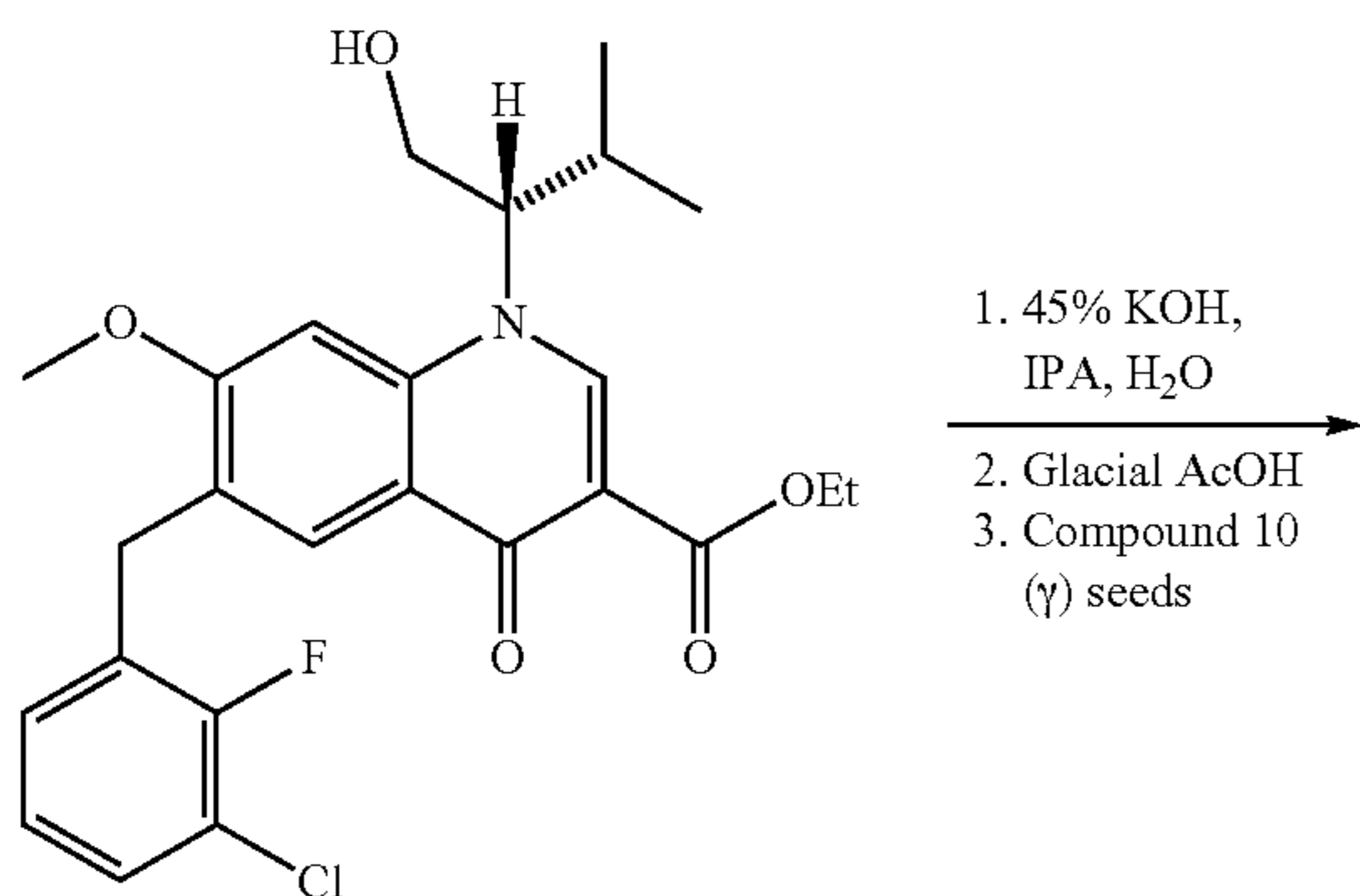
Compound 9a C 25 H 27 ClFNO 5 Mol. Wt.: 475.94
