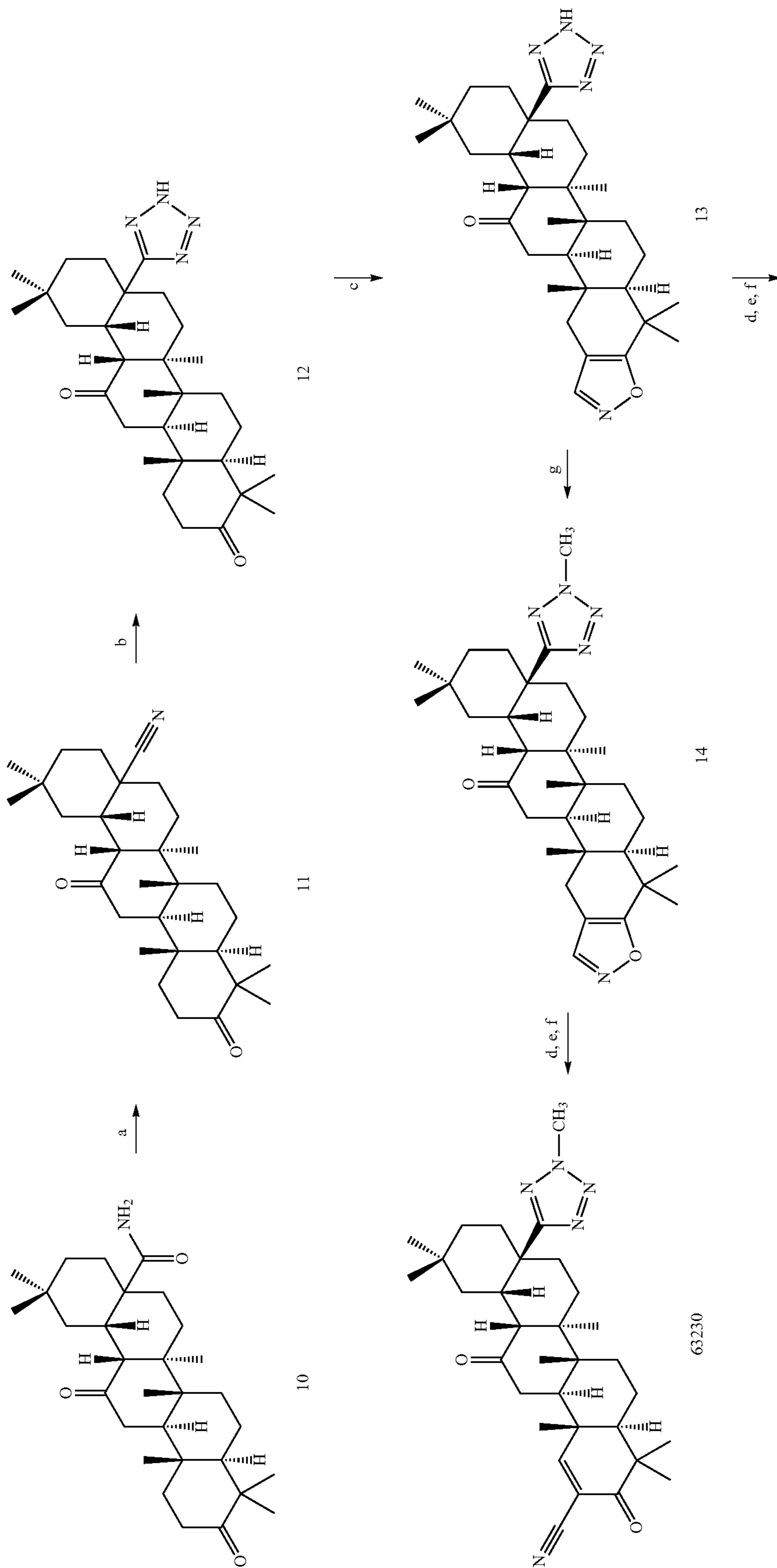
Scheme 7:
