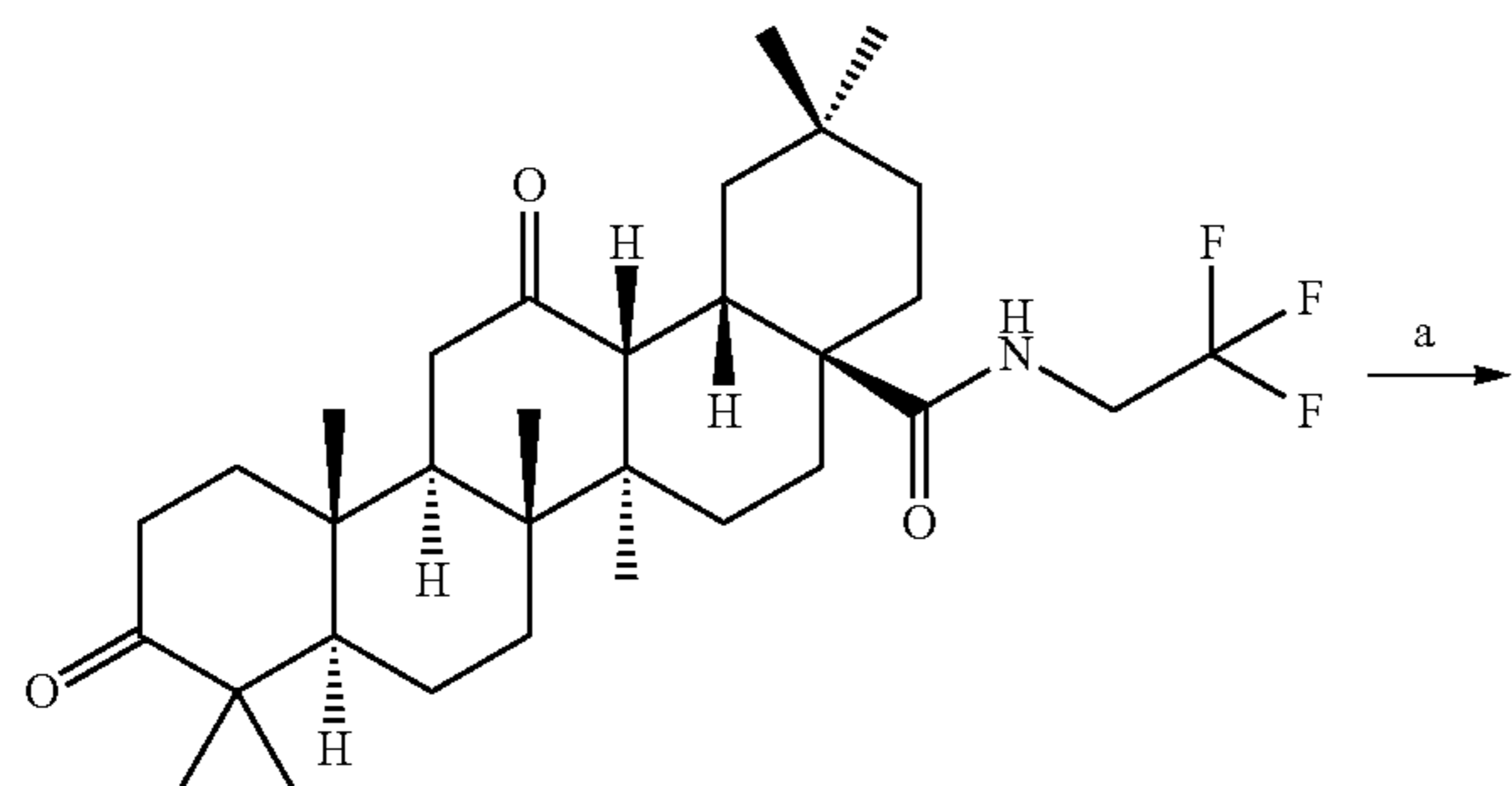
Scheme 8:
