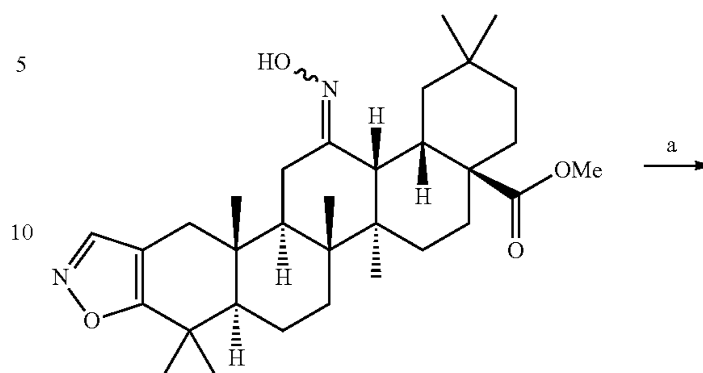
Scheme 17:
