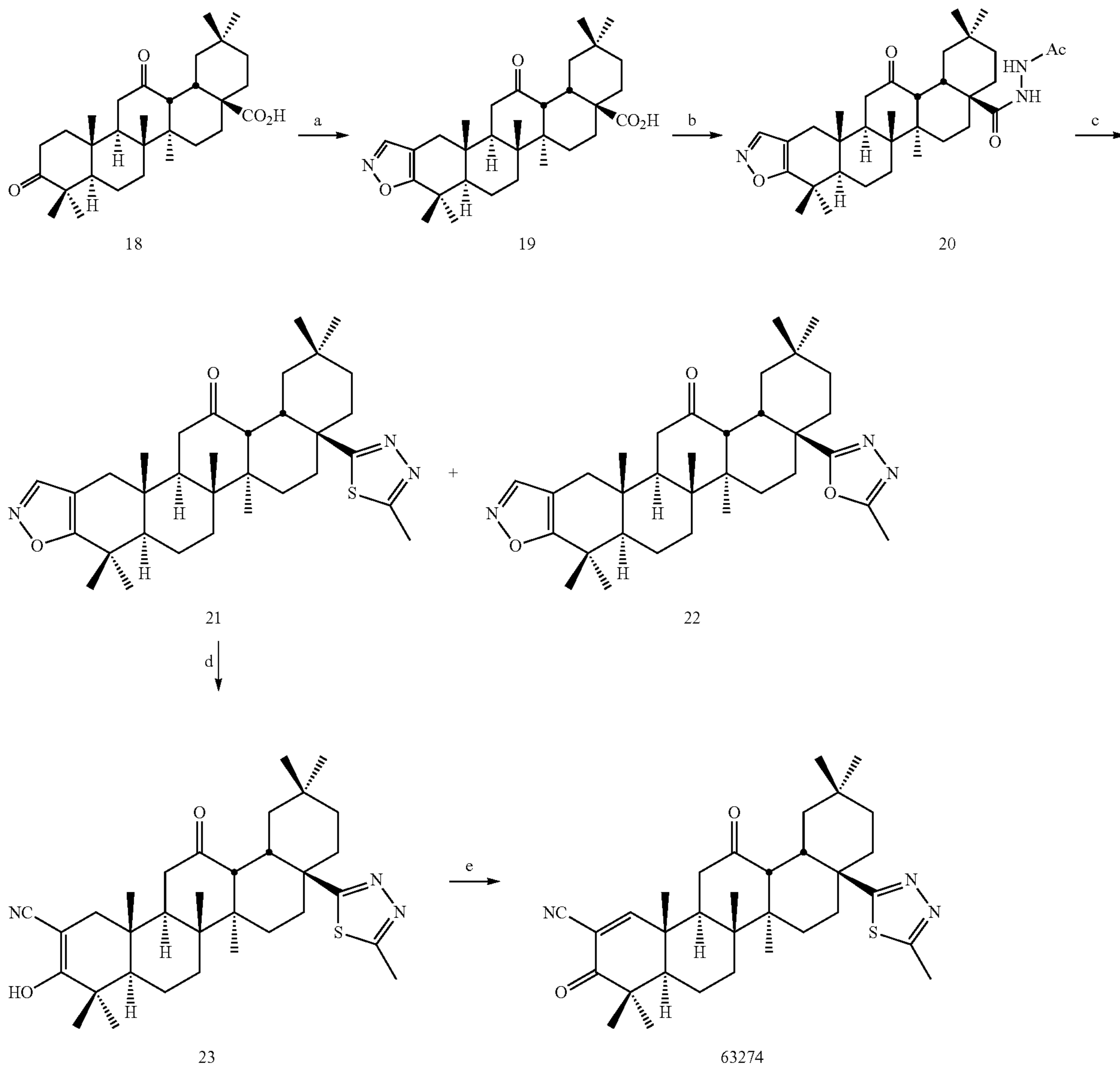
Scheme 10:
