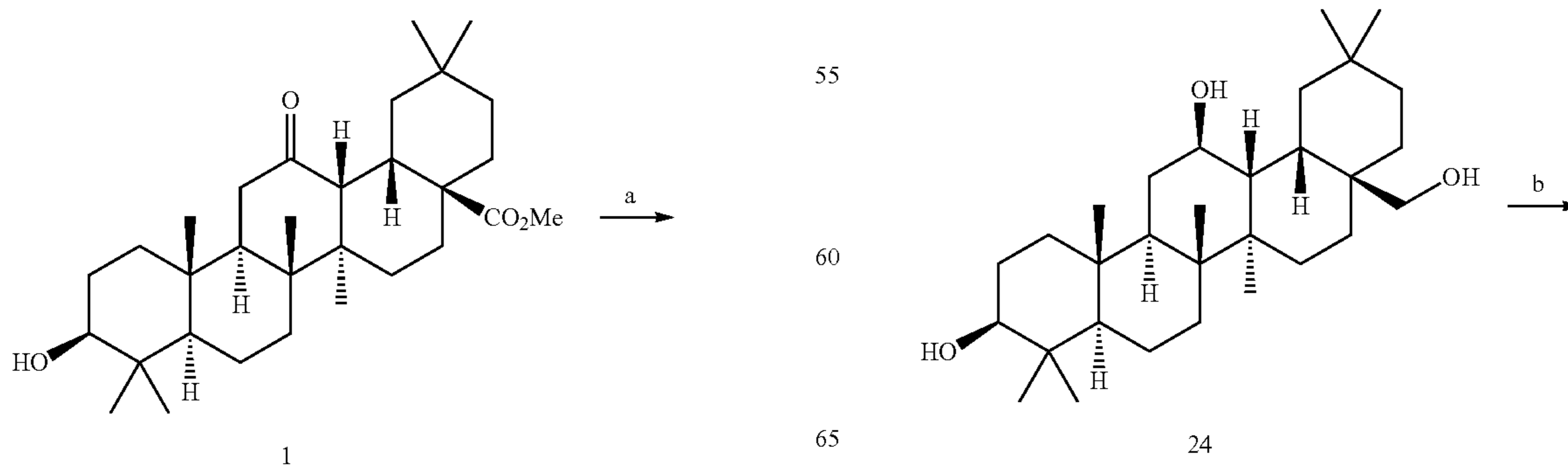
Scheme 11:
