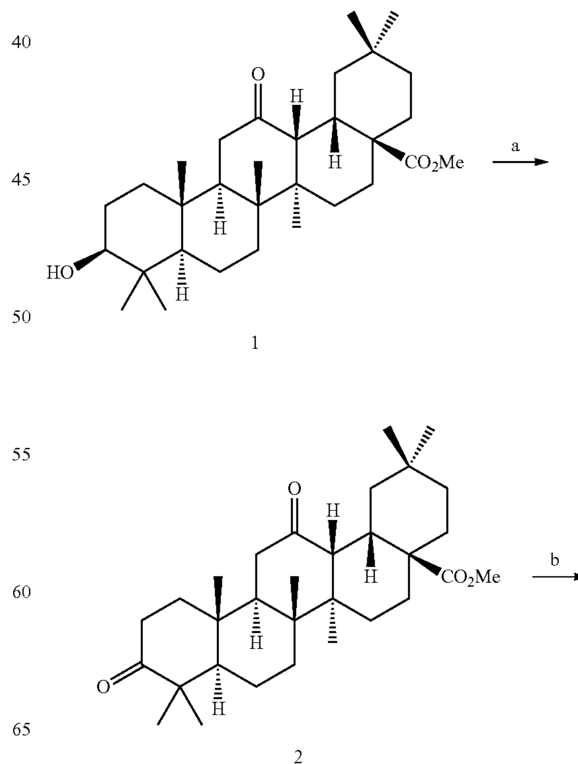
Scheme 1:
