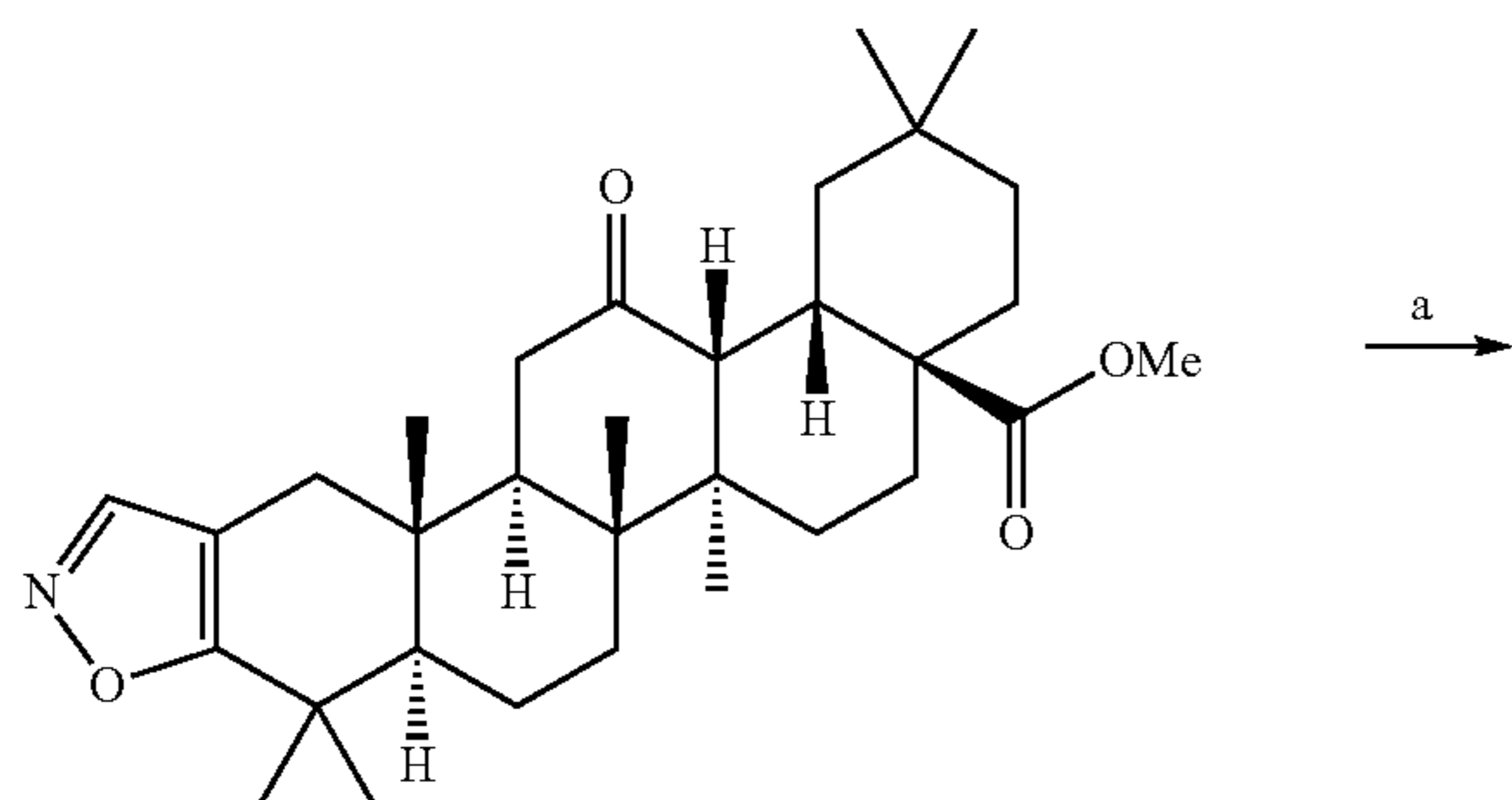
Scheme 16:
