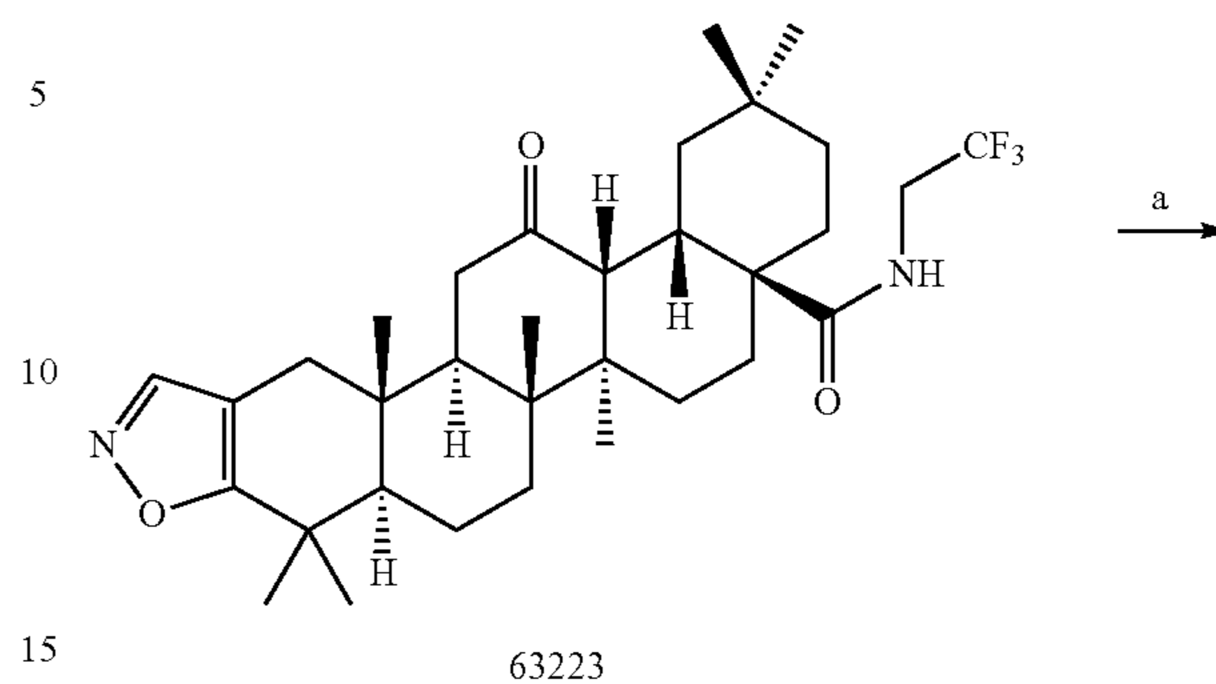
Scheme 9:
