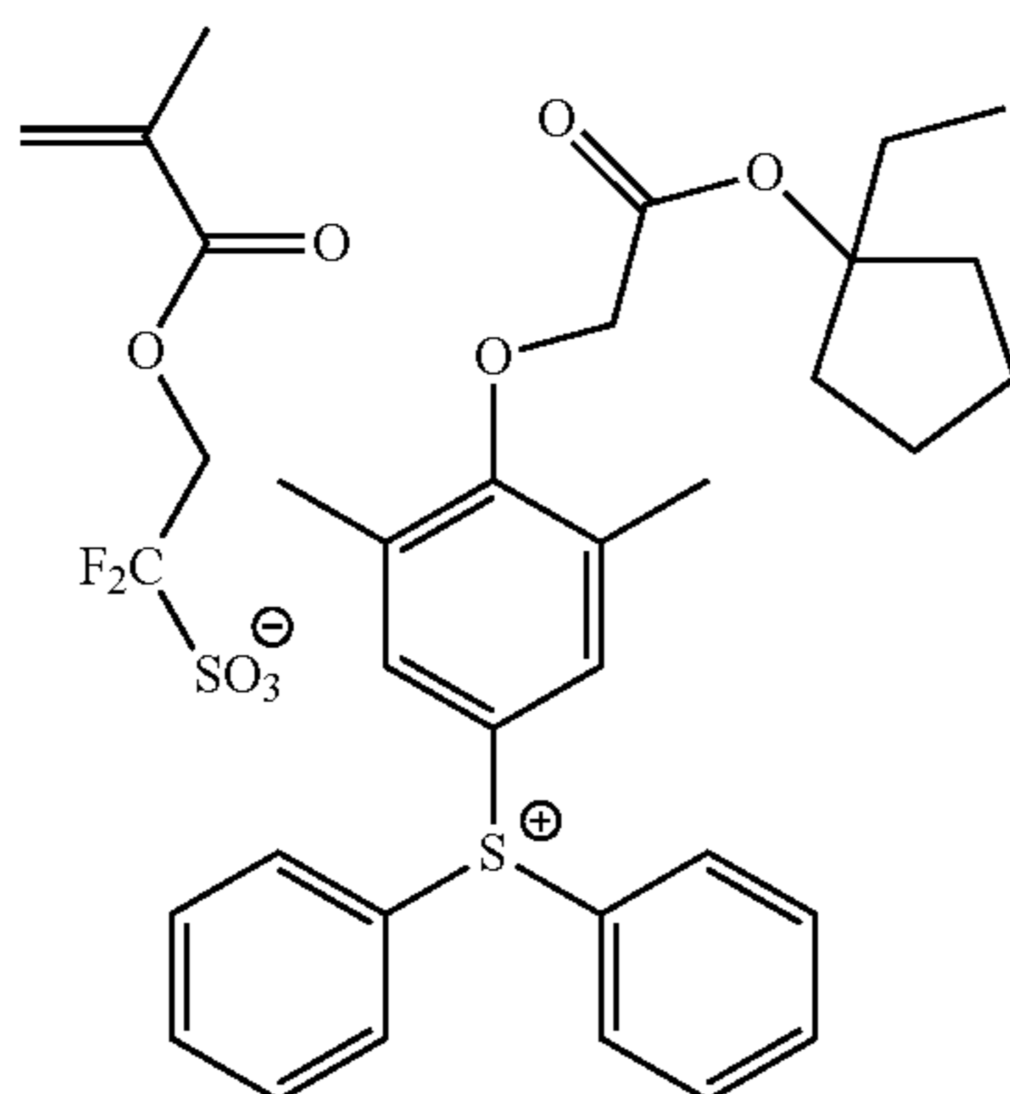
[Chemical Formula 68]
