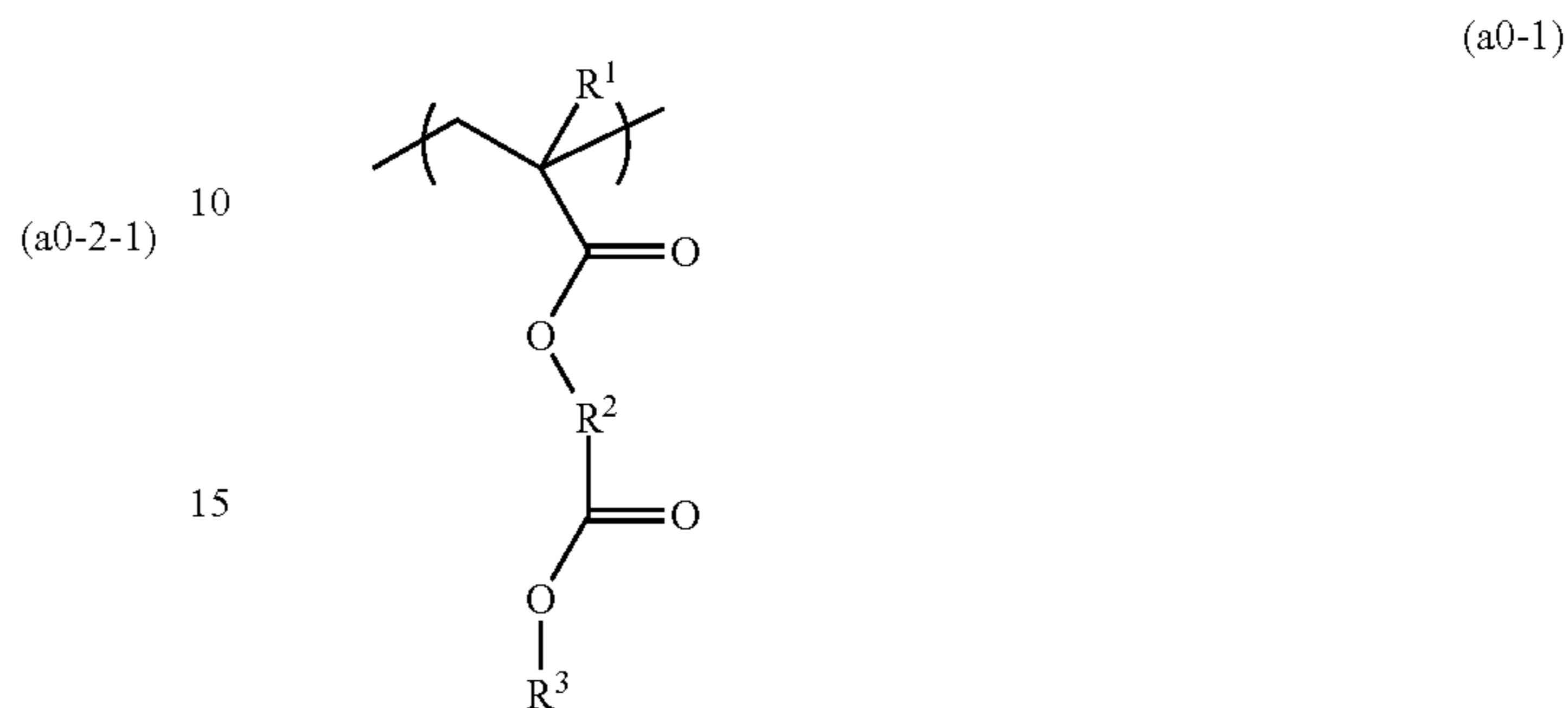
[Chemical Formula 5]
