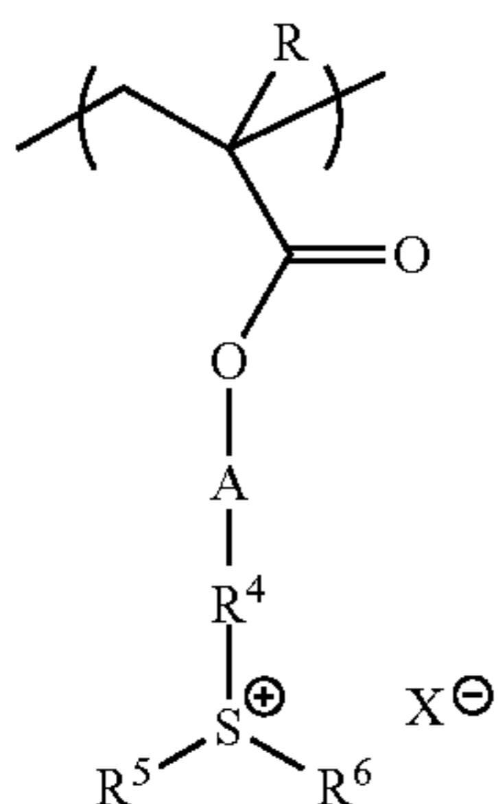
[Chemical Formula 4]
