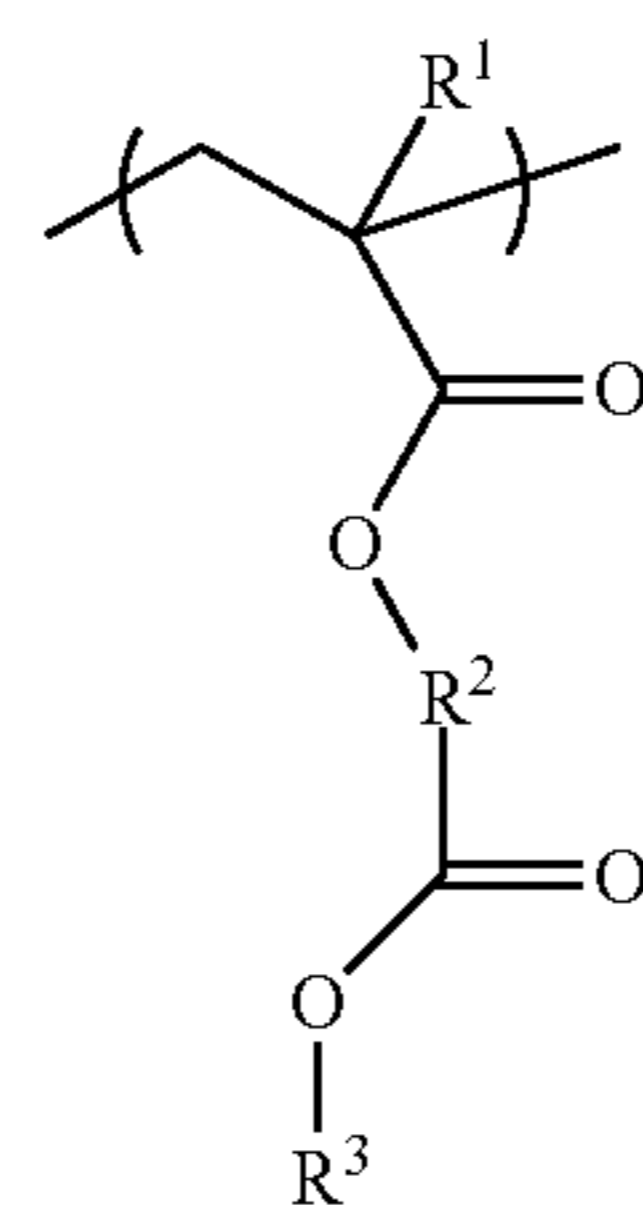
[Chemical Formula 61]
