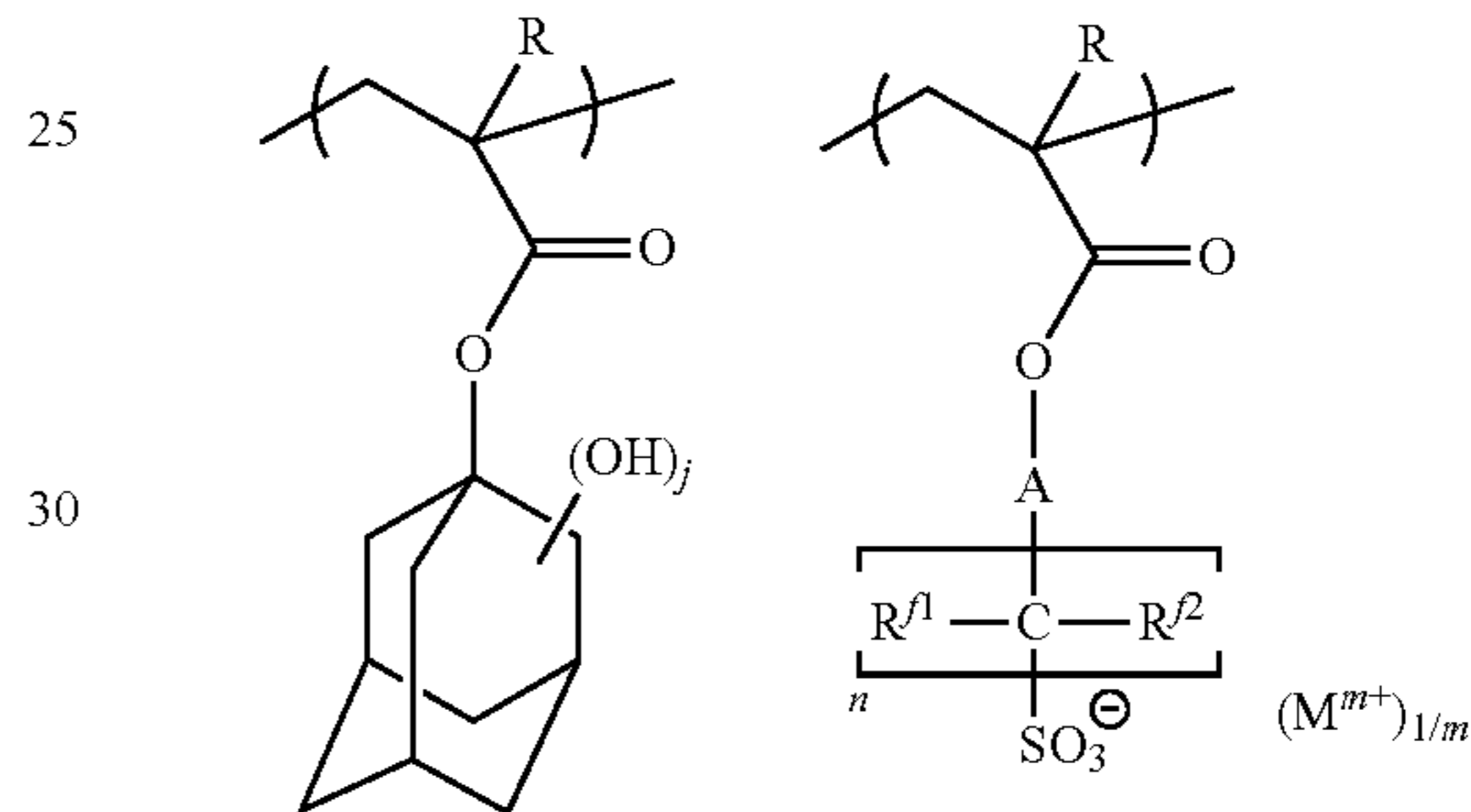
[Chemical Formula 47]
