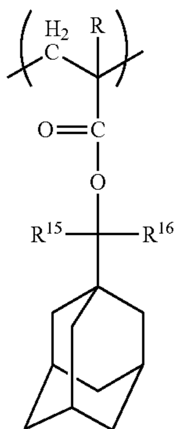
[Chemical Formula 14]
