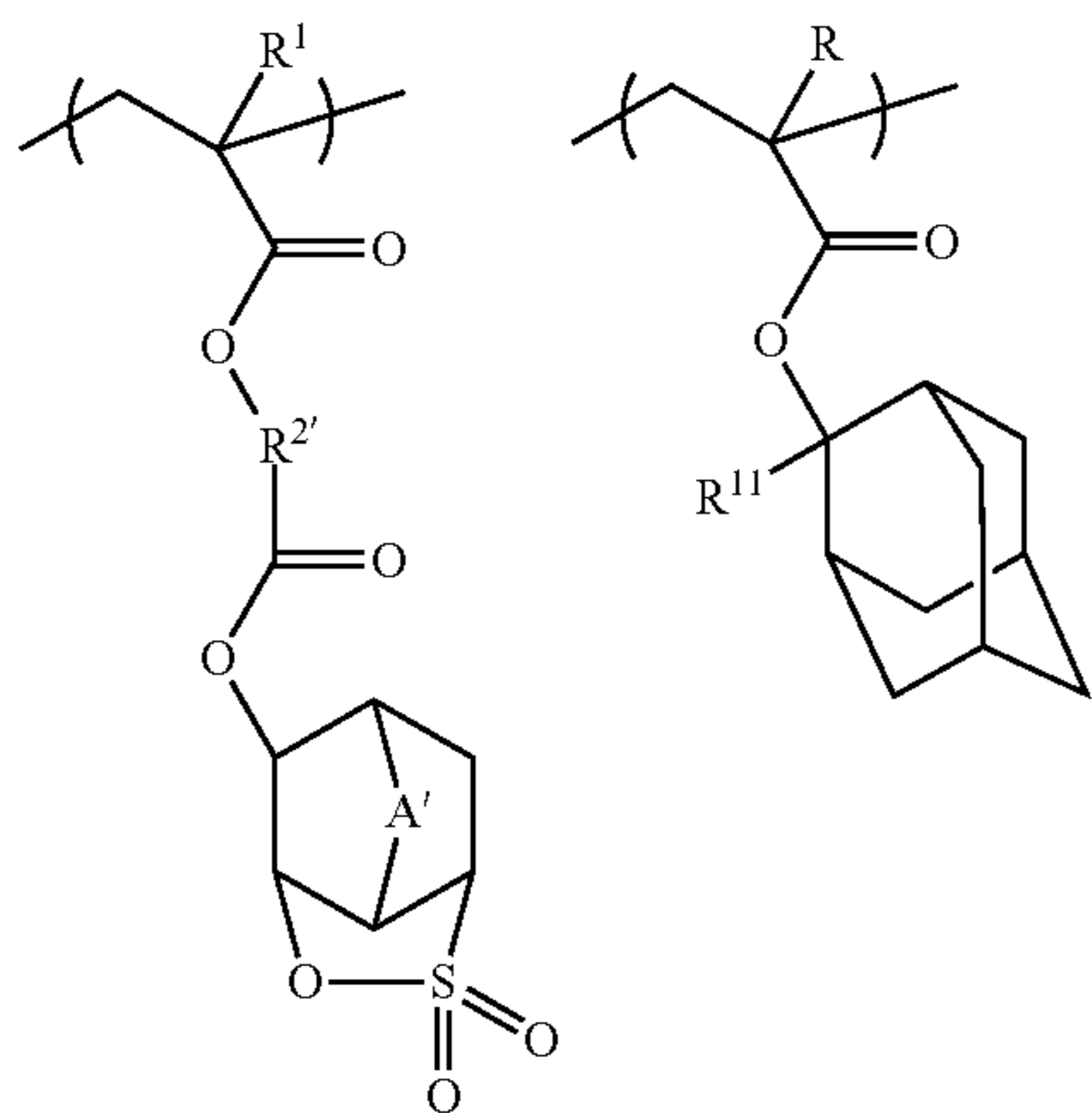
[Chemical Formula 45]
