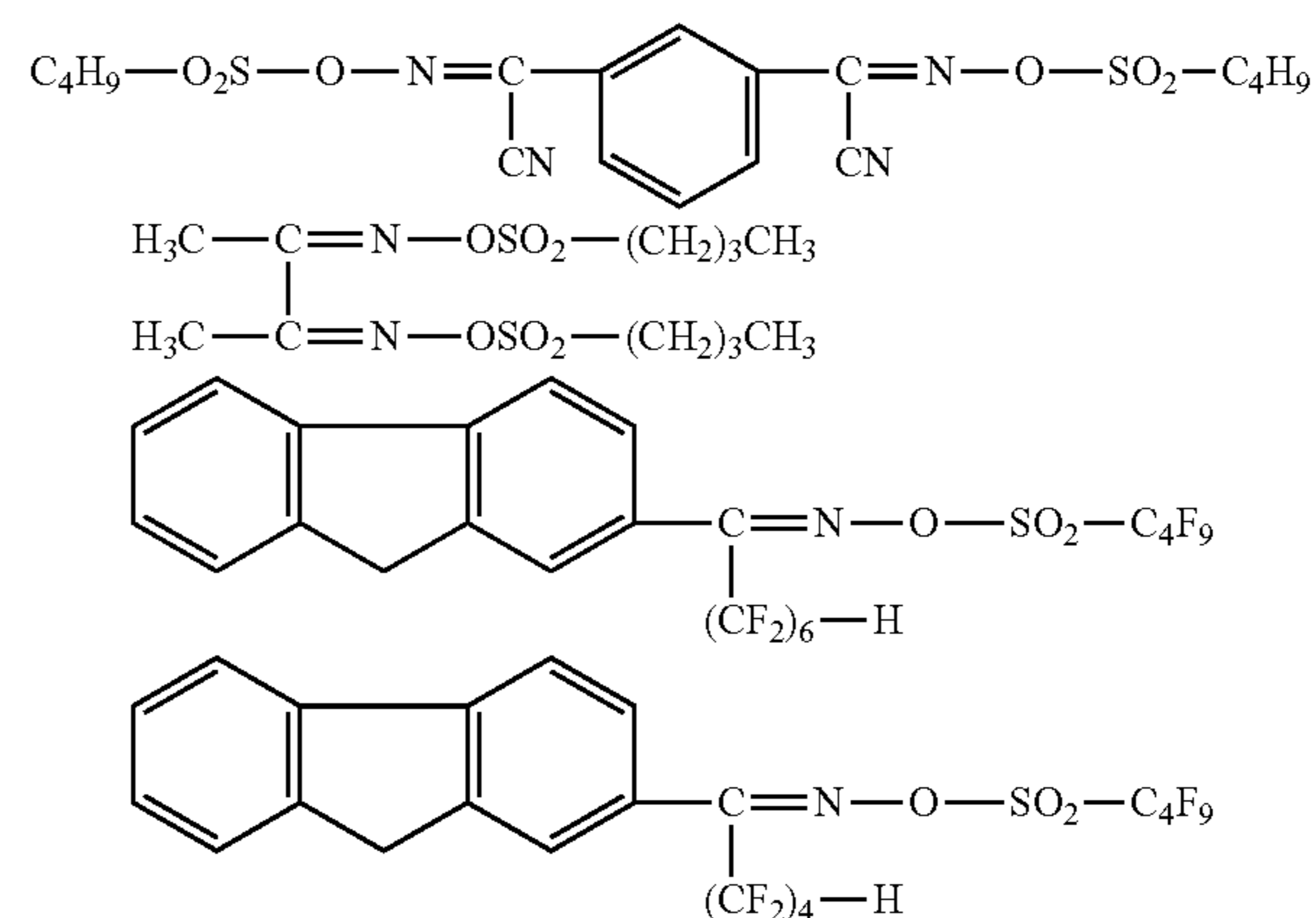
[Chemical Formula 60]
