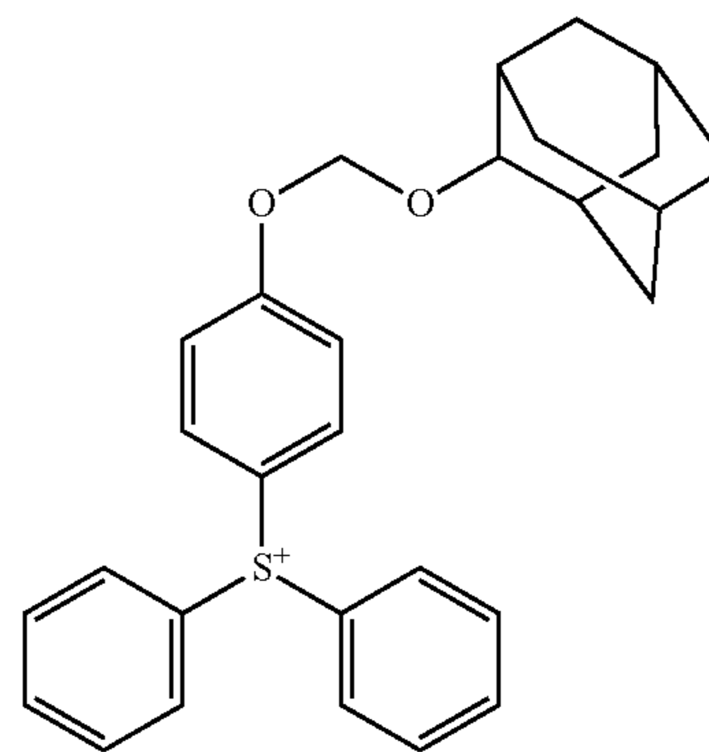
(I-1-1) 45
