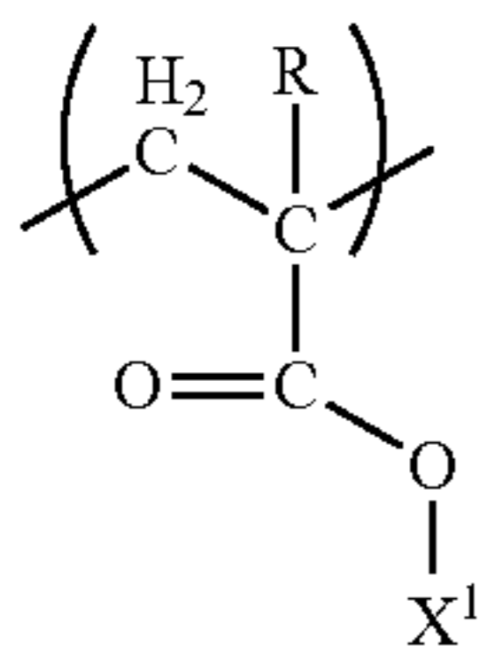
[Chemical Formula 18]
