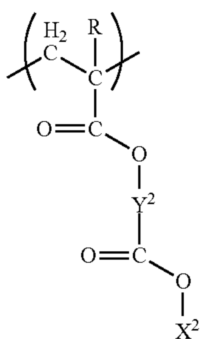
[Chemical Formula 19]
