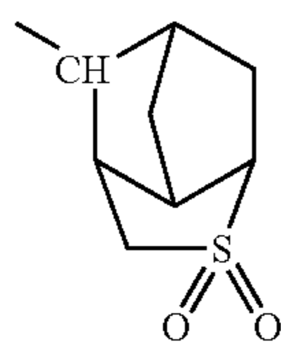
[Chemical Formula 6]
