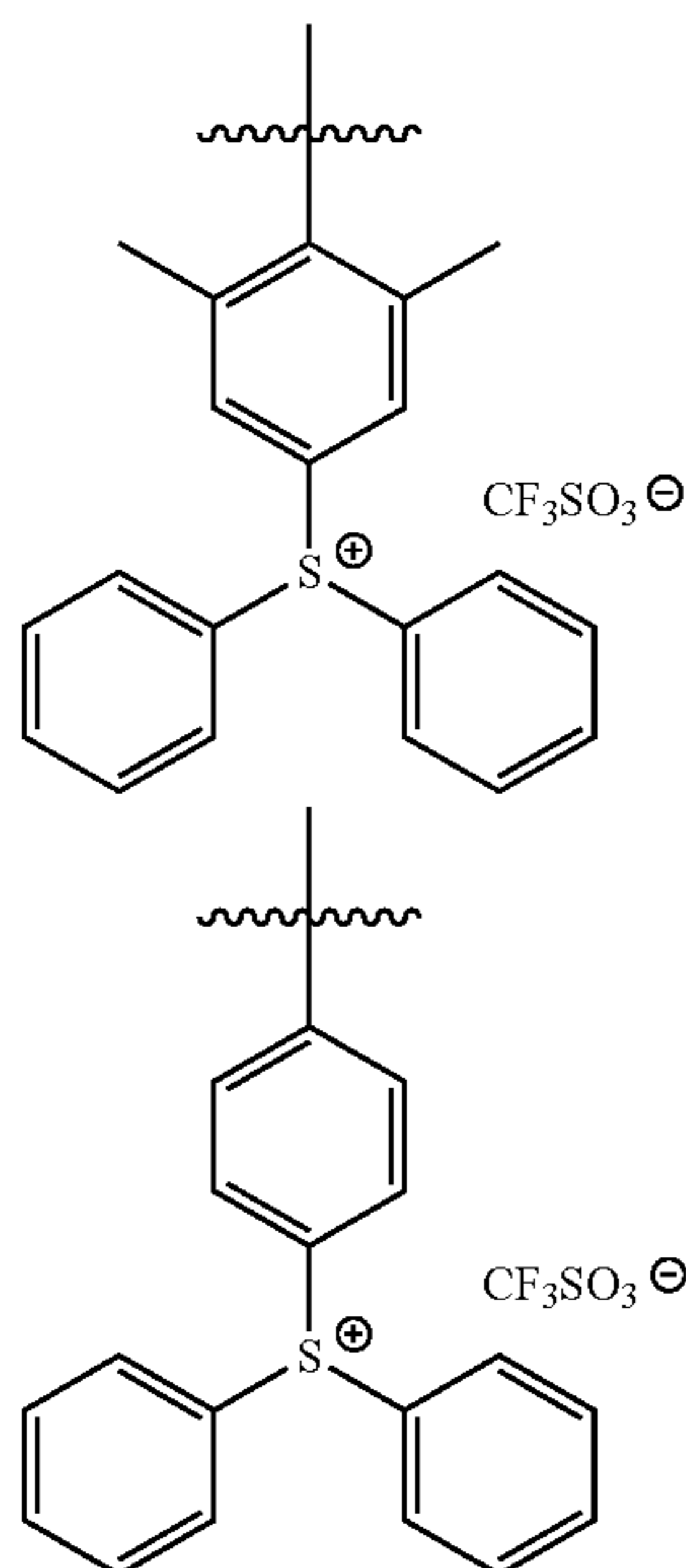
[Chemical Formula 9]
