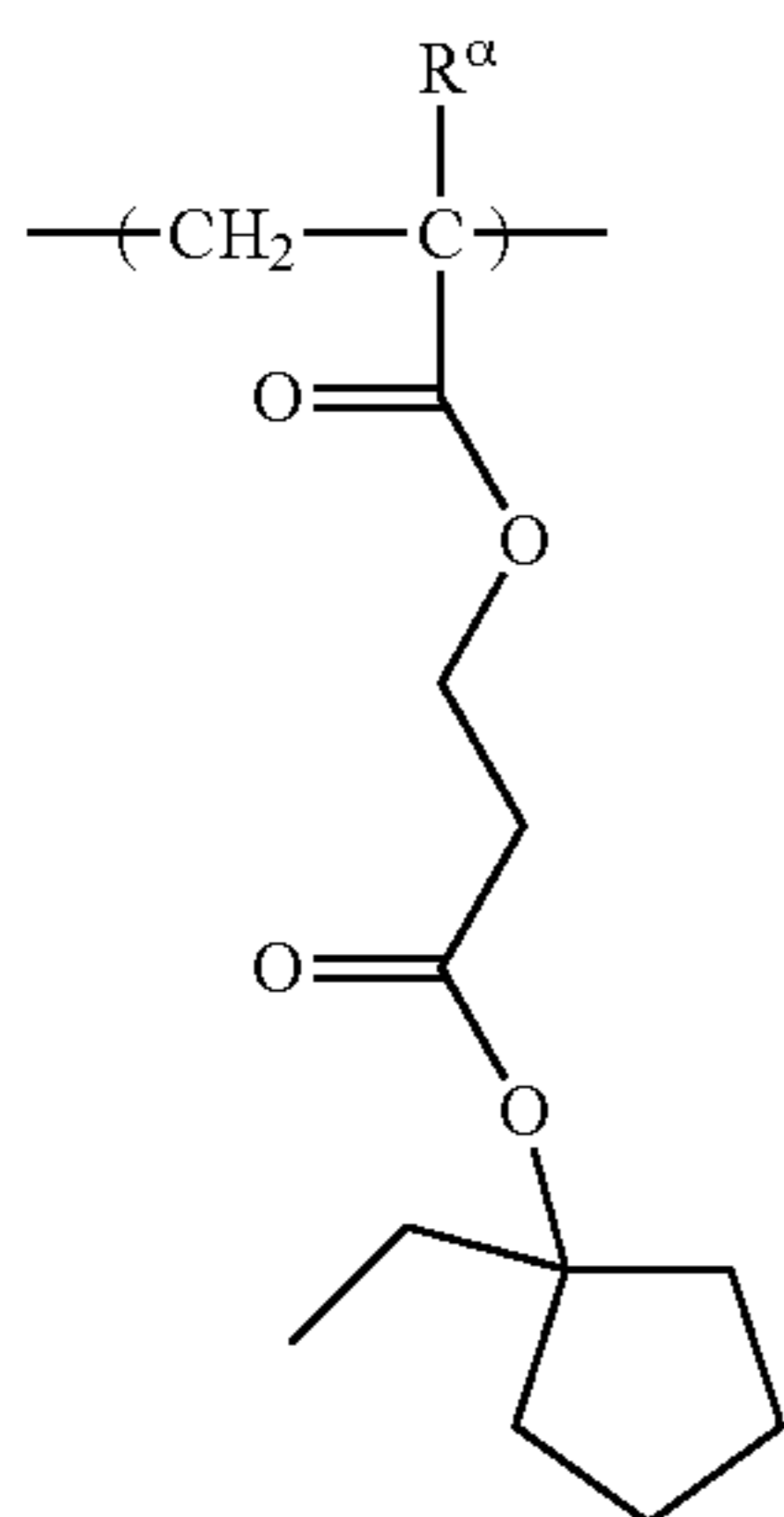
[Chemical Formula 27]
