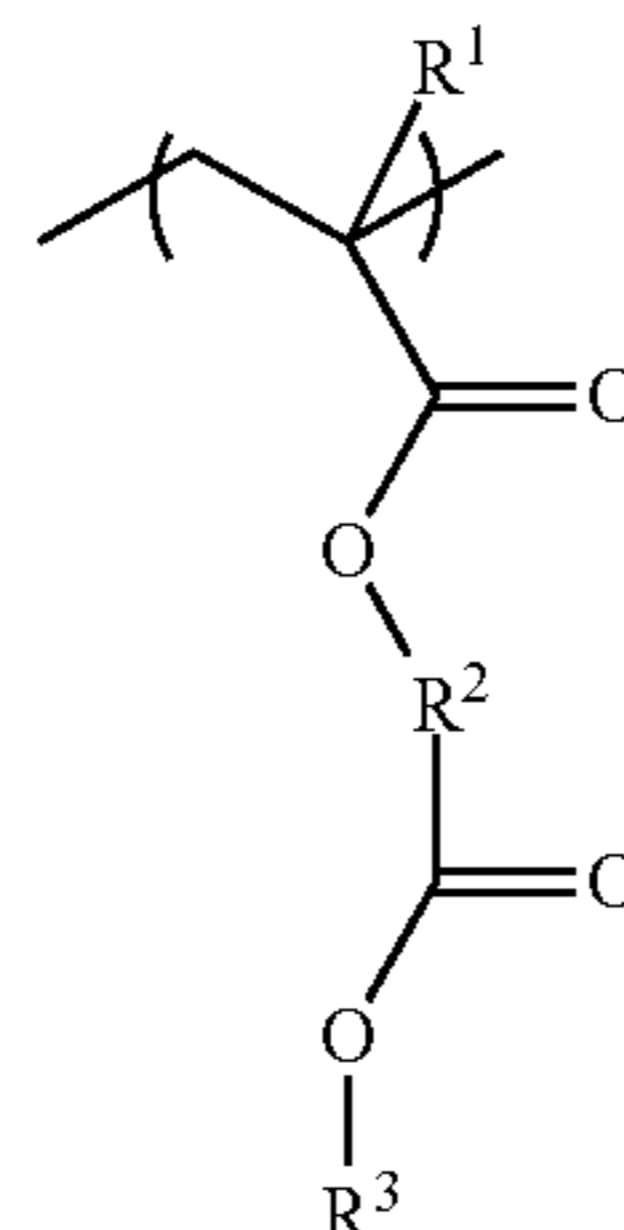
[Chemical Formula 1]
