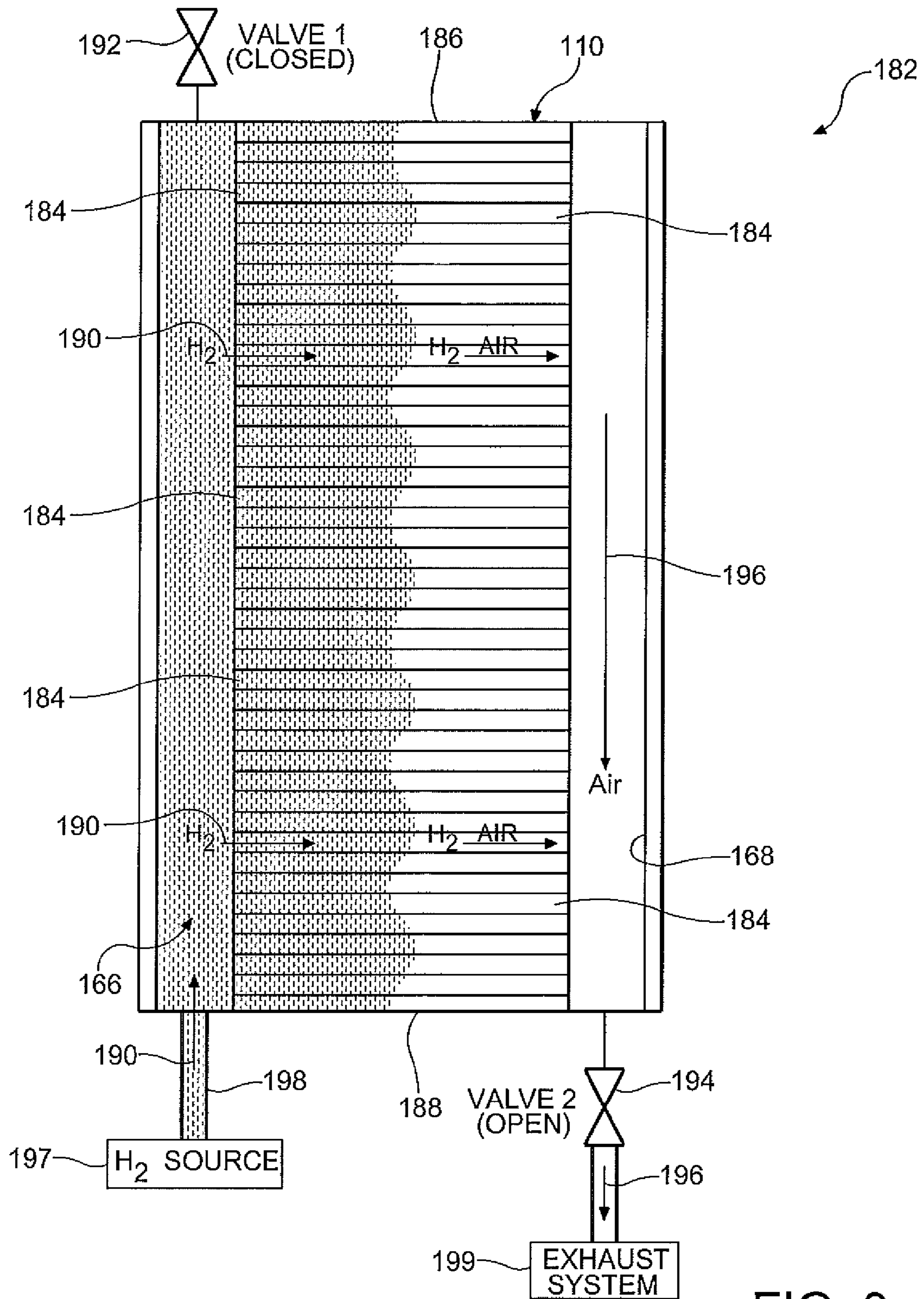
FIG. 3 (Prior Art)
