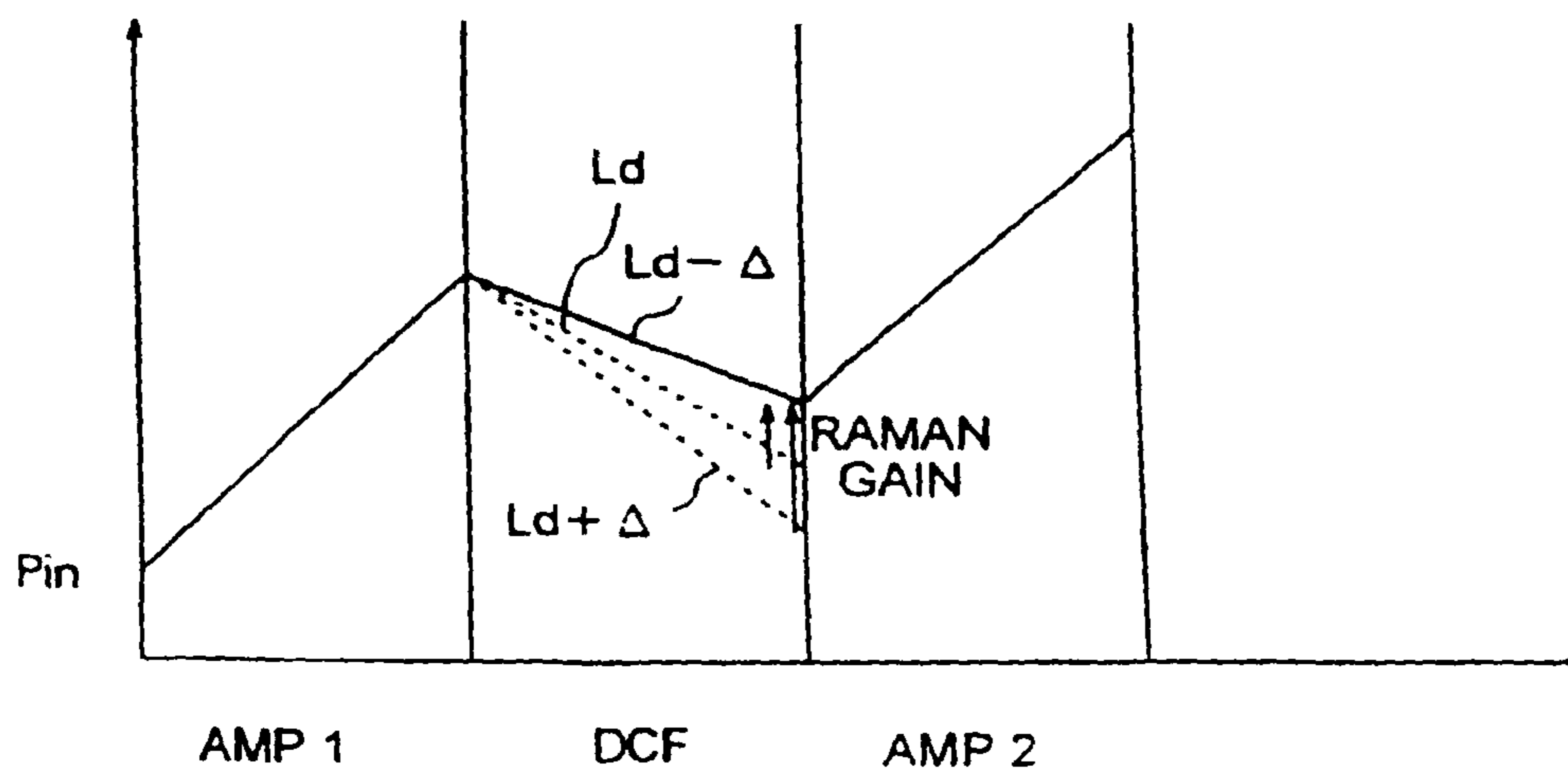
COMPENSATION FOR FLUCTUATION IN LOSS OF DCF DUE TO RAMAN AMPLIFYING EFFECT
