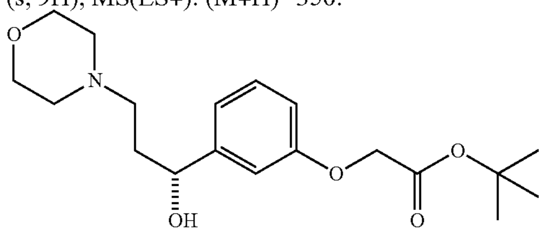
1R-(3-(tert-butoxycarbonylmethoxy)phenyl)-3-(1-morpholino)propan-1-ol
