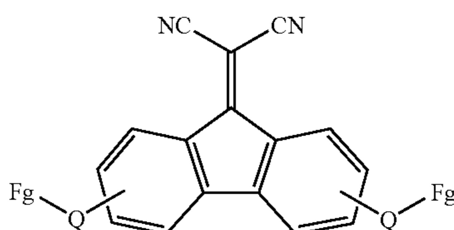
9-fluorenylidene malonitriles
