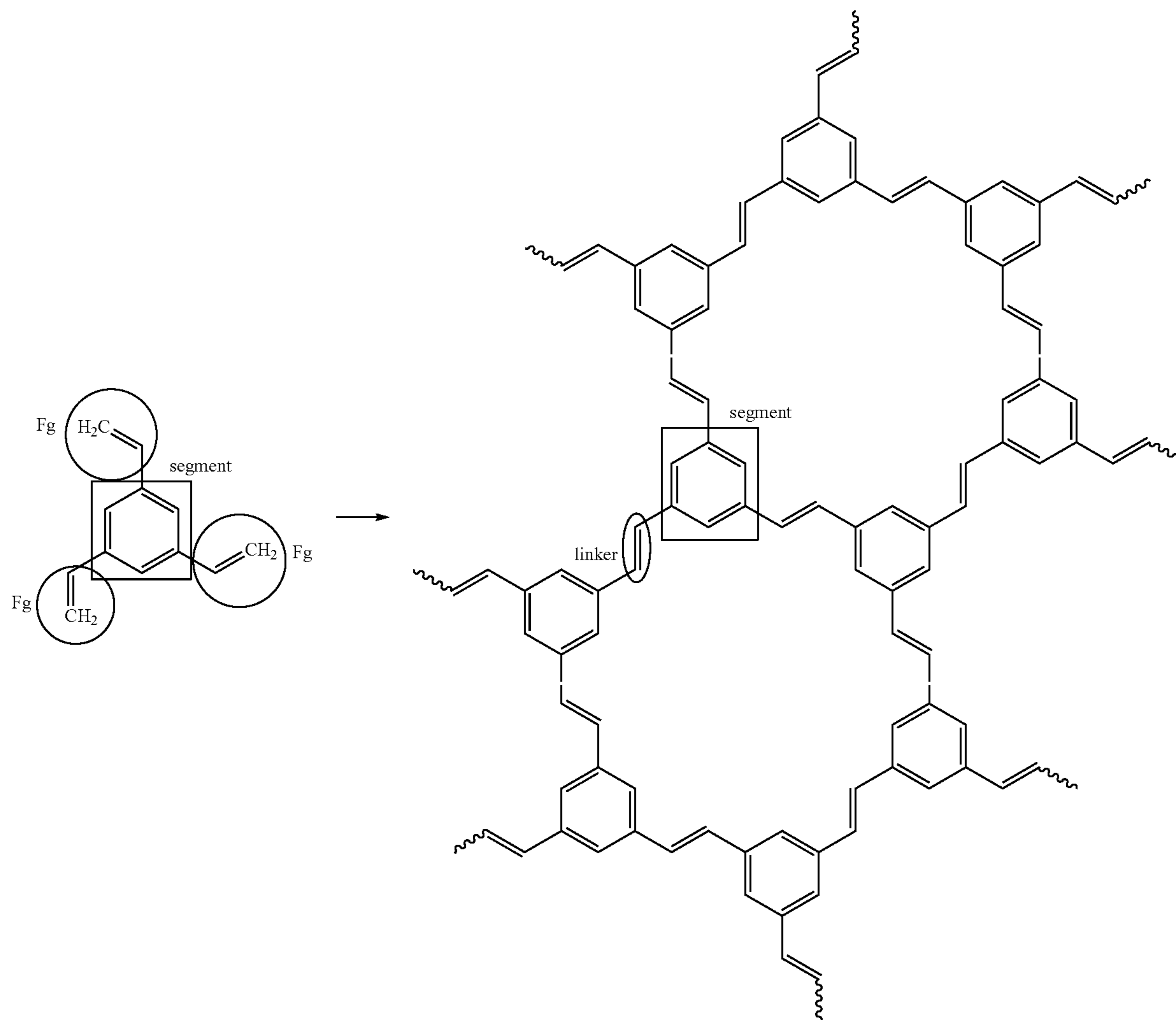
Strategy 1: Production of a Type 1 SOF using one type of molecular building block. This SOF contains an ethylene (two atom) linker type.
