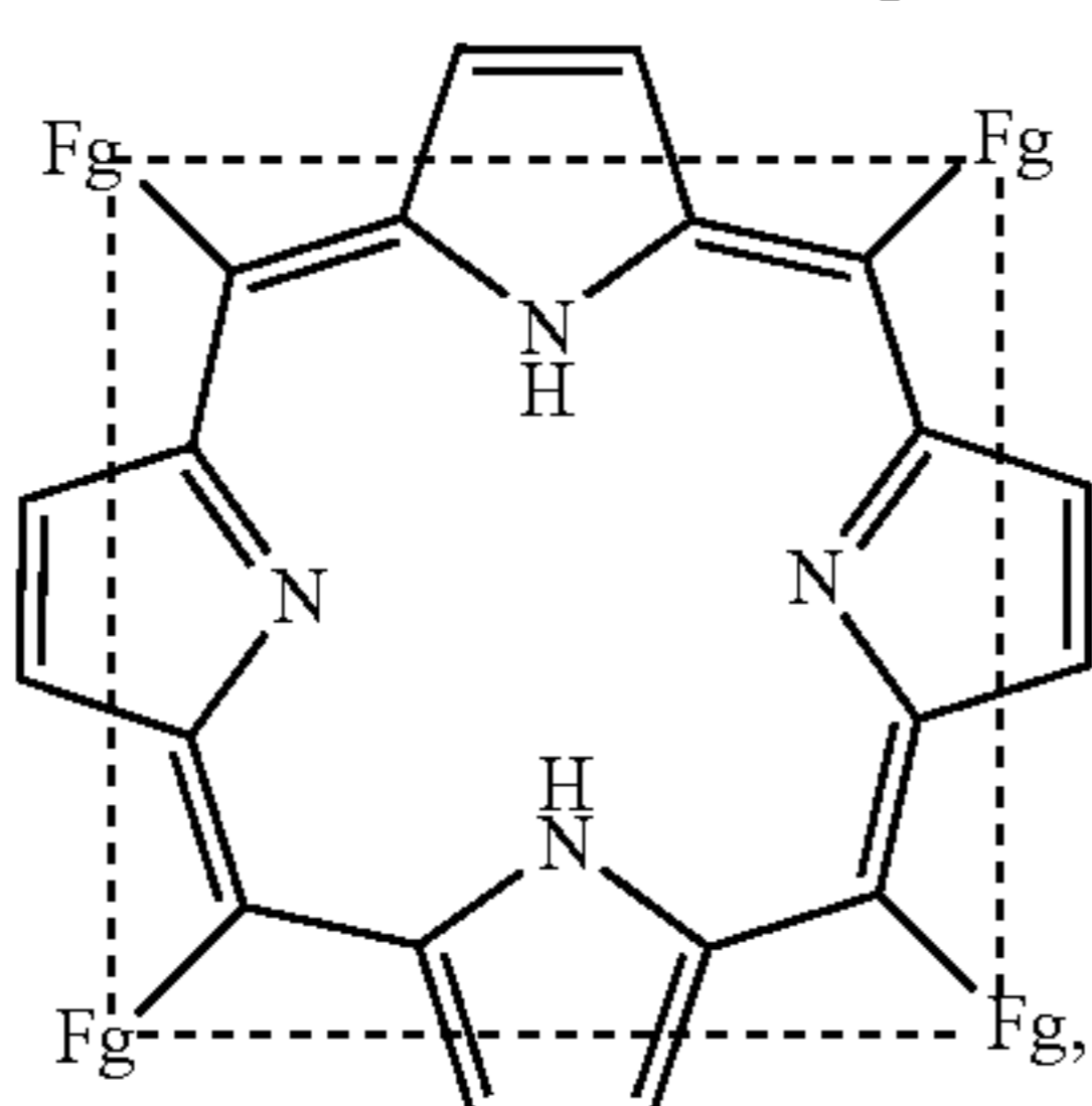
ideal square building block
