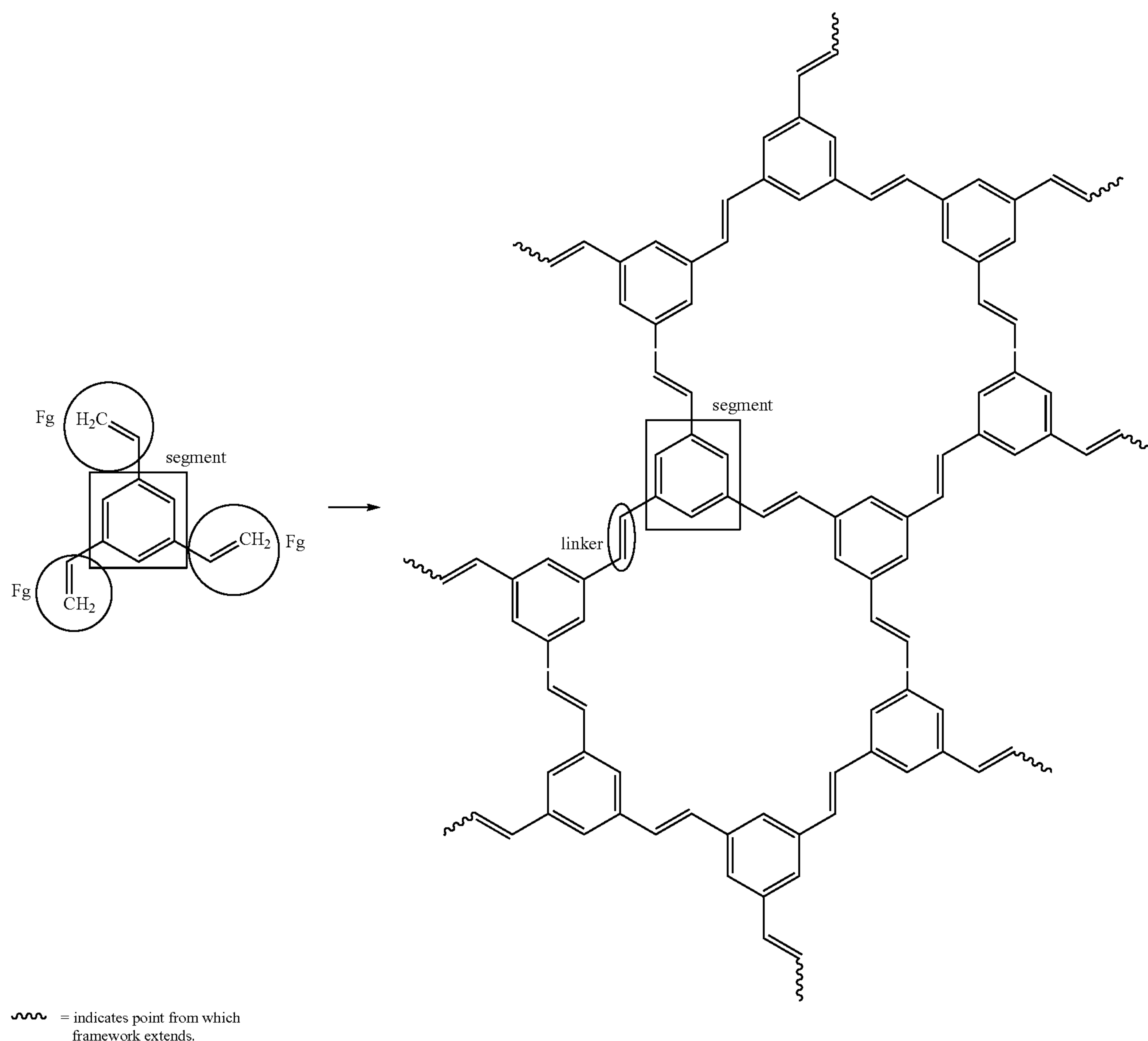
Strategy 1: Production of a Type 1 SOF using one type of molecular building block. This SOF contains an ethylene (two atom) linker type.
