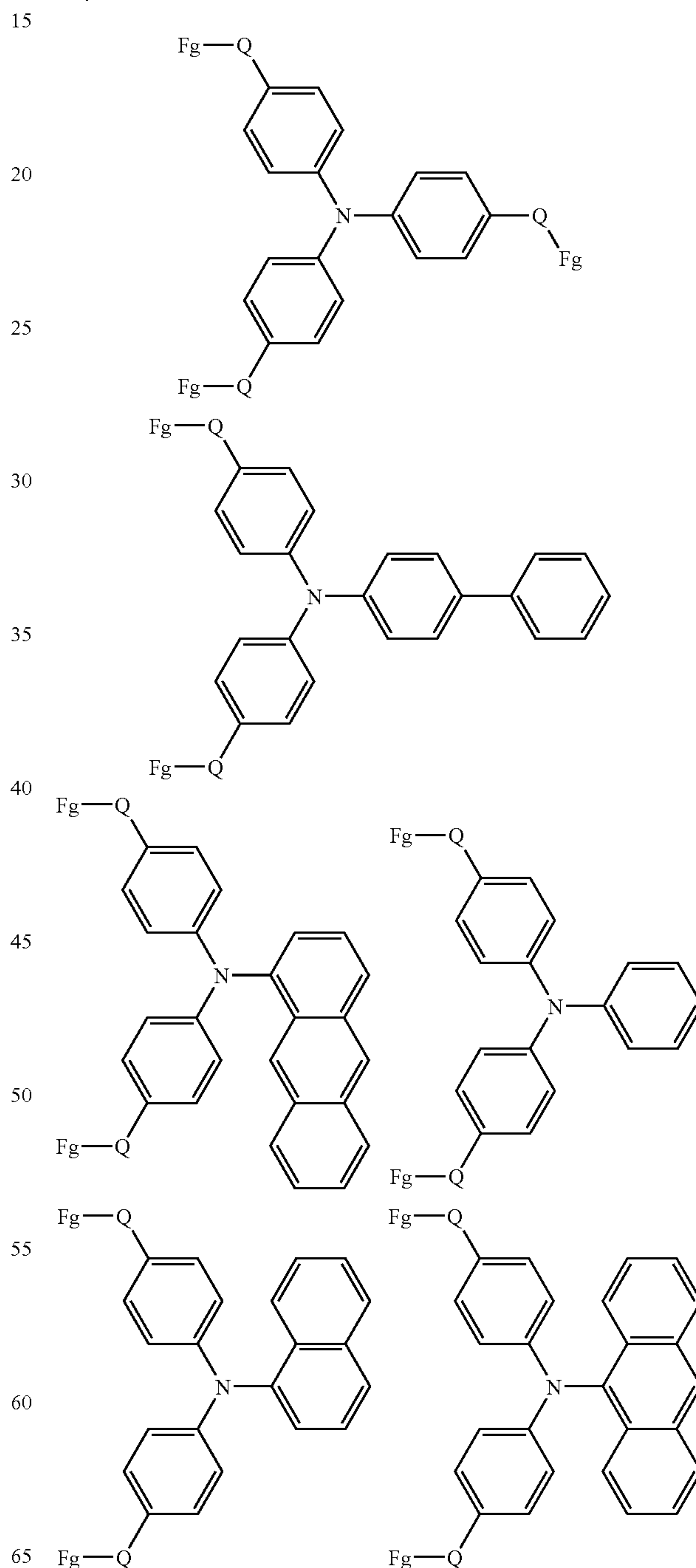
triarylamine cores
