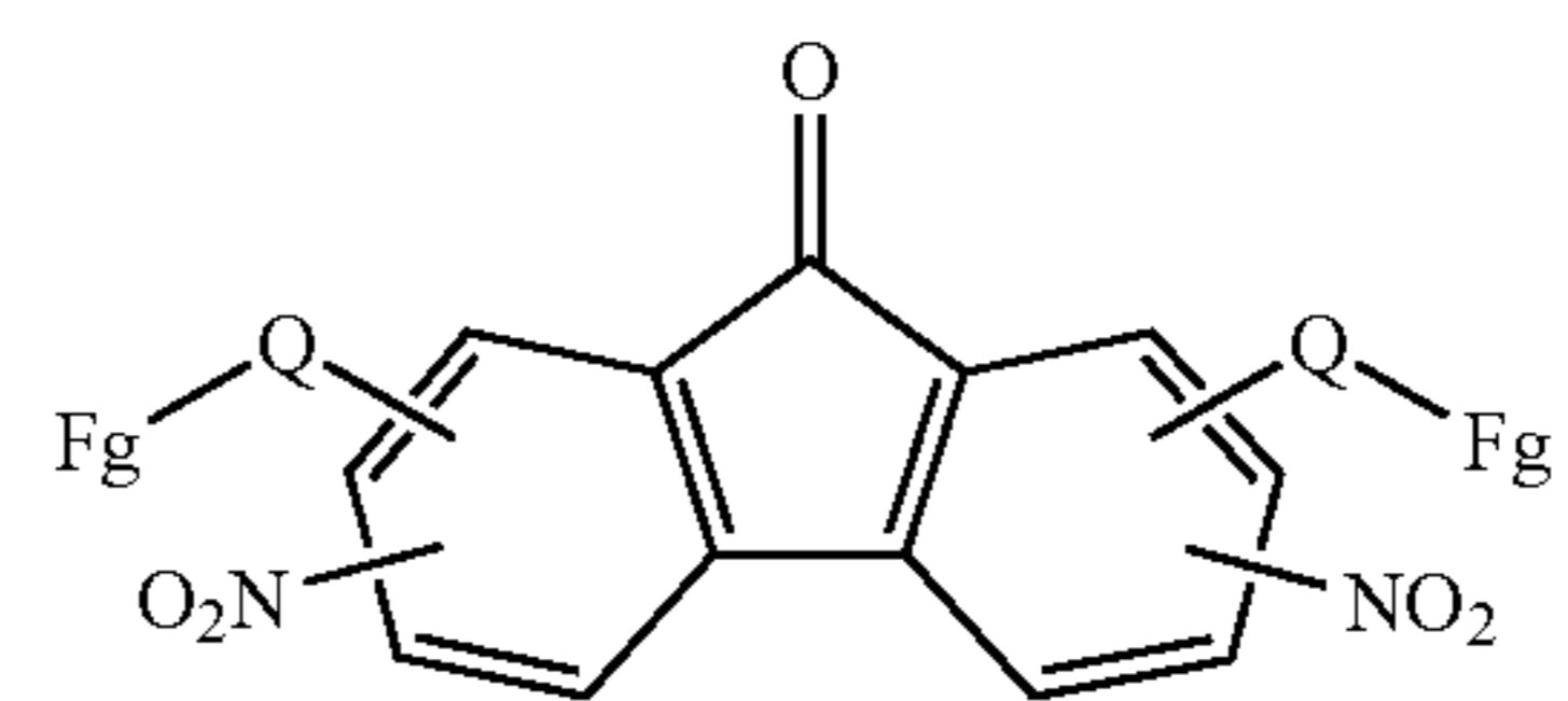
nitrofluorenones
