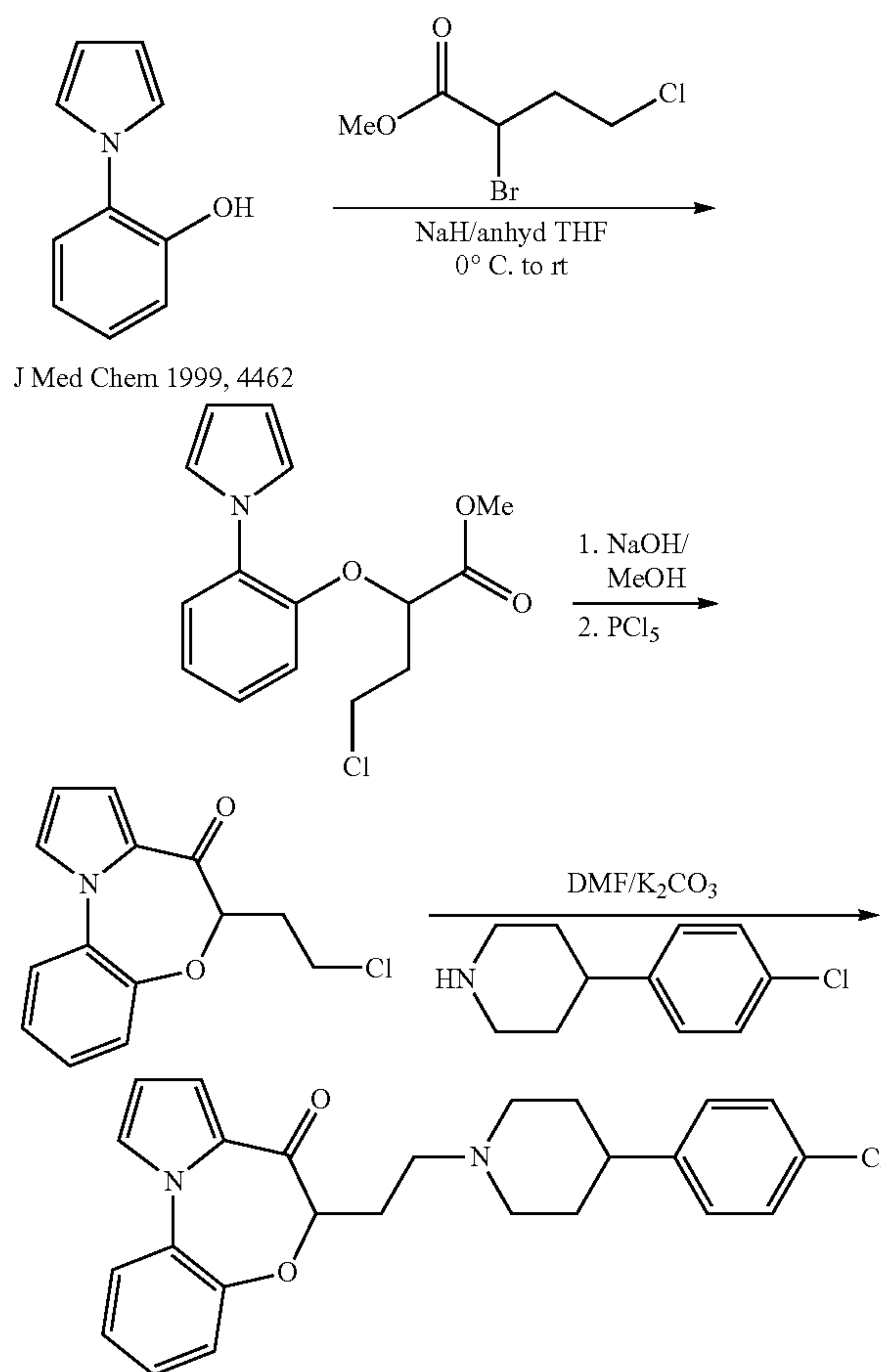
6-(2-(4-(4-chlorophenyl)piperidin-1-yl)ethyl)benzo[b]pyrrolo[1,2-d][1,4]oxazepin-7(6H)-one
