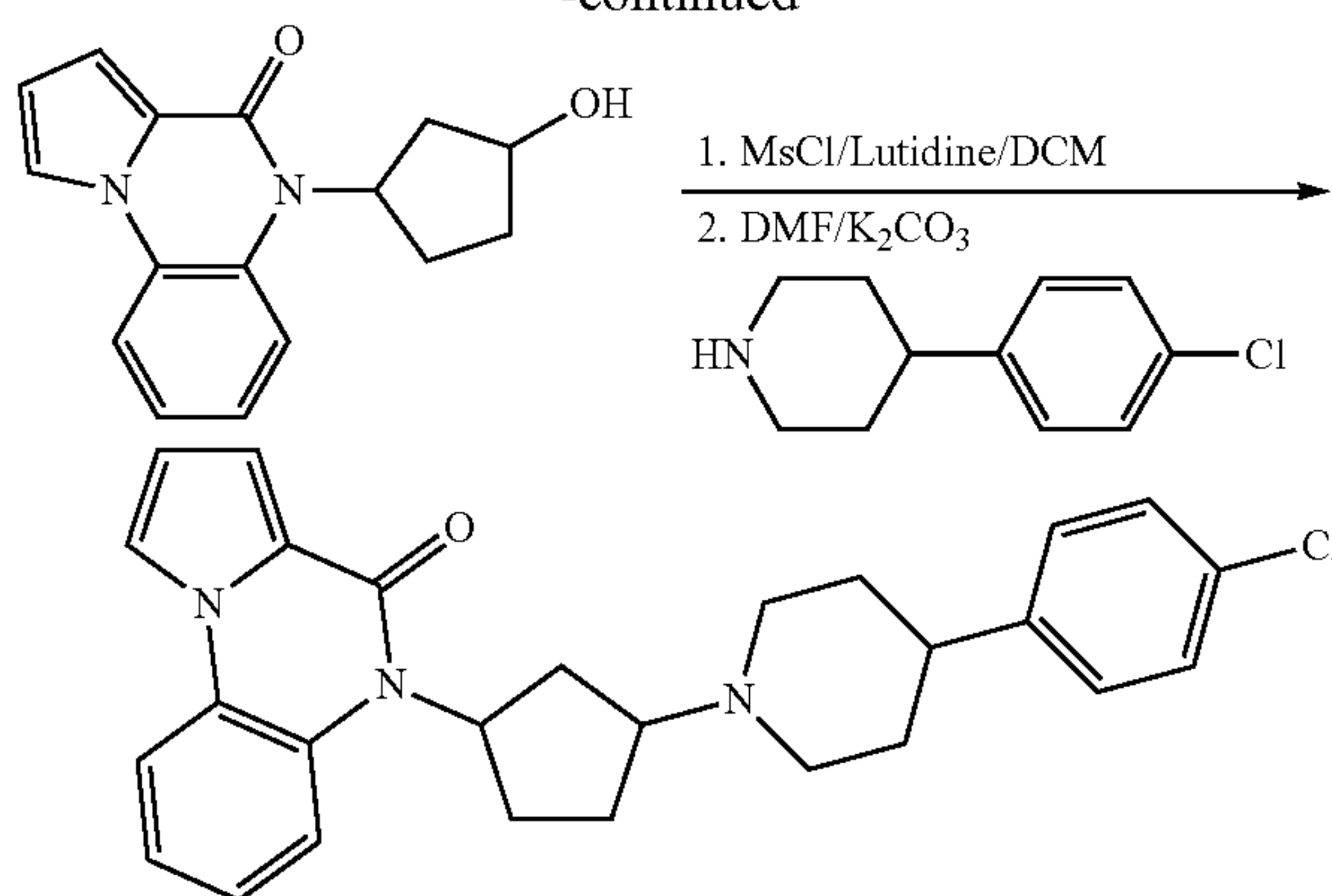
5-(3-(4-(4-chlorophenyl)piperidin-1-yl)cyclopentyl)pyrrolo[1,2-a]quinoxalin-4(5H)-one
