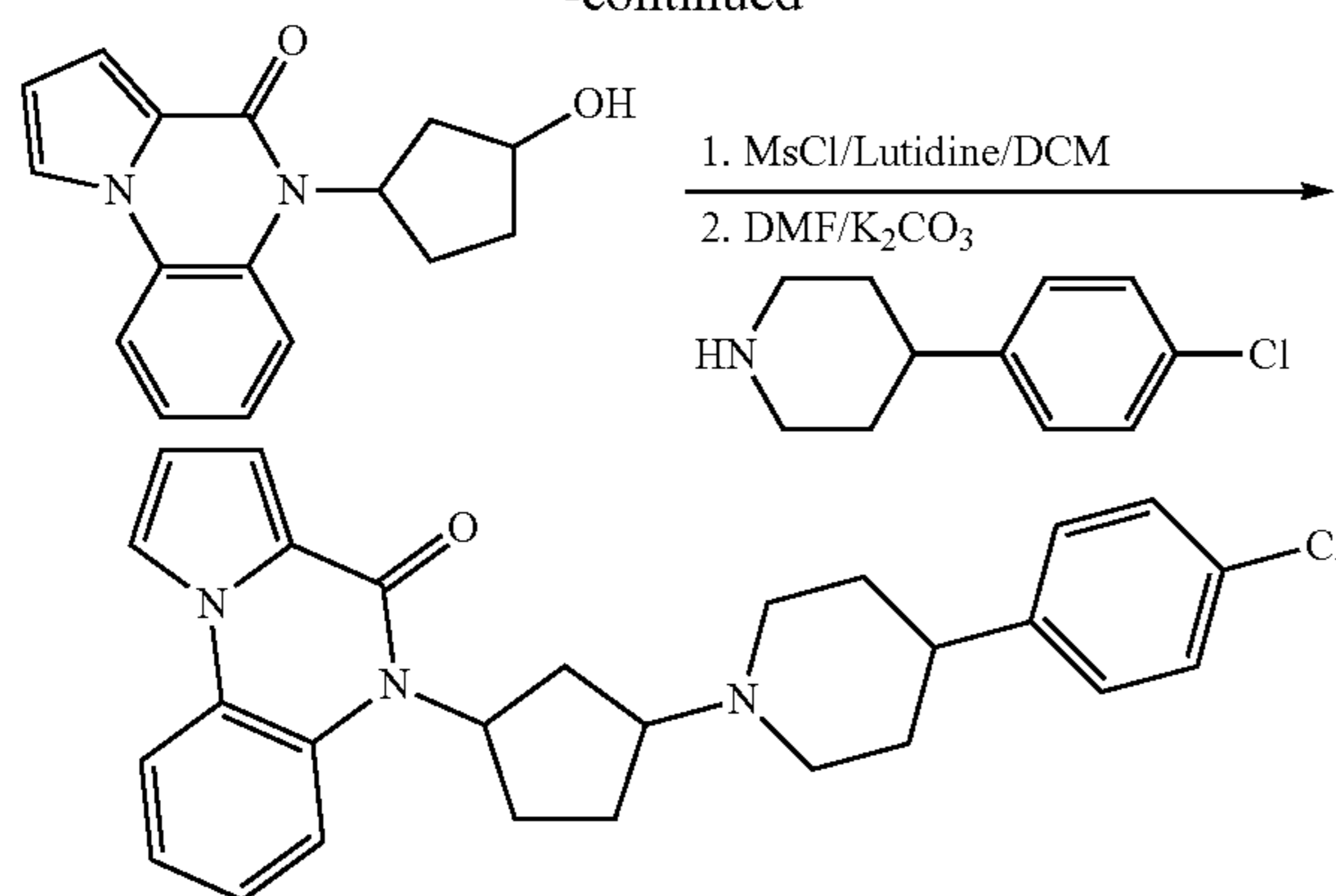
5-(3-(4-(4-chlorophenyl)piperidin-1-yl)cyclopentyl)pyrrolo[1,2-a]quinoxalin-4(5H)-one
