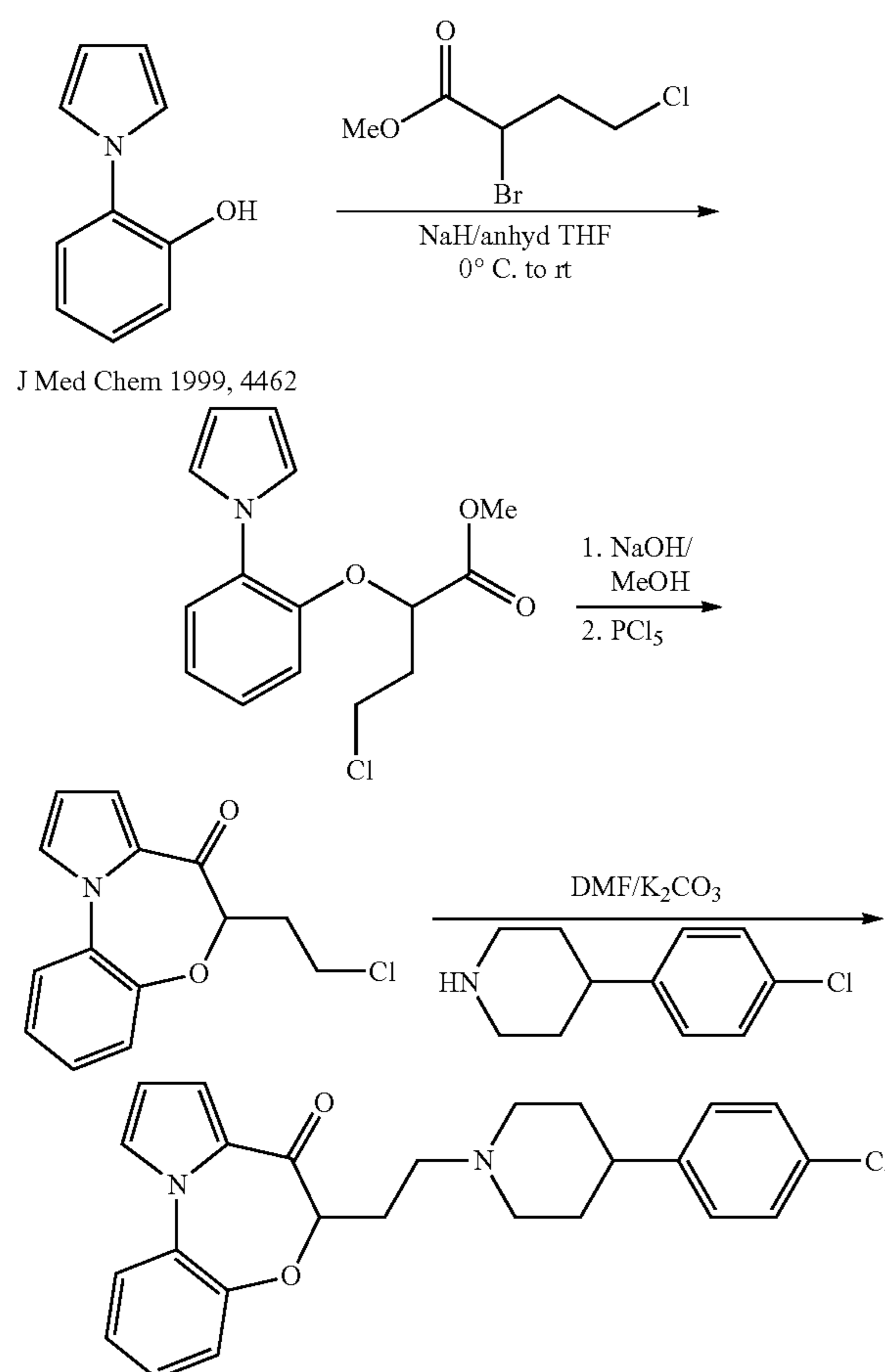
6-(2-(4-(4-chlorophenyl)piperidin-1-yl)ethyl)benzo[b]pyrrolo[1,2-d][1,4]oxazepin-7(6H)-one
