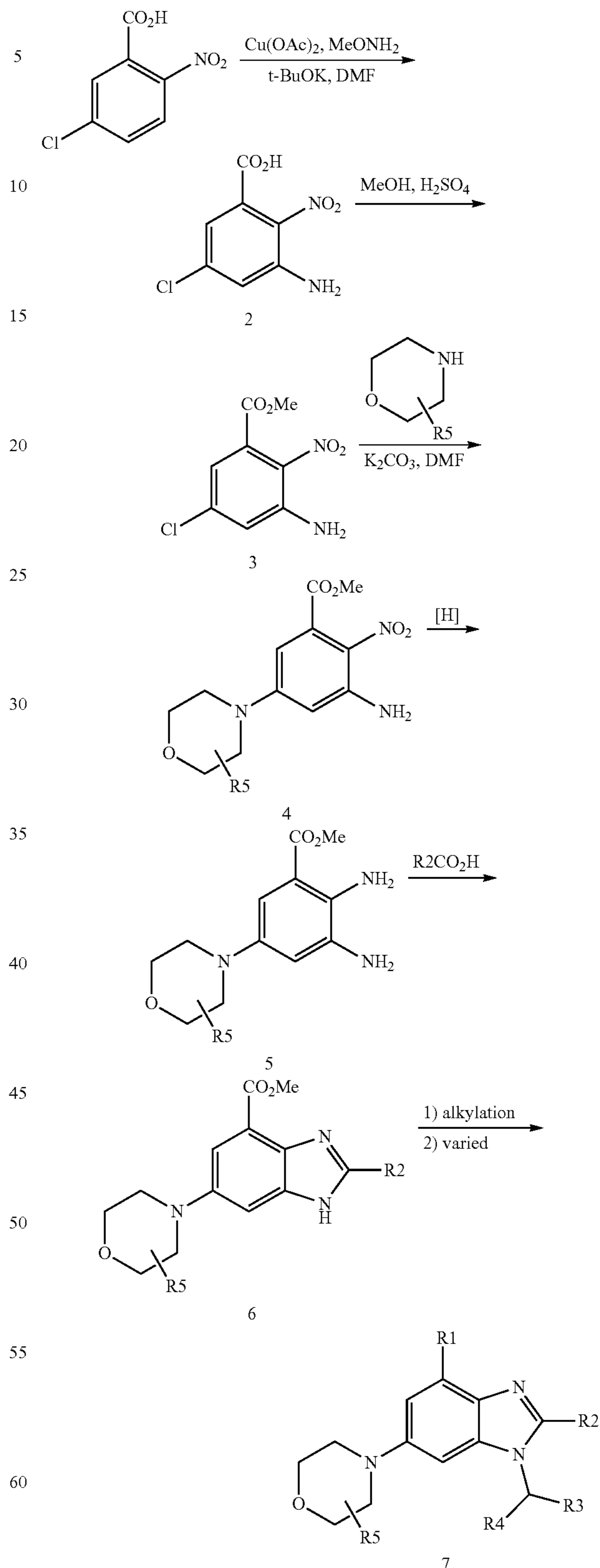
Scheme VII
