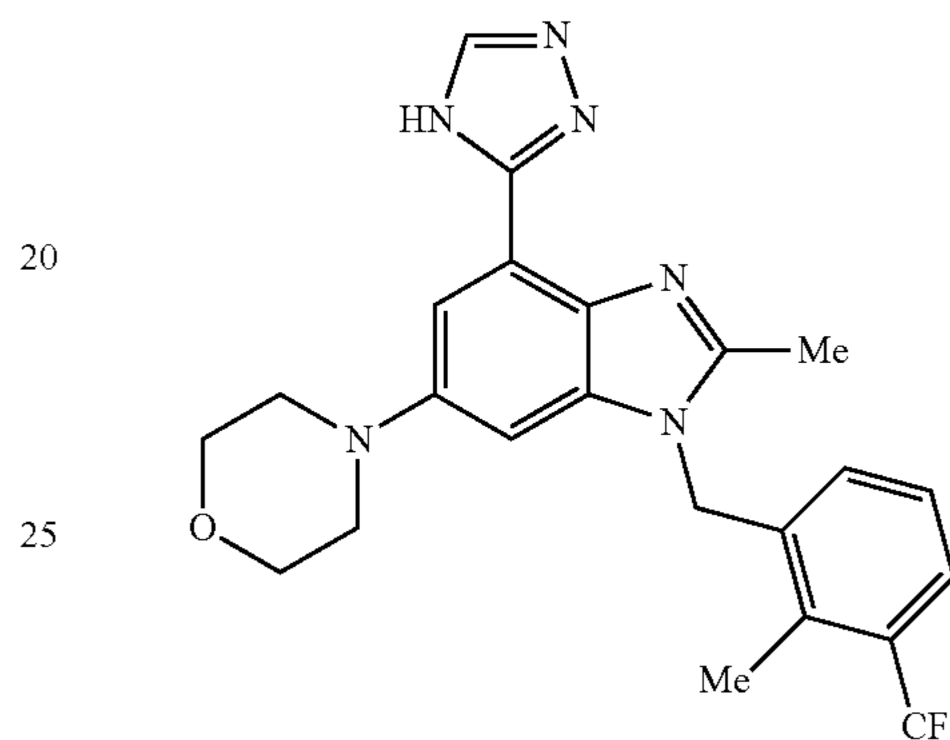
Preparation of 2-methyl-1-([2-methyl-3-(trifluoromethyl)phenyl]methyl)-6-(4-morpholinyl)-4-(1H-1,2,4-triazol-3-yl)-1H-benzimidazole
