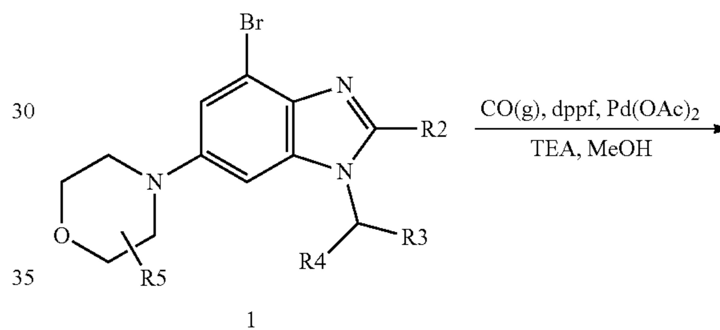
Scheme V
