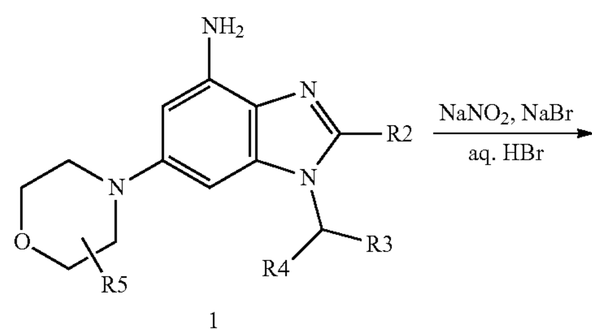
Scheme IV
