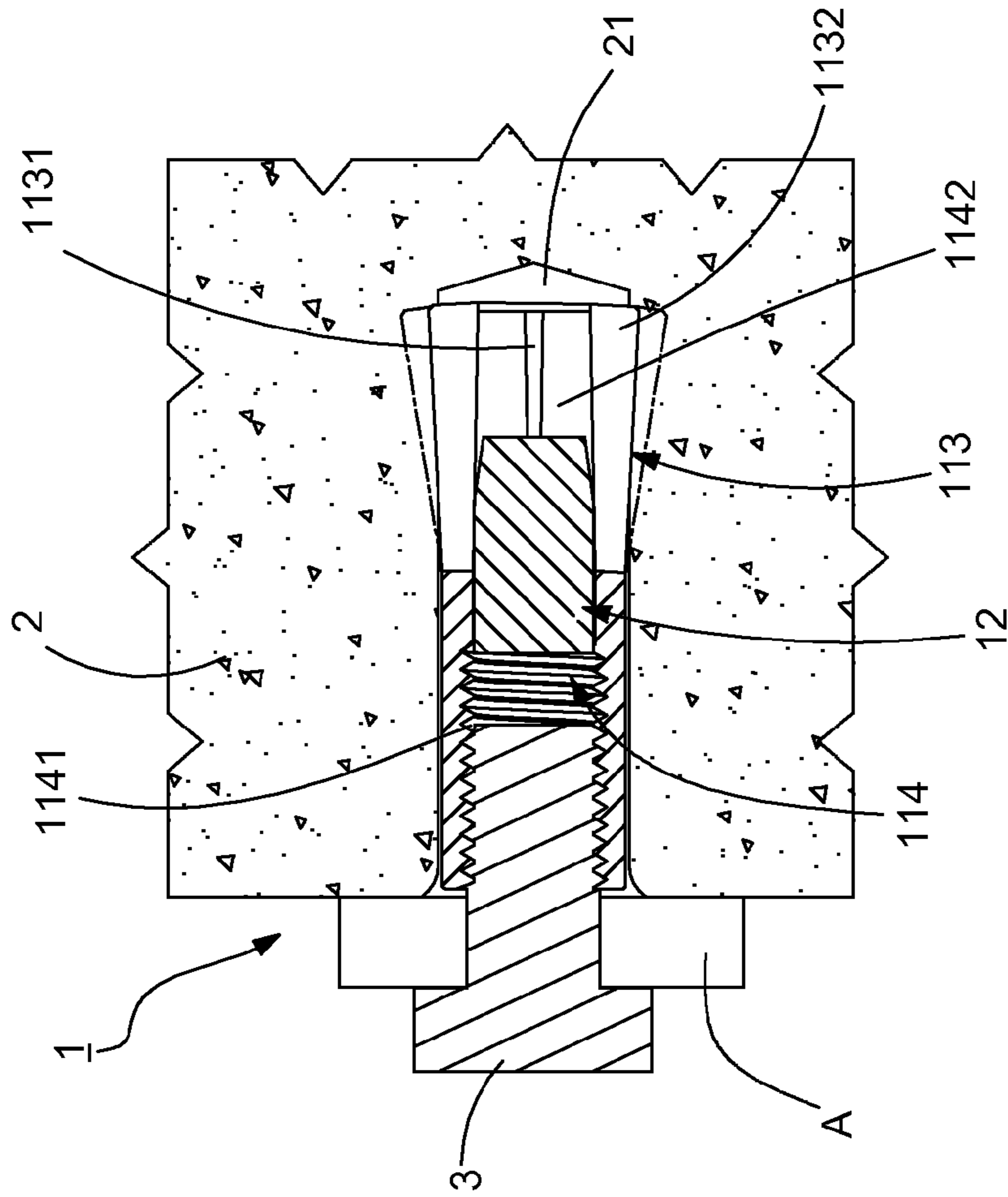
FIG. 3 (PRIOR ART)
