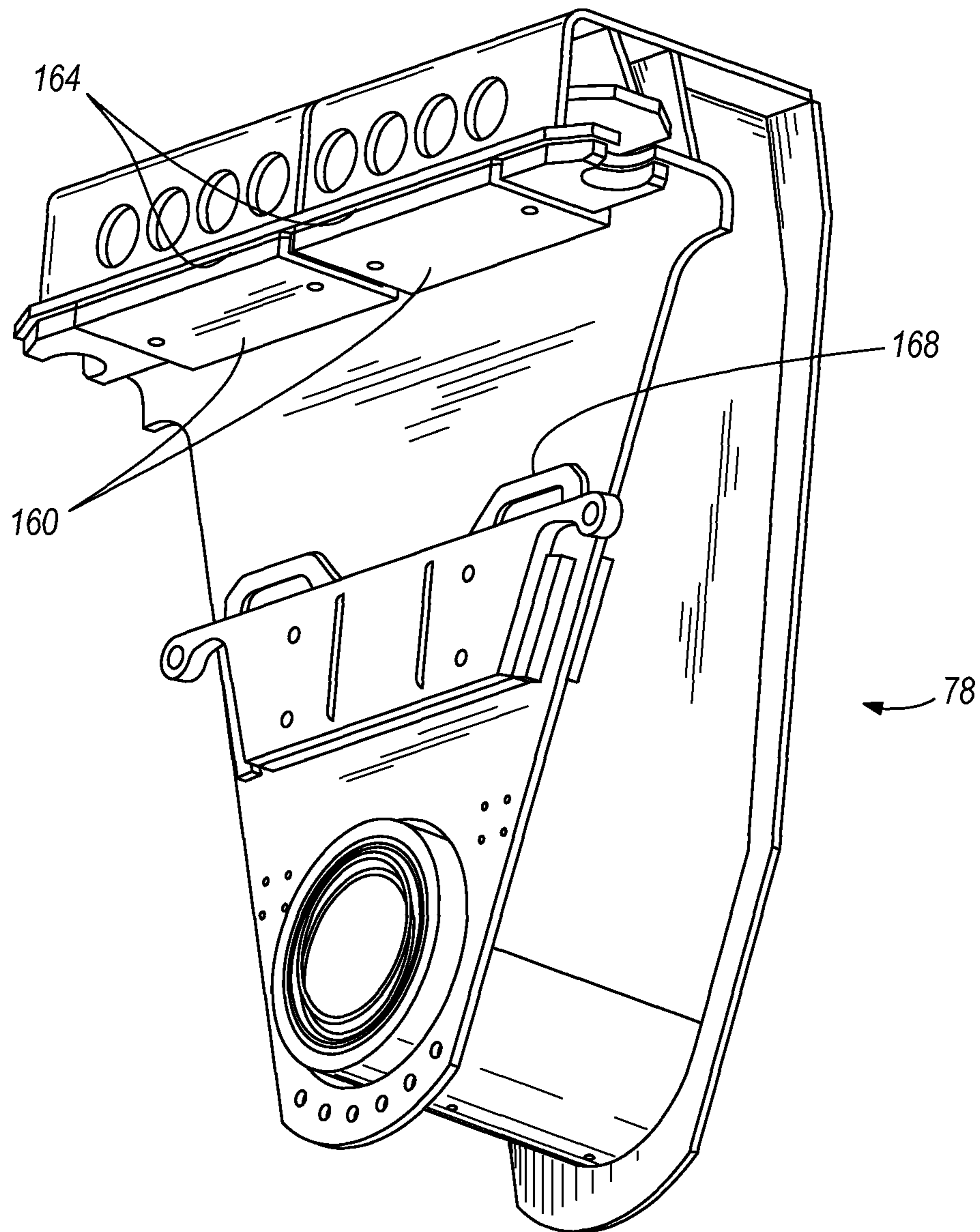
FIG. 3 PRIOR ART
