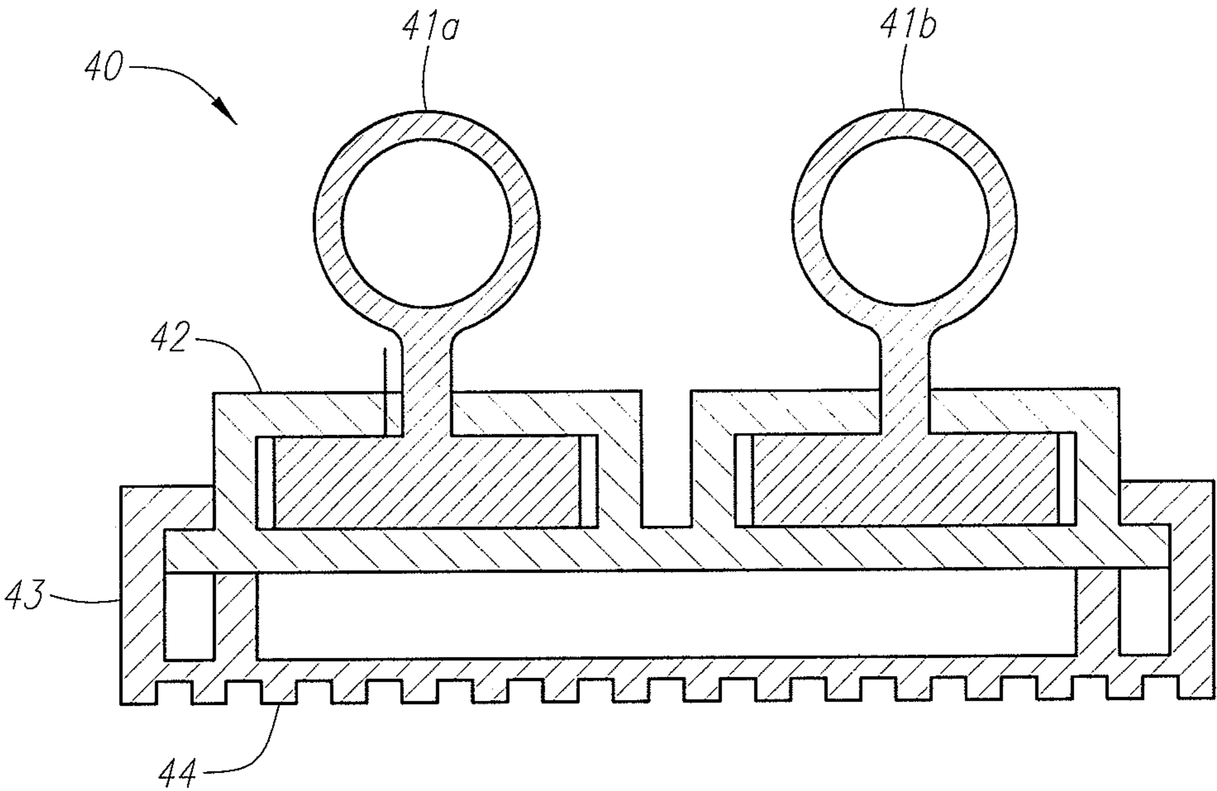
FIG. 4 (PRIOR ART)
