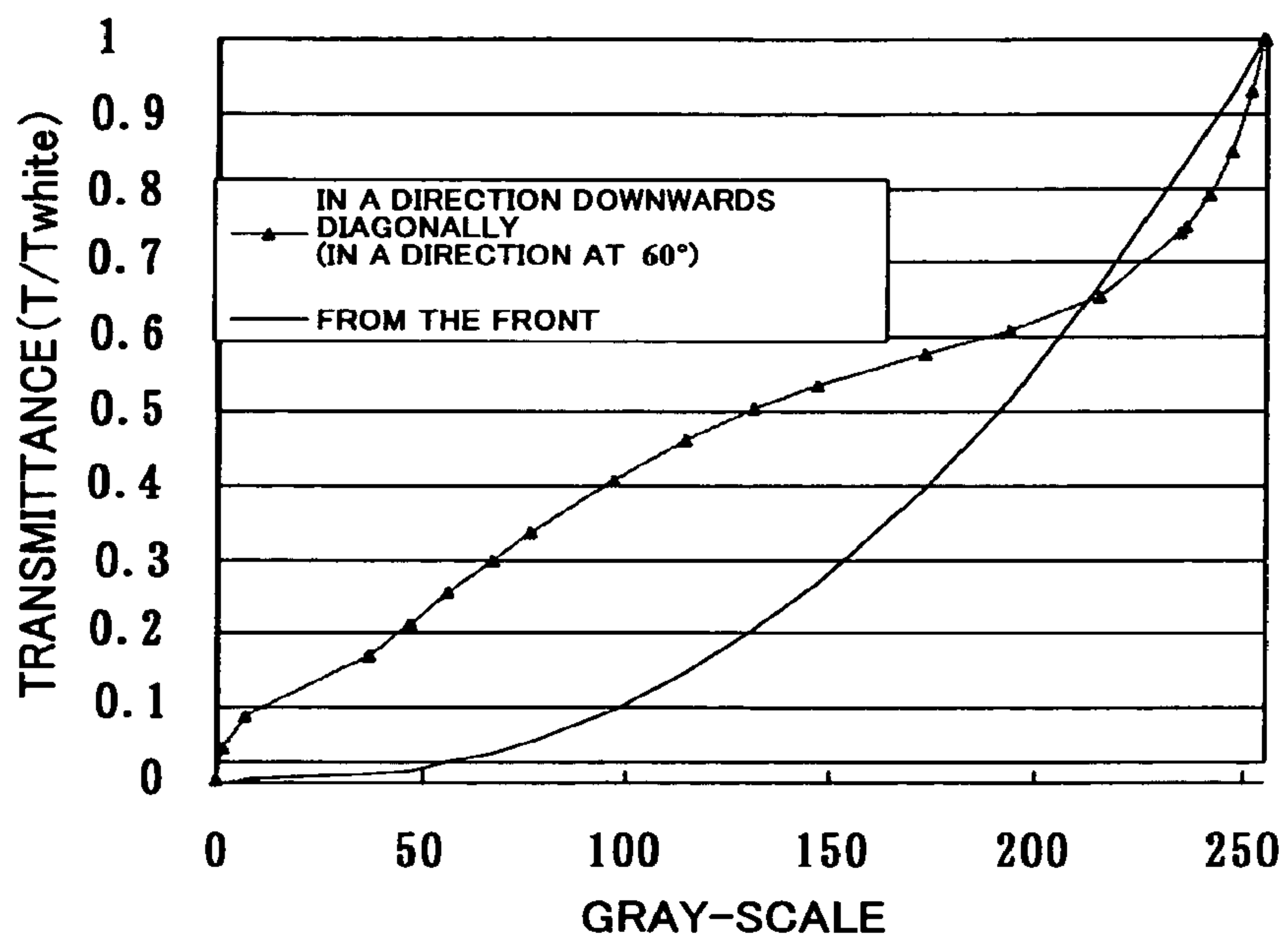
FIG. 2 (PRIOR ART)
