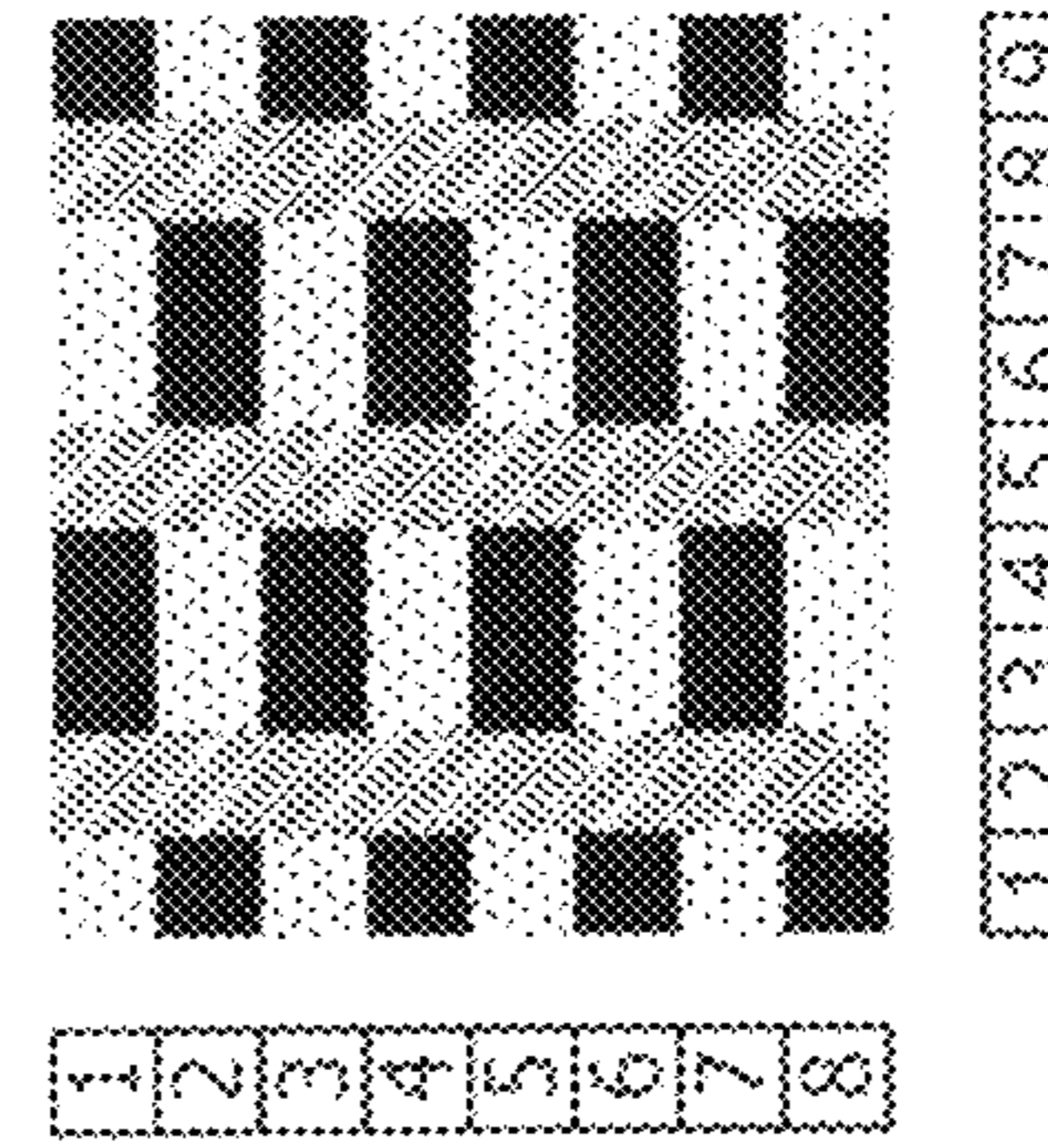
FIG. 41C FRAME INVERSION + LINE INVERSION + DOT INVERSION
